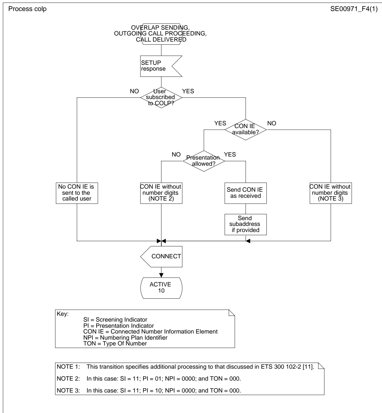
Figure 4: Originating network side dynamic description
