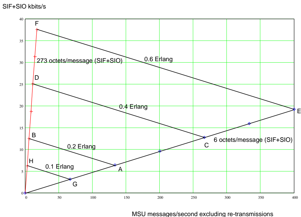
Figure ZA.1: Signalling link loading
