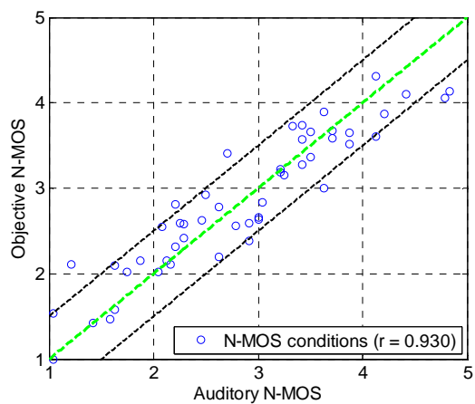
Validation Results:
