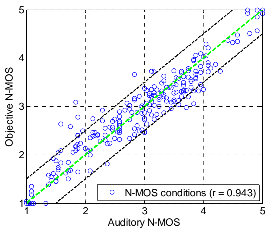
Training Results:
