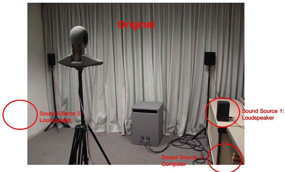
Figure 8: Simulation arrangement in a standard office room
