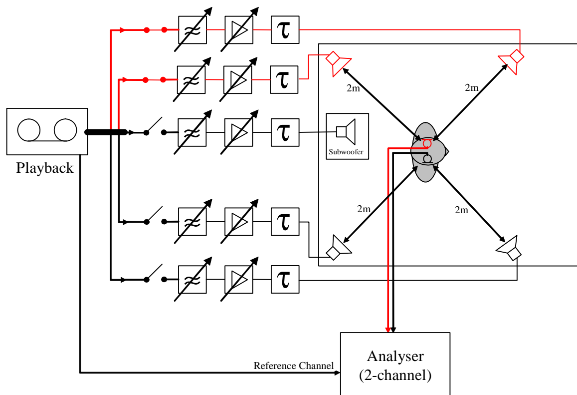
Figure 6: Block diagram of equalization setup
