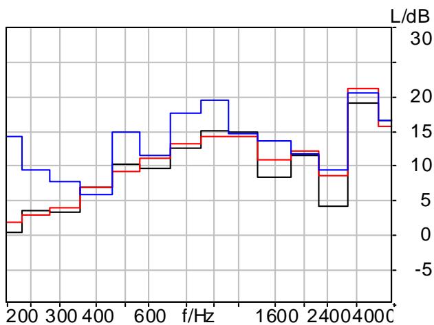
Figure B.5: Measurements of phone 5: black-fully anechoic; red - office type room; blue - semi anechoic
