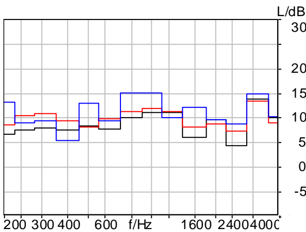
Figure B.6: Measurements of phone 6: black-fully anechoic; red - office type room; blue - semi anechoic
