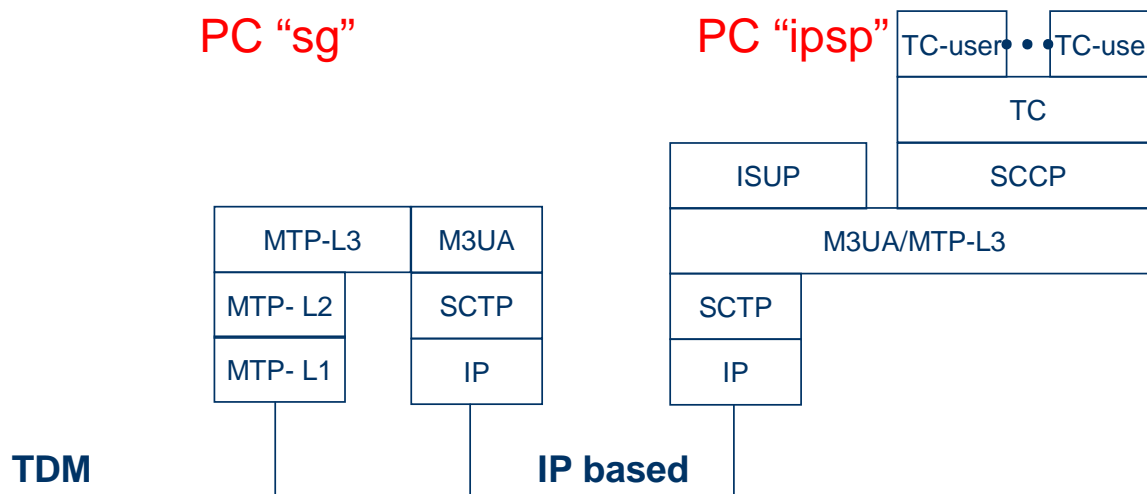
ETSI TS 102 142: SG has an SS7 Point Code different from the IPSP
