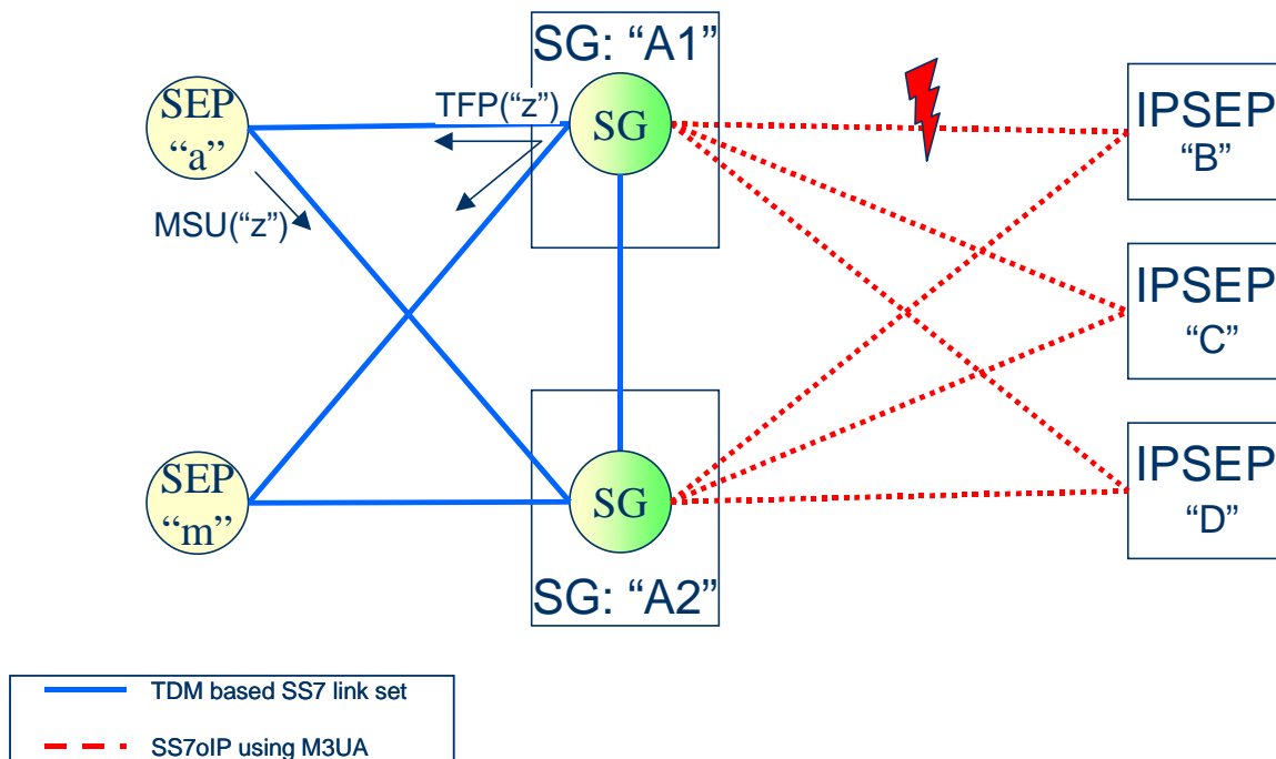
Figure 13: Migration in the SEP access area for quasi-associated signalling
