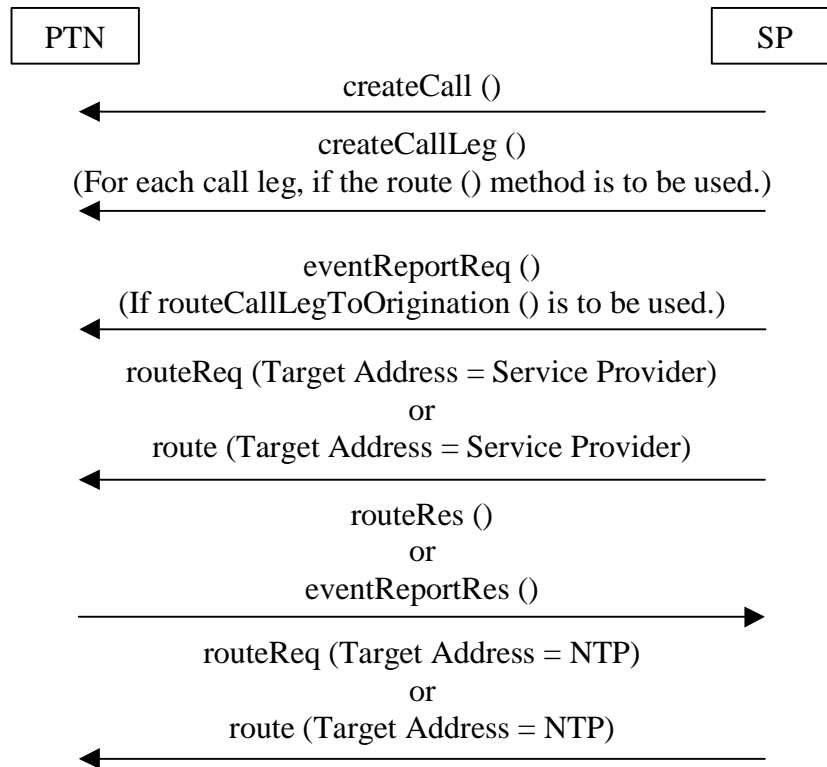
Figure 41: Interrogation of a network termination point for data delivery
