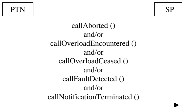
Figure 55: Event traceability
