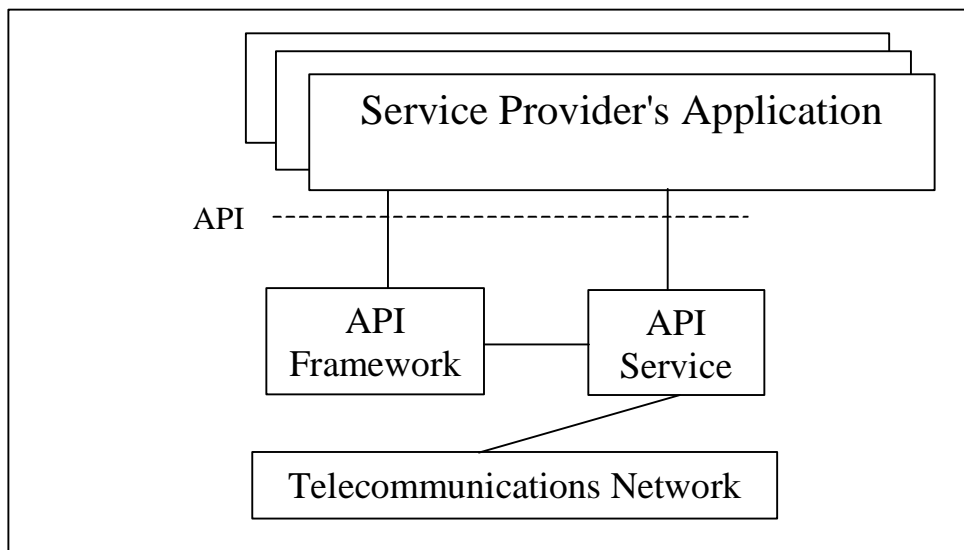
Figure 1: API Architecture
