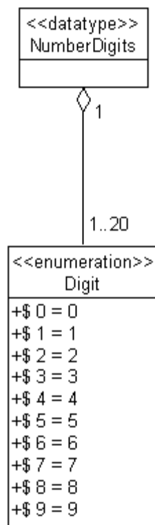
Figure 81: Type specification of QSIG digit string
