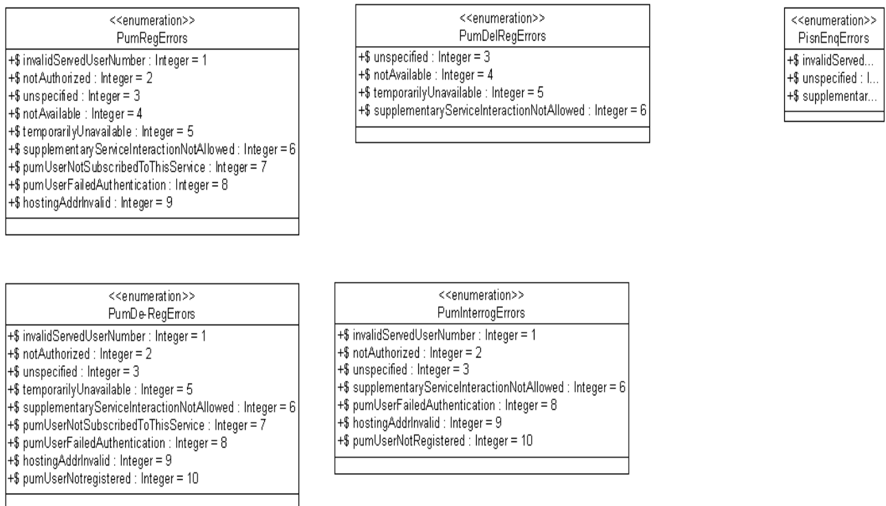
Figure 73: PUMR error codes
