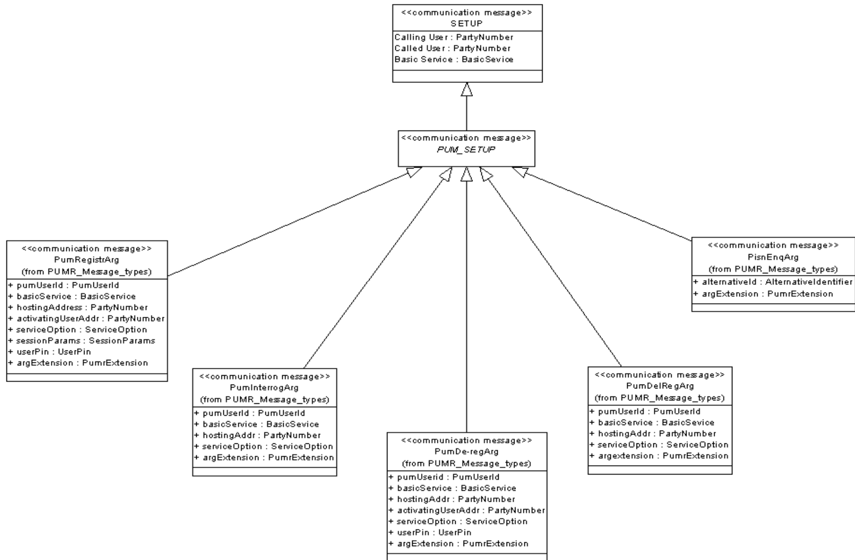
Figure 63: PUMR message contents carried in the SETUP signal
