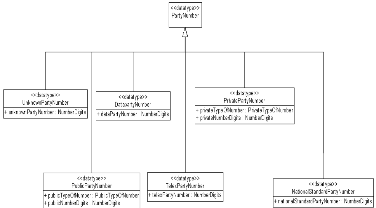
Figure 80: Type specification of QSIG party number
