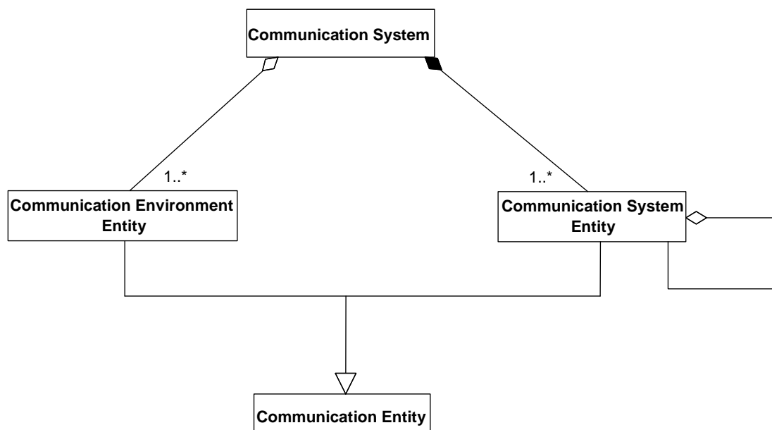
Figure 7: Generic class diagram for communication systems
