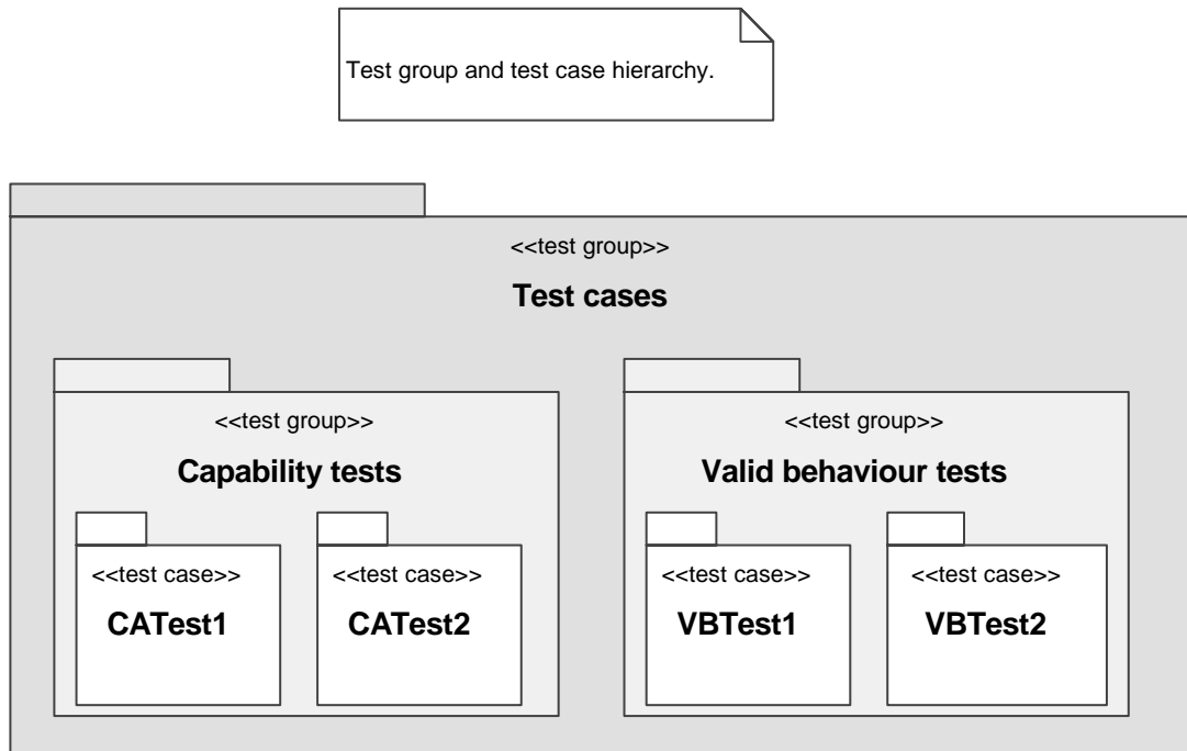
Figure 85: Test case structure
