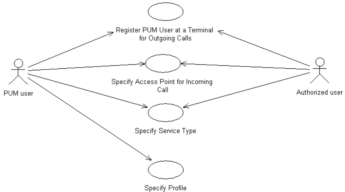
Figure 44: PUM Registration use case diagram
