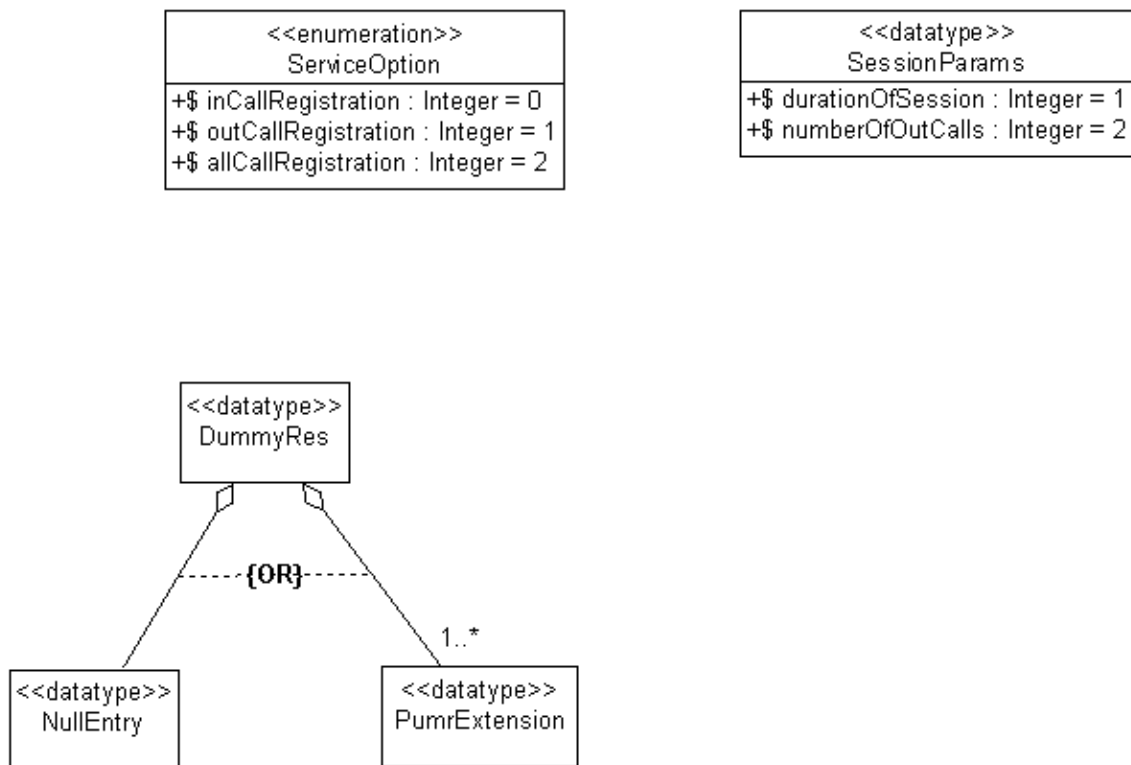
Figure 72: PUMR general data types
