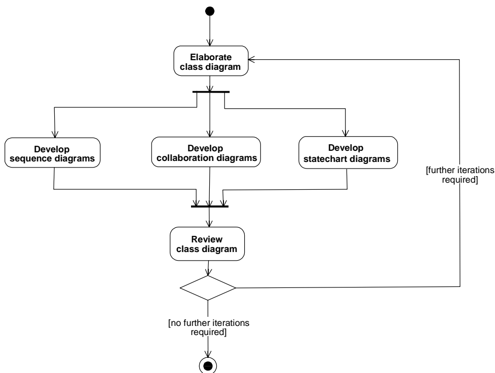
Figure 18: Specification Model development
