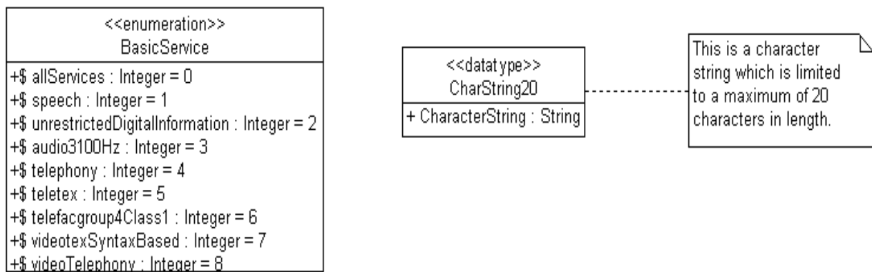
Figure 79: QSIG general data types
