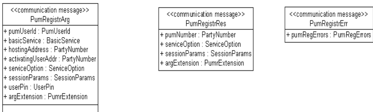
Figure 67: PUMR registration message types
