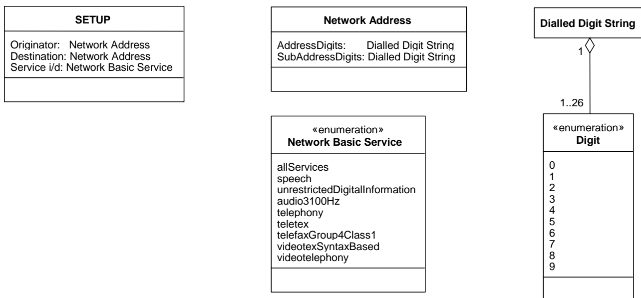
Figure 26: Example of message classes using attributes
