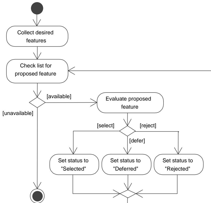
Figure 5: The feature evaluation process
