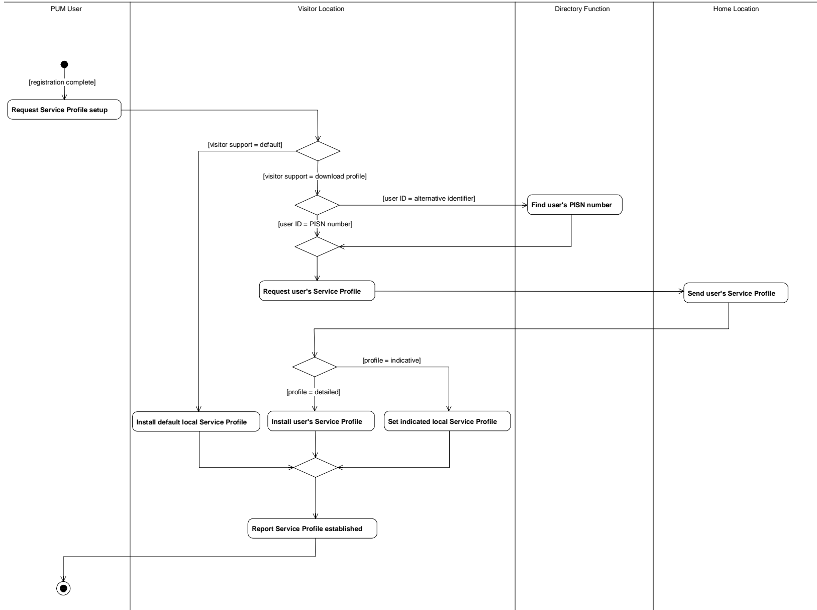
Figure 17: PUM Specify Profile activity diagram using swimlanes
