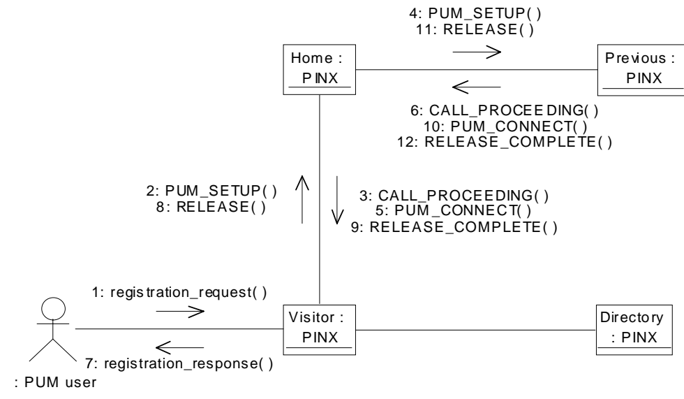
Figure 29: An example UML collaboration diagram for PUMR
