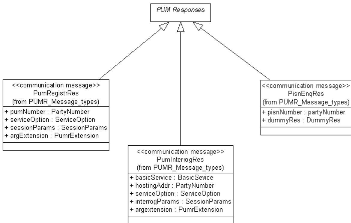
Figure 65: Contents of the PUMR response messages
