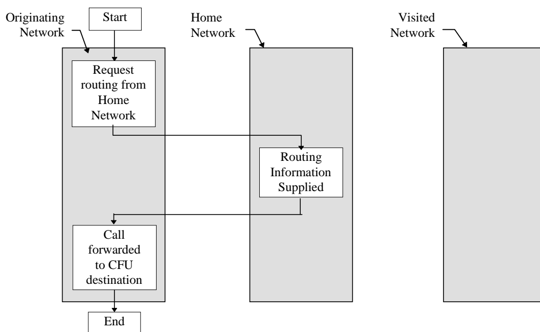
Figure 22: CTM Call Forwarding Unconditional (Non-geographic)
