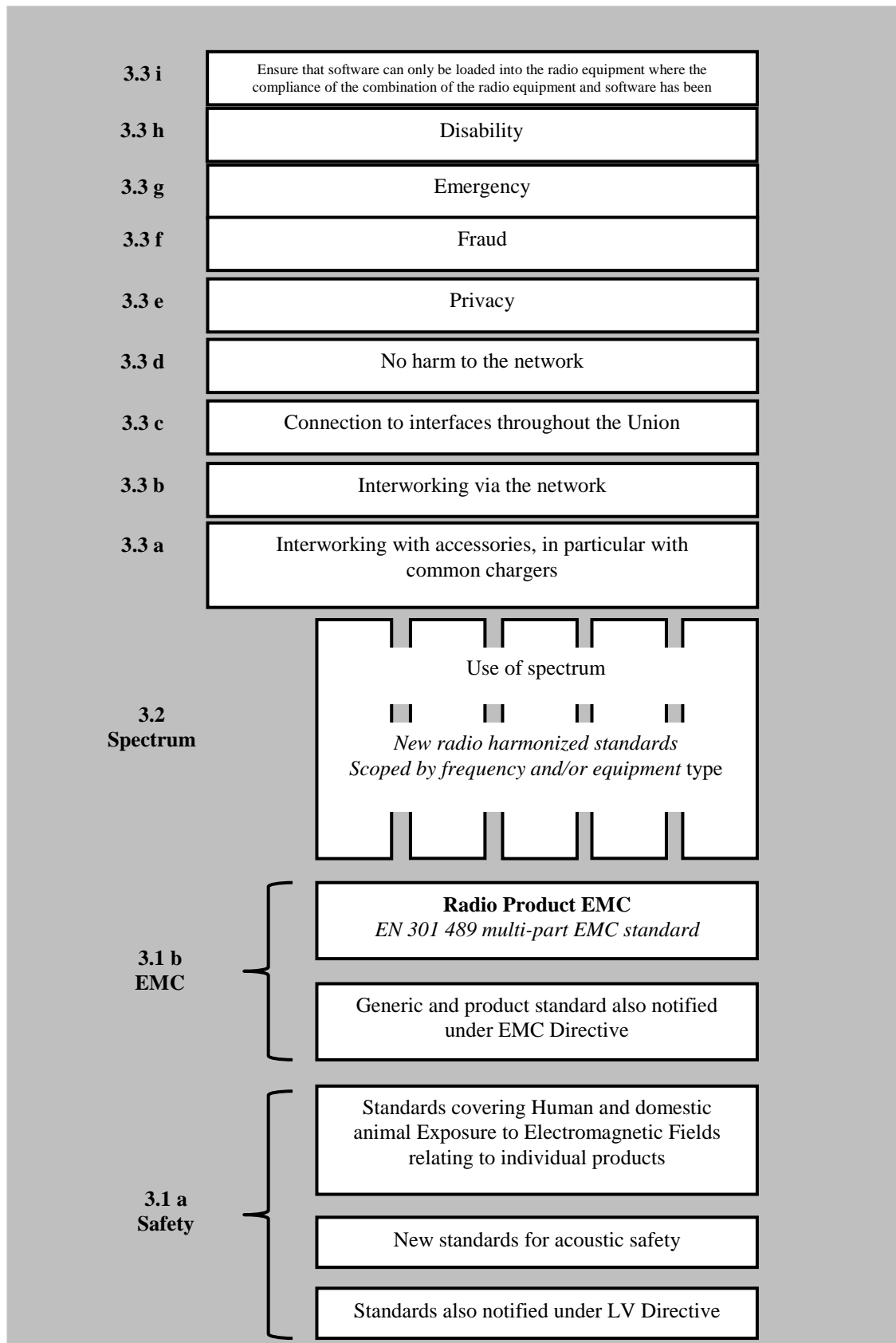
Figure D.2: Modular structure for the various standards used under the RED [i.1]
