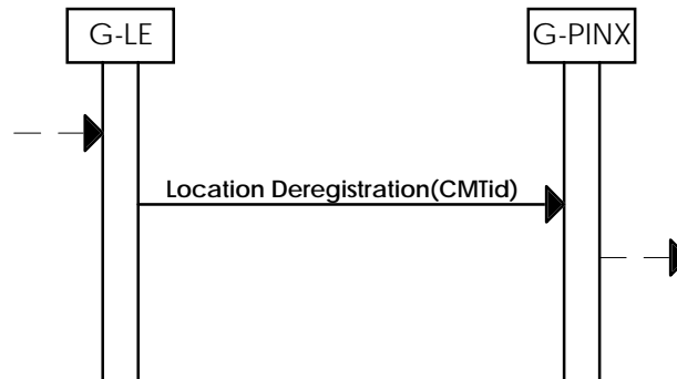
Figure 10: Location deregistration of the private network user
