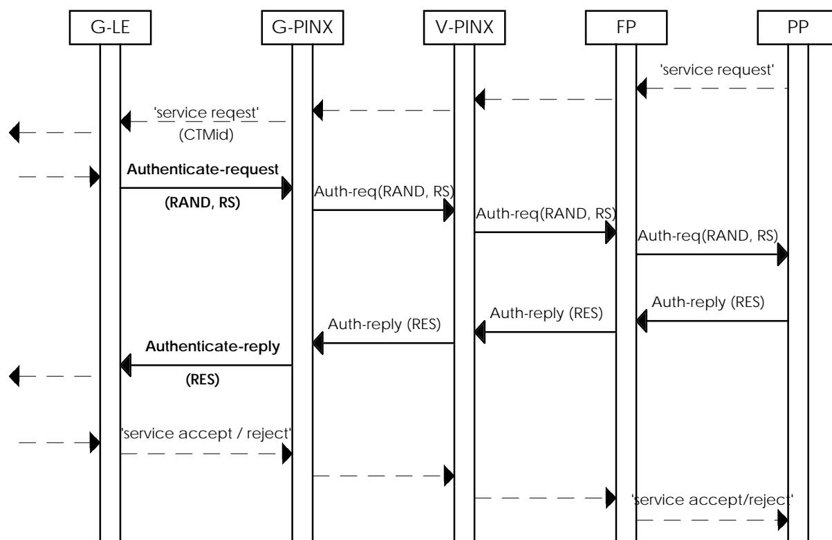
Figure 7: Authentication, public network user roaming in PISN
