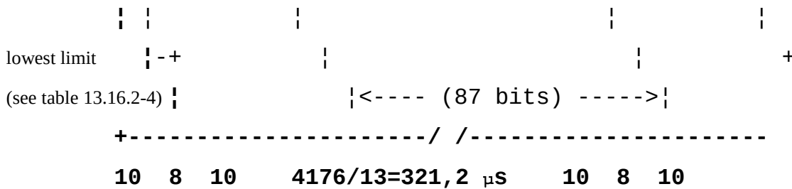
Figure 13.16.2-2: Power / time template for access burst
