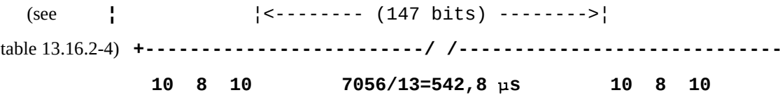
Figure 13.16.2-1: Power / time template for normal bursts
