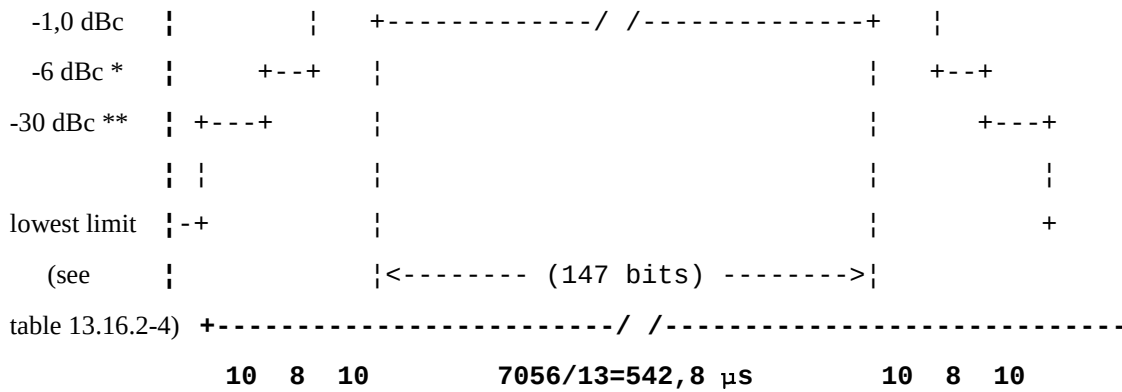
Figure 13.17.3b-1: Power / time template for normal bursts
