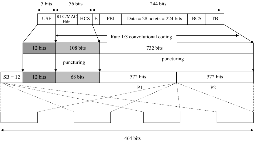
Figure 17: Coding and puncturing for MCS-2; rate 0.66 GMSK, one RLC block per radio block. In case of EC operation only P1 is defined.
