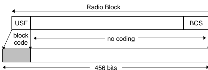
Figure 7: Radio Block structure for CS-1 to CS-3
