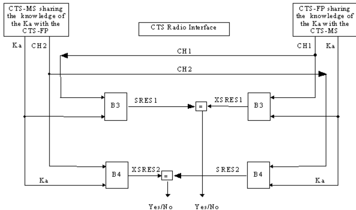
Figure E1: General mutual authentication procedure
