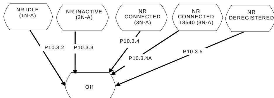
Figure 10.3.1-1: UE postamble states and procedures for NR/5GC
