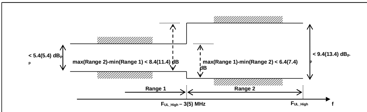
Figure 6.4G.2.4_1.5-1: The test requirements for EVM equalizer spectral flatness with the maximum allowed variation of the coefficients indicated for unshaped modulations (the ETC test requirements are within brackets)
