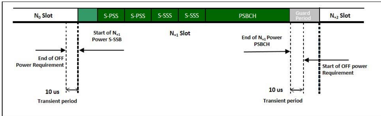
Figure 6.3E.3.0.3-1: S-SSB time mask for NR V2X UE
