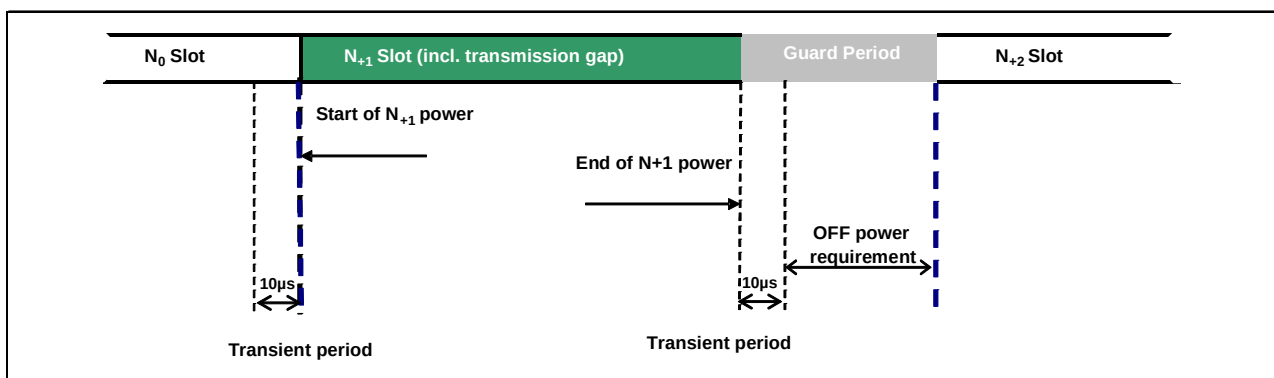
Figure 6.3E.3.0.2-1: General PSCCH/PSSCH time mask for NR V2X UE
