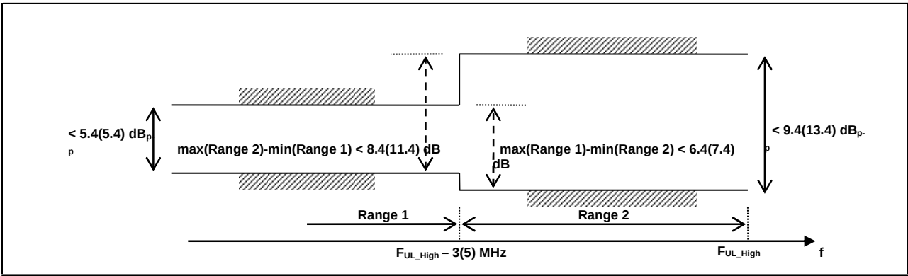
Figure 6.4E.2.5.1D.5-1: The test requirements for EVM equalizer spectral flatness with the maximum allowed variation of the coefficients indicated for unshaped modulations (the ETC test requirements are within brackets)
