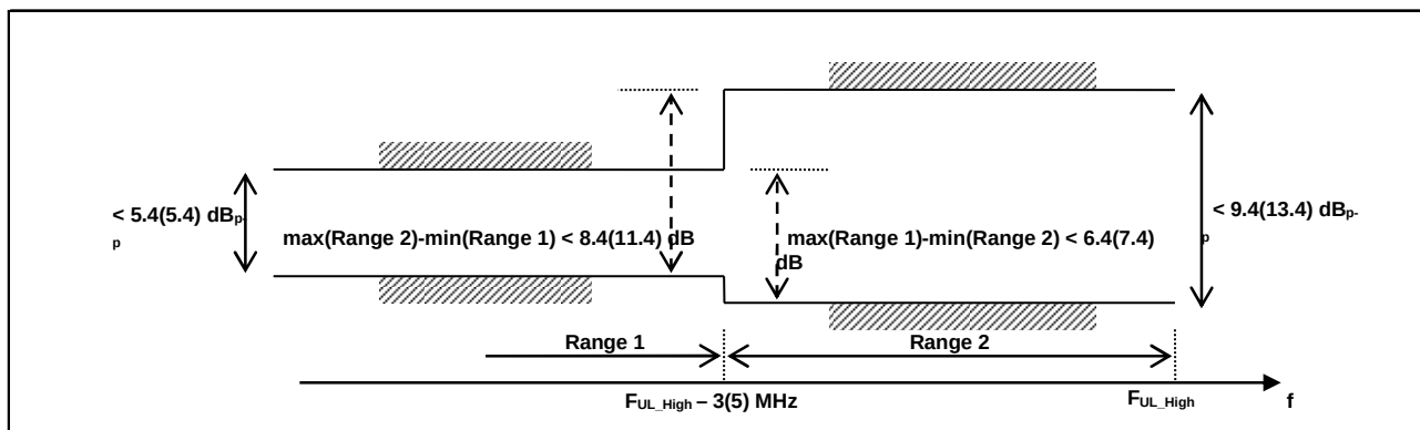
Figure 6.4J.2.4.5-1: The test requirements for EVM equalizer spectral flatness with the maximum allowed variation of the coefficients indicated for unshaped modulations (the ETC test requirements are within brackets)
