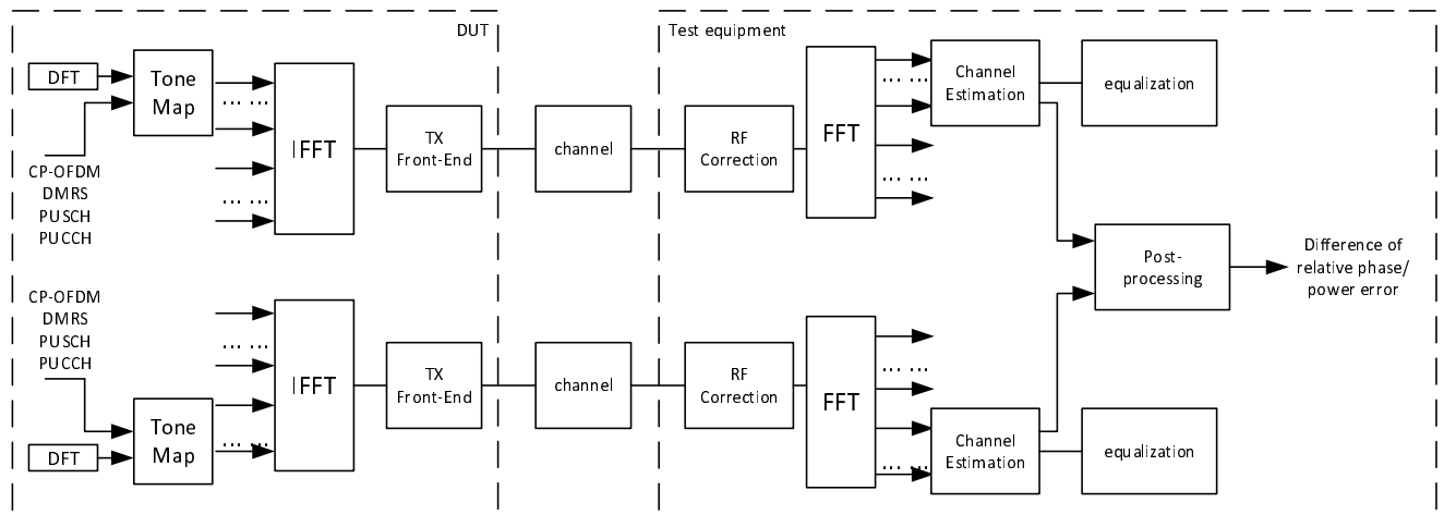
Figure J.1-1 - Measurement point for difference of relative phase/power error for UL coherent MIMO
