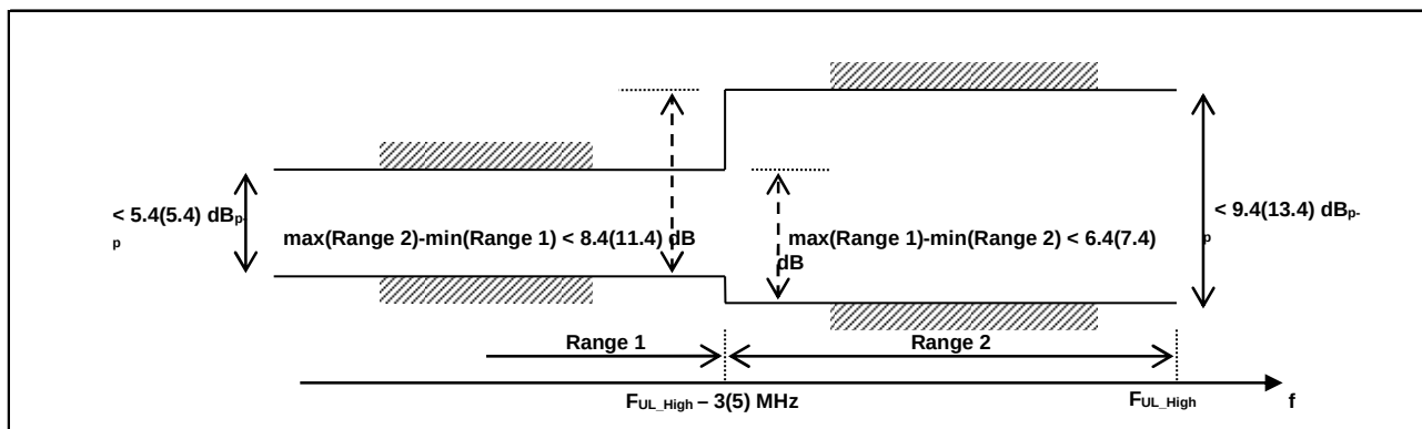
Figure 6.4E.2.5.1.5-1: The test requirements for EVM equalizer spectral flatness with the maximum allowed variation of the coefficients indicated for unshaped modulations (the ETC test requirements are within brackets)
