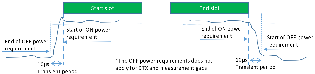
Figure 6.3J.3.1.3-1: General ON/OFF time mask for NR UL transmission in FR1
