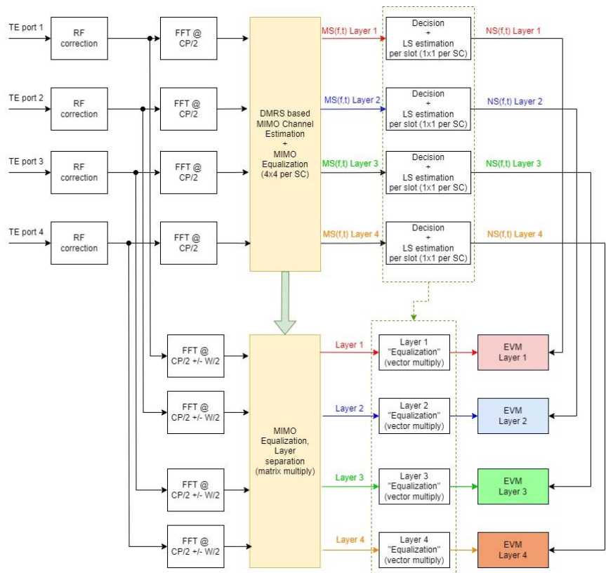
Figure E.8.1-2: EVM calculation block diagram for 4-Layer UL MIMO
