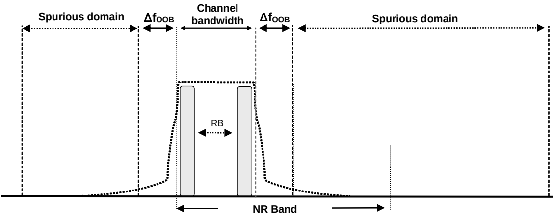
Figure 6.5J.0-1: Transmitter RF spectrum
