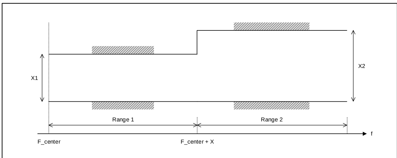
Figure 6.4J.2.5.5-1: The limits for EVM equalizer spectral flatness with the maximum allowed variation. F_{center} denotes the center frequency of the allocated block of PRBs. X , in MHz, is equal to 25 % of the bandwidth of the PRB allocation.
