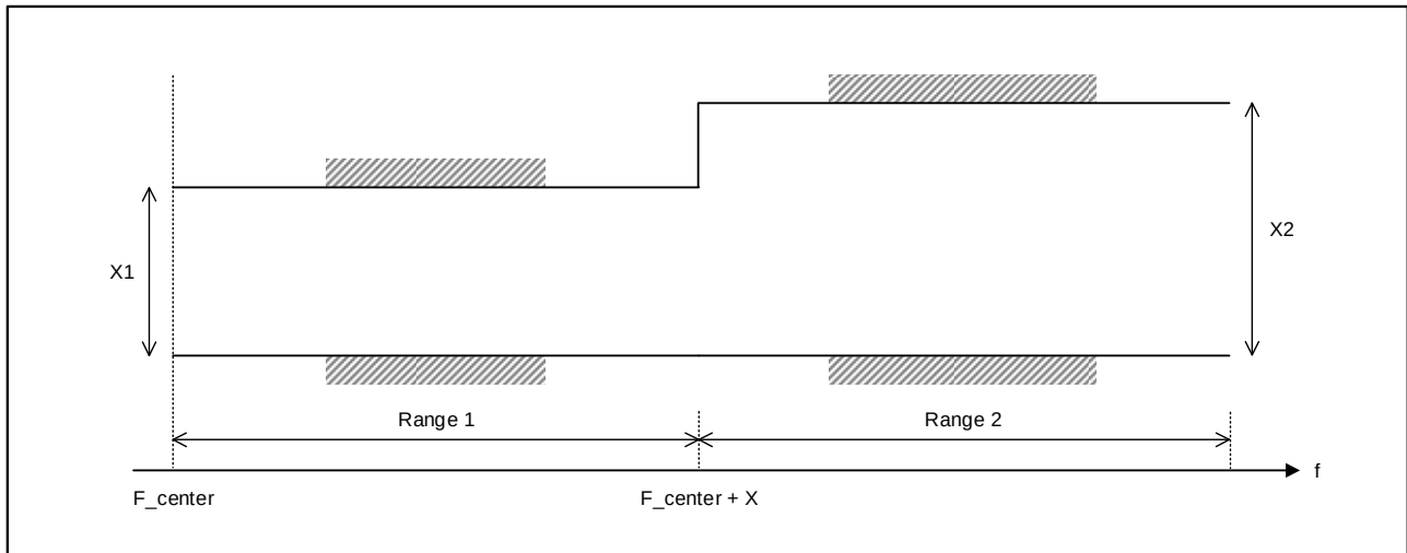
Figure 6.4.2.5.5-1: The limits for EVM equalizer spectral flatness with the maximum allowed variation. F_{center} denotes the center frequency of the allocated block of PRBs. X , in MHz, is equal to 25 % of the bandwidth of the PRB allocation.
