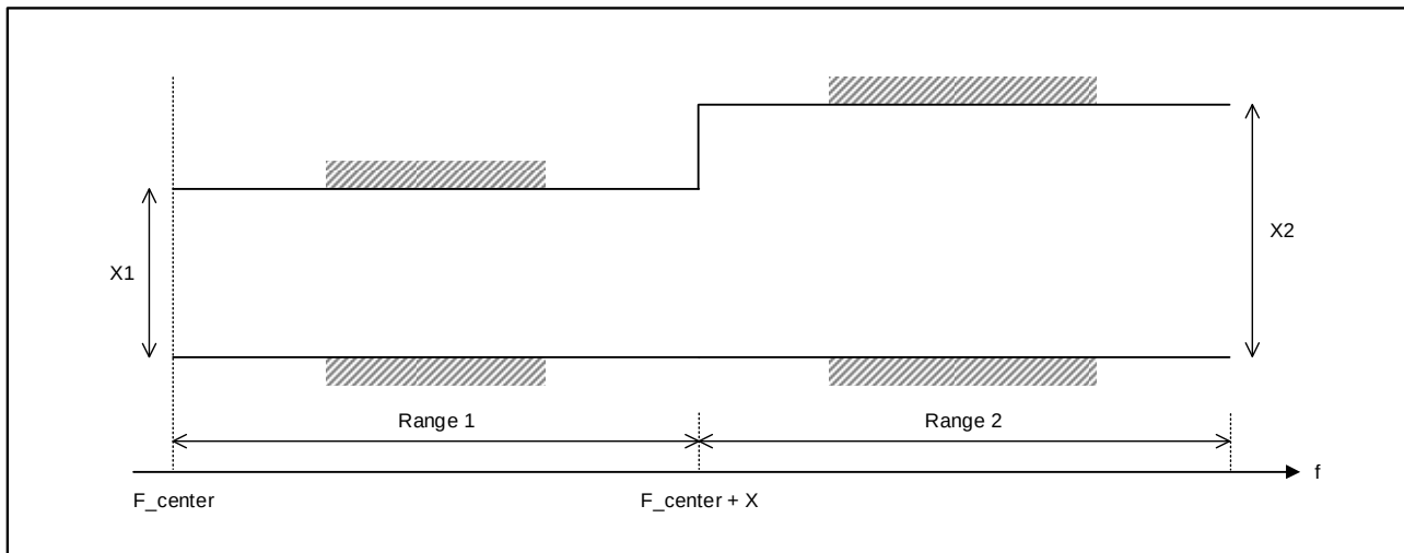
Figure 6.4J.2.5.5-1: The limits for EVM equalizer spectral flatness with the maximum allowed variation. F_{center} denotes the center frequency of the allocated block of PRBs. X, in MHz, is equal to 25 % of the bandwidth of the PRB allocation.
