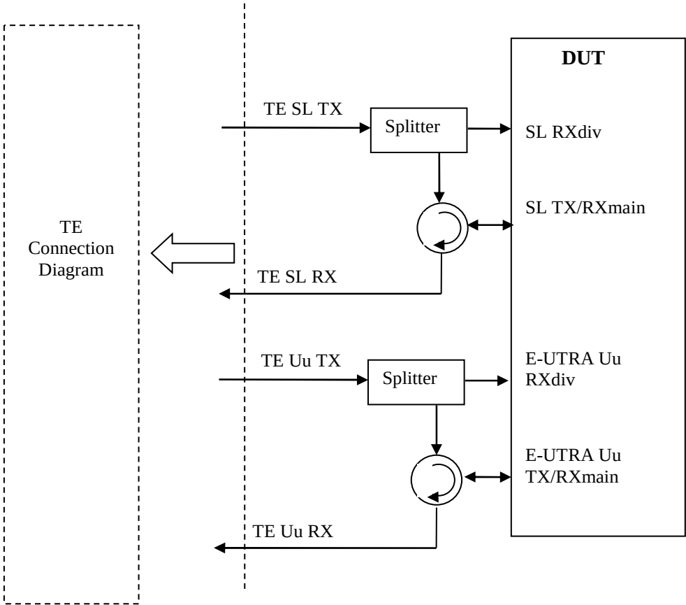
Figure A.3.2.7.4: User Equipment connection for con-current E-UTRA Uu and NR Sidelink operation
