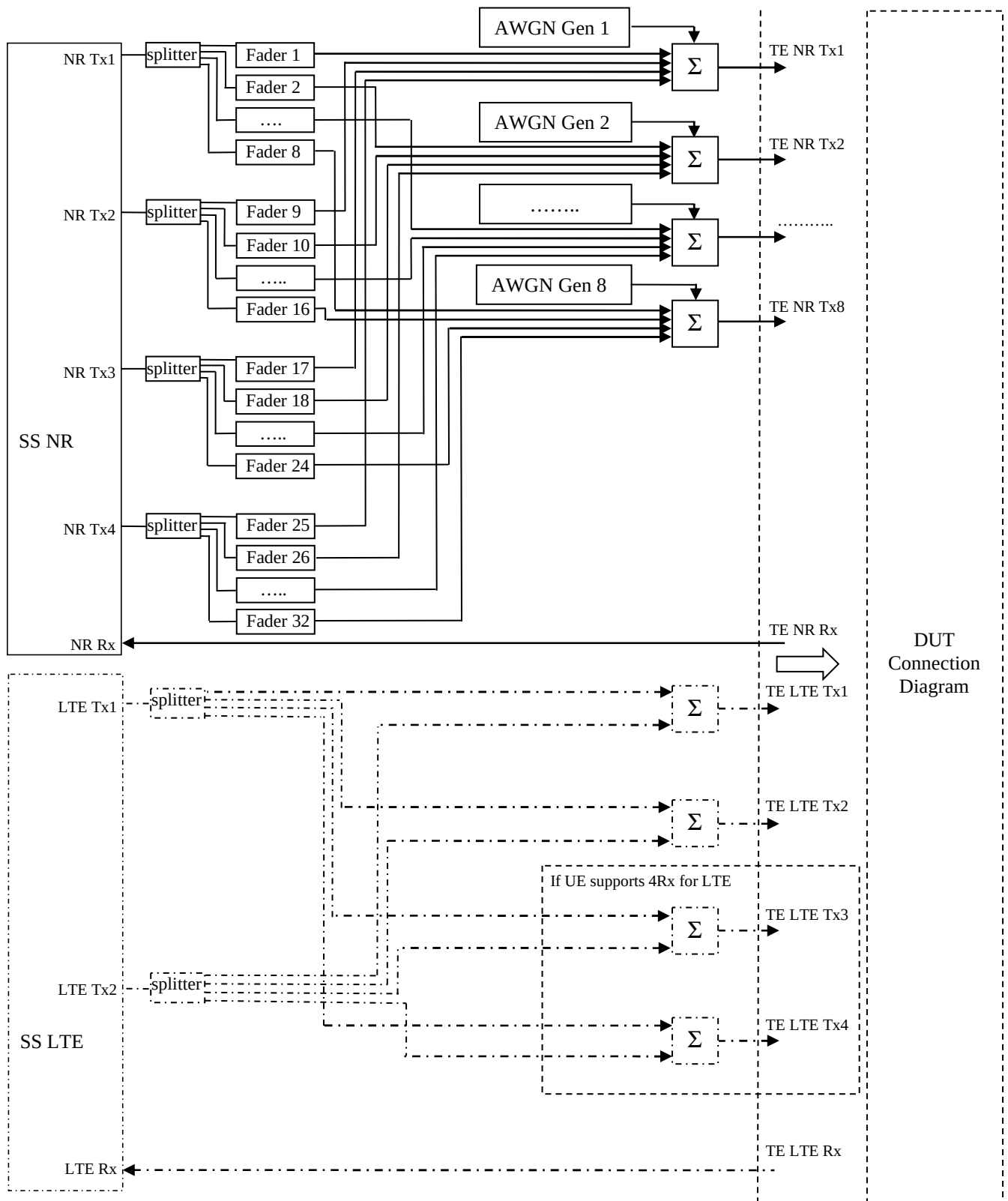
Figure A.3.1.7.13: Test Equipment connection for Demodulation Performance and CSI reporting tests with antenna configuration 4x8
