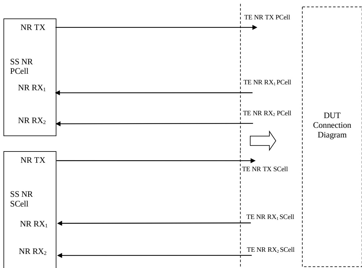
Figure A.3.1.1.6: Test Equipment connection for NR intra-band UL contiguous CA with UL MIMO or Tx diversity
