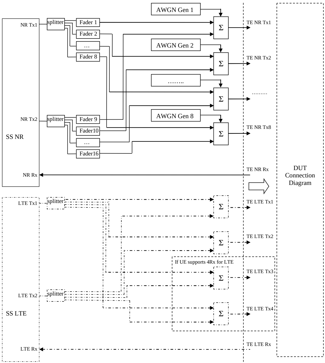
Figure A.3.1.7.12: Test Equipment connection for Demodulation Performance and CSI reporting tests with antenna configuration 2x8
