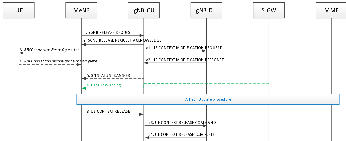
Figure 8.4.2.1-1 SgNB release procedure in EN-DC (MN initiated)
