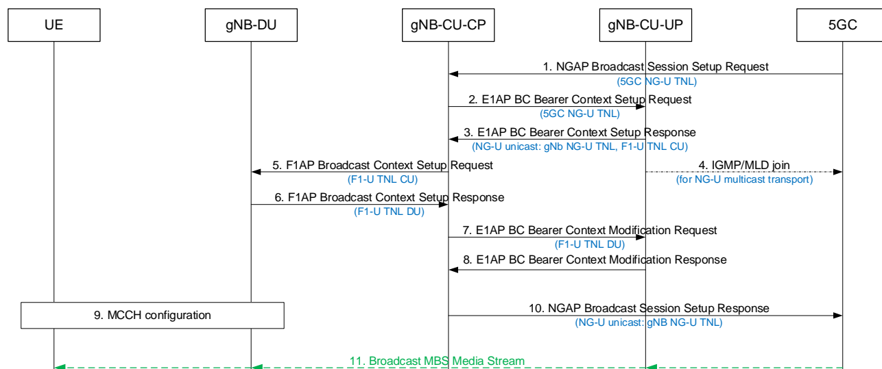
Figure 8.15.1.1-1: Broadcast MBS Session Setup
