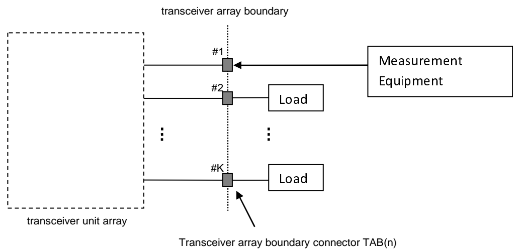
Figure 4.5.1.2-1: Receiver test ports
