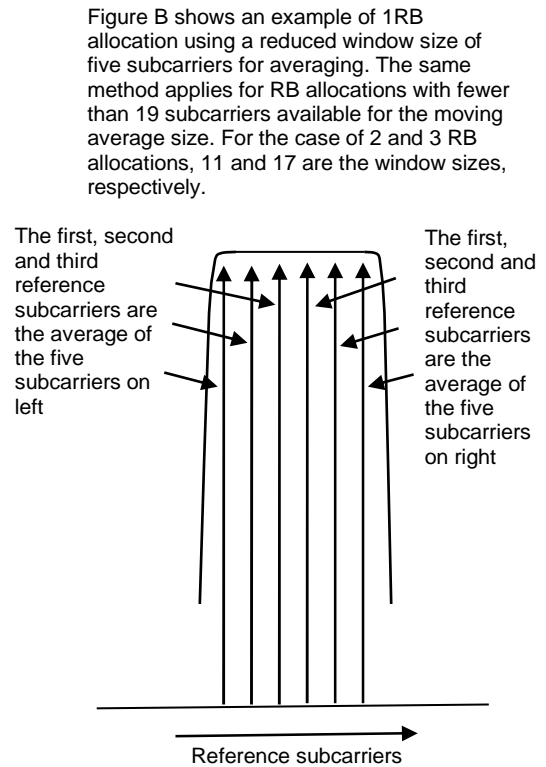
B. Moving averaging for the case when the number of available reference subcarriers within a set of contiguously allocated RBs is smaller than the moving average window size
