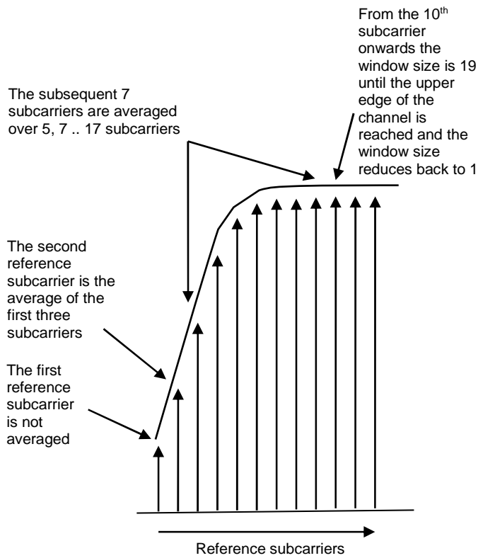
A. Moving averaging at channel edge
