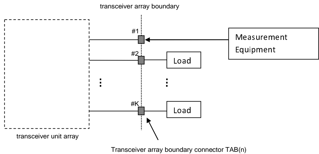
Figure 4.5.2.2-1: Receiver test ports
