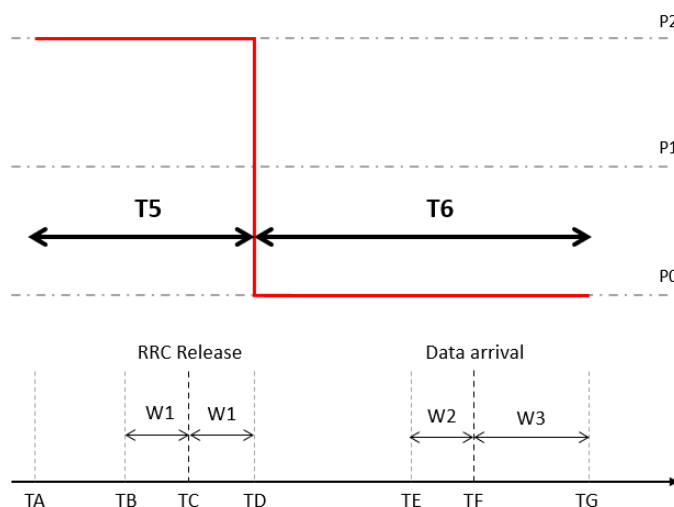
Figure A.6.2.1.1-2: RSRP variation model for CG-SDT Sub-test#2
