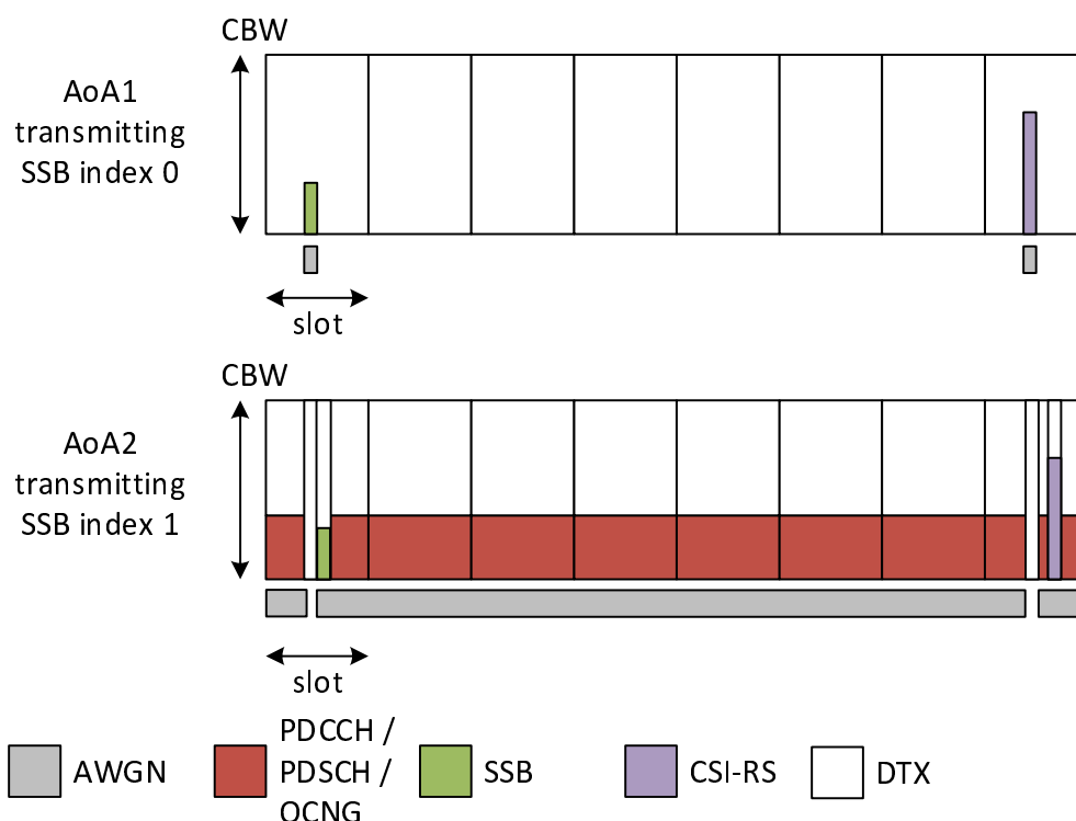
Figure A.7.5.8.1.1.1-2: Time multiplexed downlink transmissions during T2
