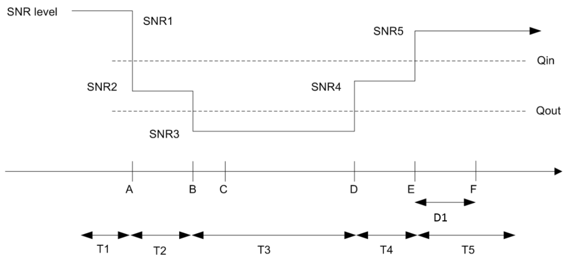
Figure A.11.4.1.3.1-1: SNR variation for in-sync testing.
