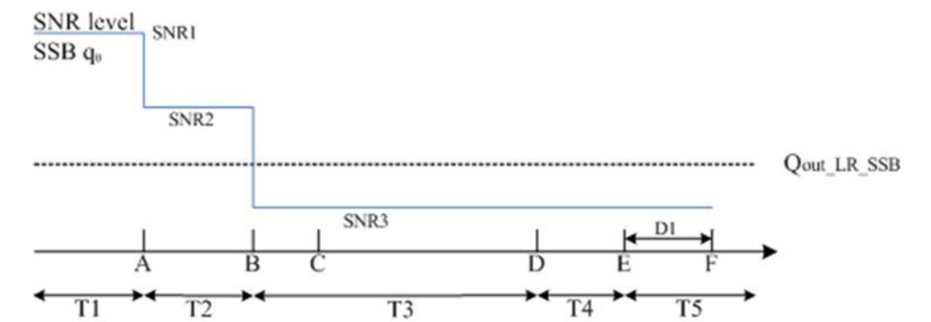
Figure A.4.5.5.2.1-1: SNR variation for SSB-based beam failure detection and link recovery testing in DRX mode
