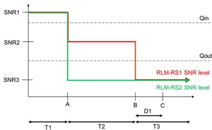
Figure A.17.5.1.7.1-1: SNR variation for CSI-RS out-of-sync testing
