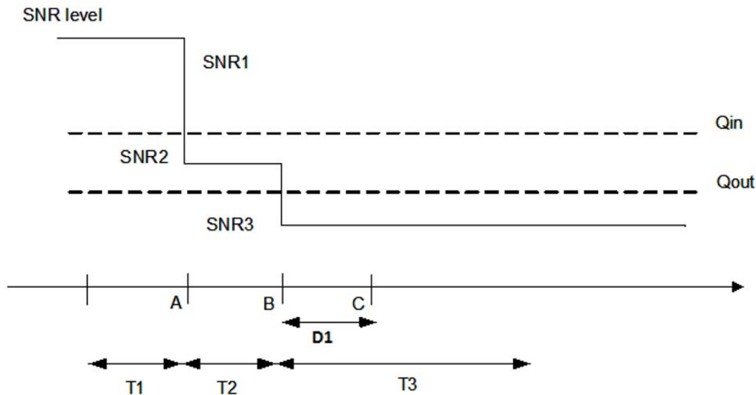
Figure A.16.5.1.1.1-1: SNR variation for out-of-sync testing
