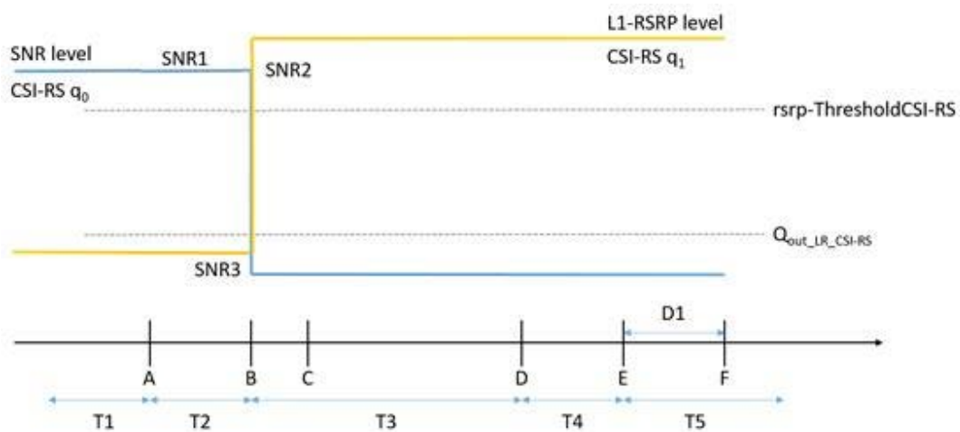
Figure A.7.5.5.8.1-1: SNR and L1-RSRP variation for CSI-RS-based beam failure detection and link recovery testing in DRX mode
