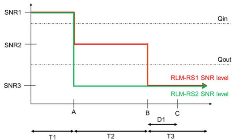
Figure A.17.5.1.5.1-1: SNR variation for CSI-RS out-of-sync testing
