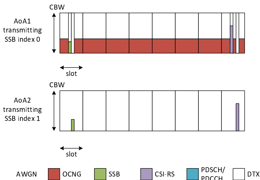
Figure A.7.6.16.1.1-1: Time multiplexed downlink transmissions (Config 1 example)
