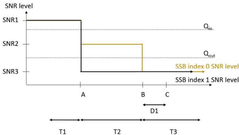
Figure A.17.5.1.3.1-1: SNR variation for out-of-sync testing
