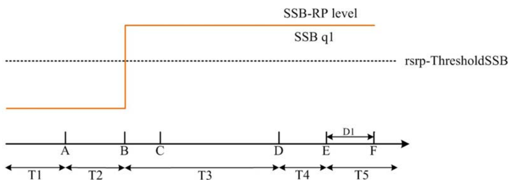
Figure A.17.5.2.5.1-2: SSB_RP level variation for SSB-based beam failure detection and link recovery testing in non-DRX mode
