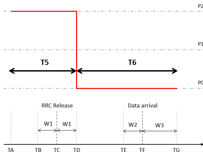
Figure A.16.2.1.2.1-2: RSRP variation model for CG-SDT Sub-test#2
