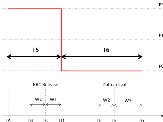
Figure A.16.2.1.1.1-2: RSRP variation model for CG-SDT Sub-test#2
