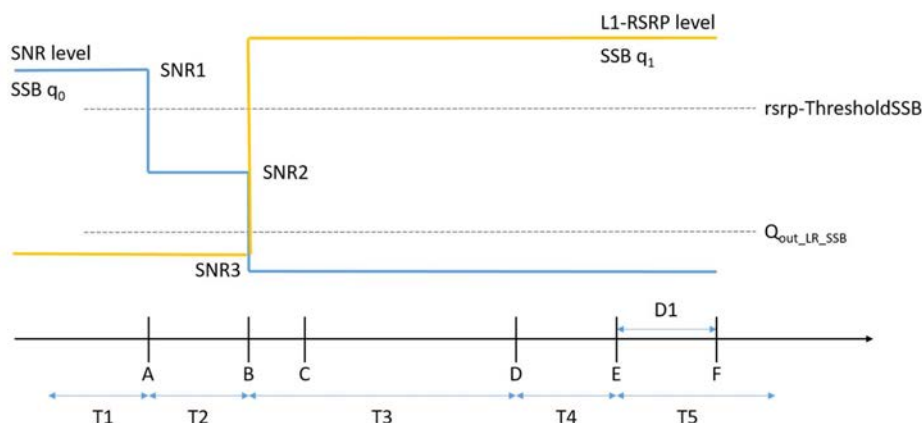
Figure A.16.5.2.2.1-1: SNR and L1-RSRP variation SSB for SSB-based beam failure detection and link recovery testing in non-DRX mode
