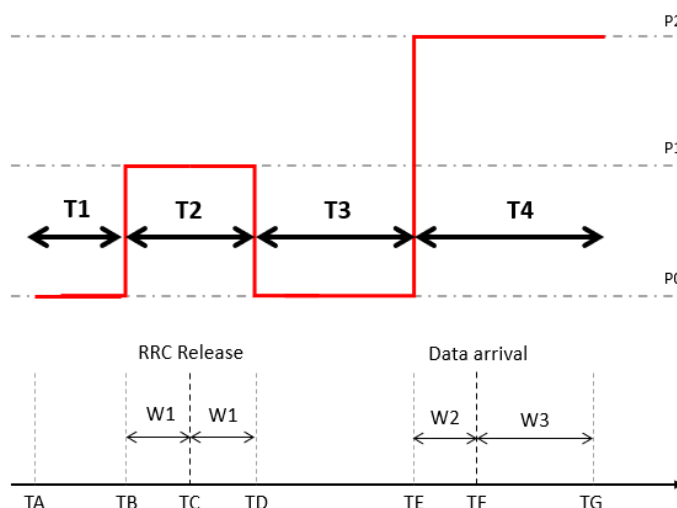
Figure A.16.2.1.1.1-1: RSRP variation model for CG-SDT Sub-test#1
