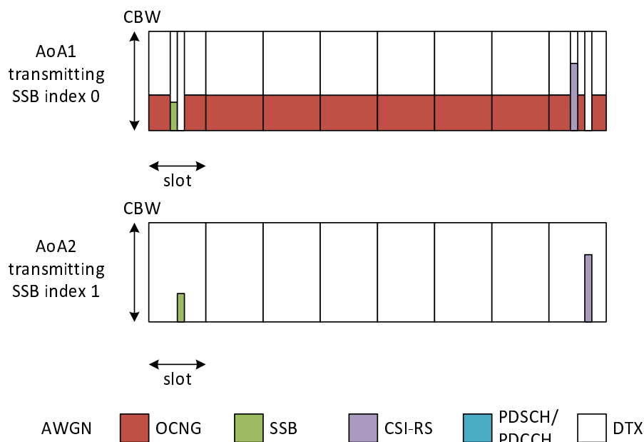
Figure A.7.6.1.11.1-1: Time multiplexed downlink transmissions (Config 1 example)
