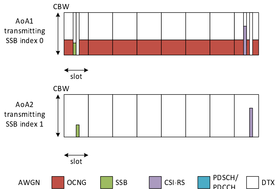
Figure A.7.6.1.6.1-1: Time multiplexed downlink transmissions (Config 1 example)
