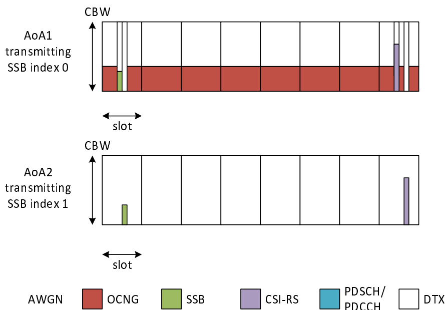
Figure A.17.6.1.3.1-1: Time multiplexed downlink transmissions (Config 1 example)
