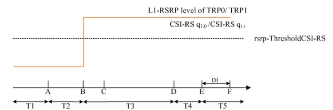
Figure A.6.5.7.1-2: L1-RSRP level variation for CSI-RS-based beam failure detection and link recovery testing in DRX mode
