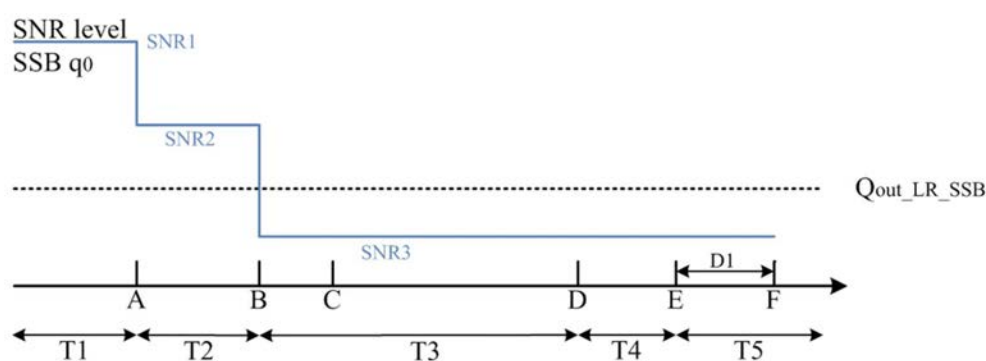
Figure A.7.5.1.1-1: SNR variation for SSB-based beam failure detection and link recovery testing in non-DRX mode
