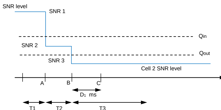
Figure A.16.5.1.14.1-1: SNR variation for CSI-RS out-of-sync testing
