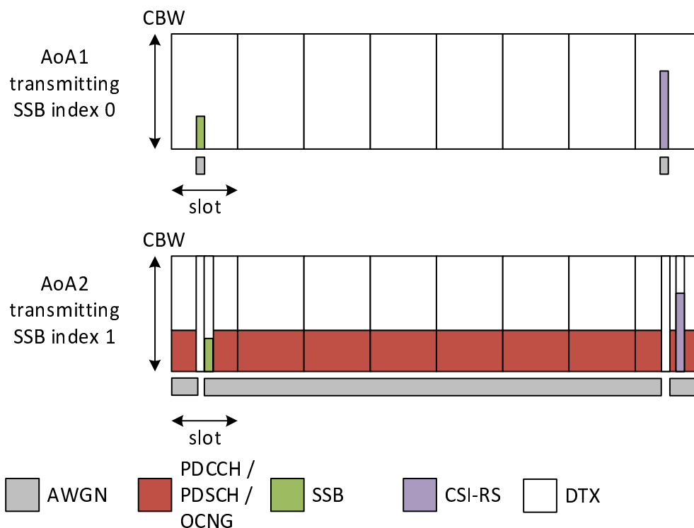
Figure A.17.5.4.1.1-2: Time multiplexed downlink transmissions during T2
