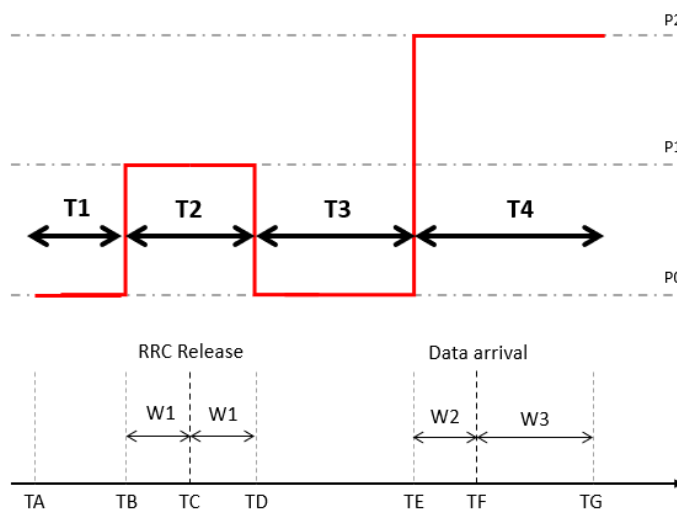
Figure A.16.2.1.2.1-1: RSRP variation model for CG-SDT Sub-test#1
