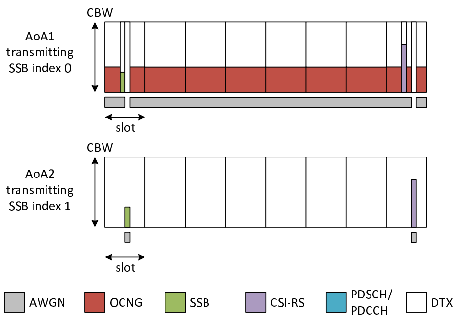
Figure A.17.5.1.2.1-2: Time multiplexed downlink transmissions
