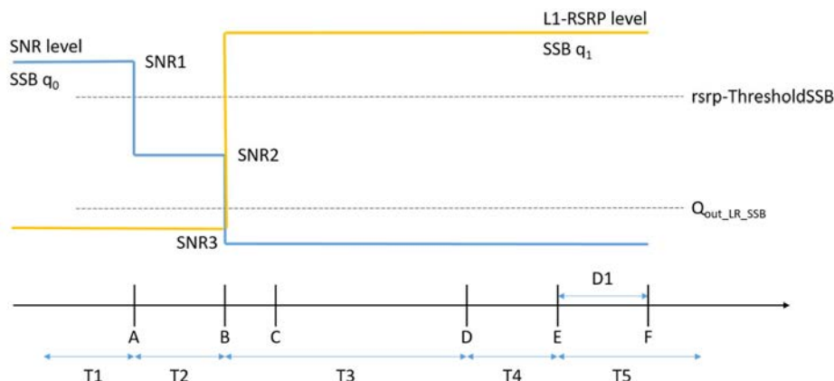
Figure A.16.5.2.1.1-1: SNR and L1-RSRP variation SSB for SSB-based beam failure detection and link recovery testing in non-DRX mode
