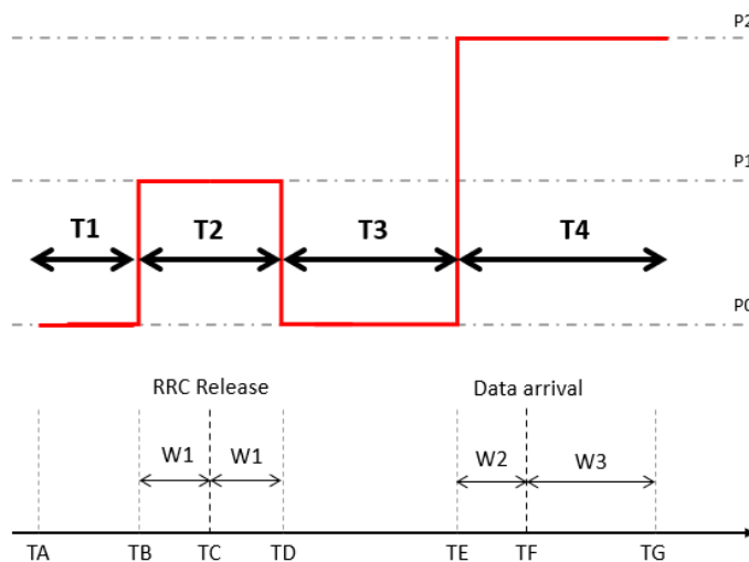
Figure A.17.2.1.1.1-1: RSRP variation model for CG-SDT Sub-test#1
