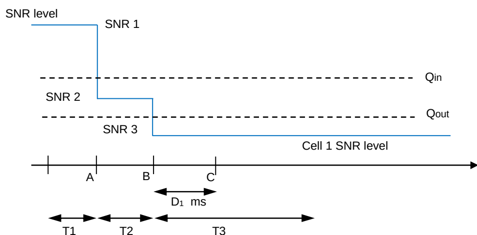
Figure A.14.4.1.5.1-1: SNR variation for CSI-RS out-of-sync testing
