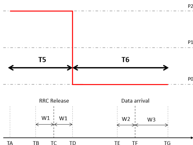
Figure A.7.2.1.1.1-2: RSRP variation for TA validation for CG-SDT Sub-test#2
