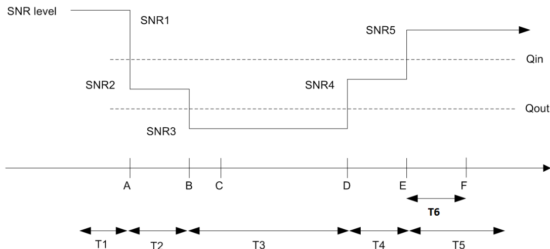
Figure A.16.5.1.12.1-1: SNR variation for CSI-RS in-sync testing
