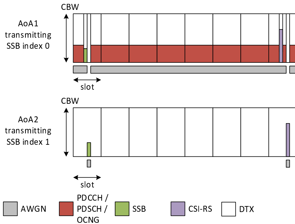
Figure A.17.5.4.2.1.1-1-1: Time multiplexed downlink transmissions during T1
