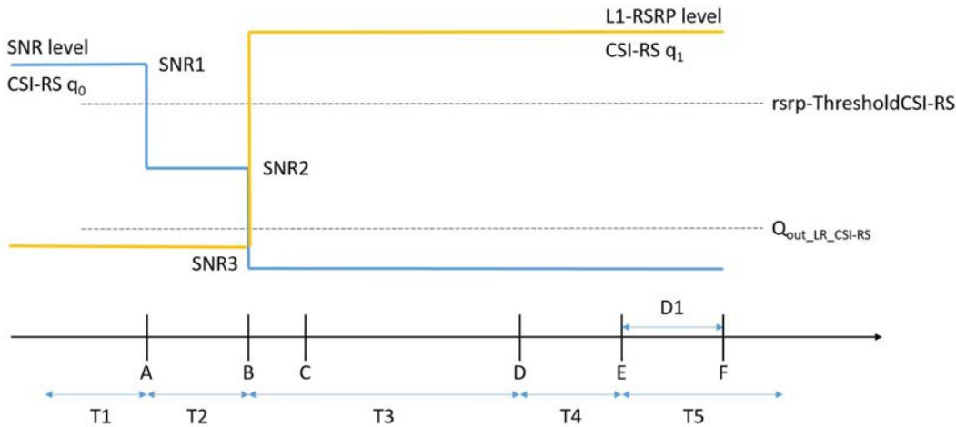
Figure A.7.5.5.12.1-1: SNR and L1-RSRP variation for CSI-RS-based beam failure detection and link recovery testing in DRX mode
