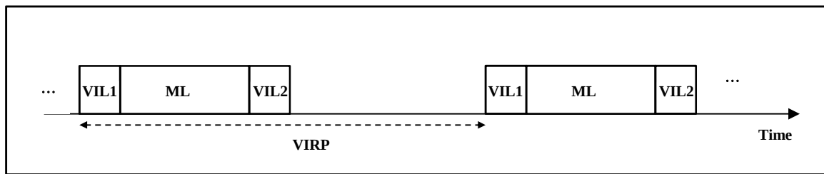
Figure 9.1.9.3-1: Illustration of NCSG parameters: VIL1, ML, VIL2 and VIRP
