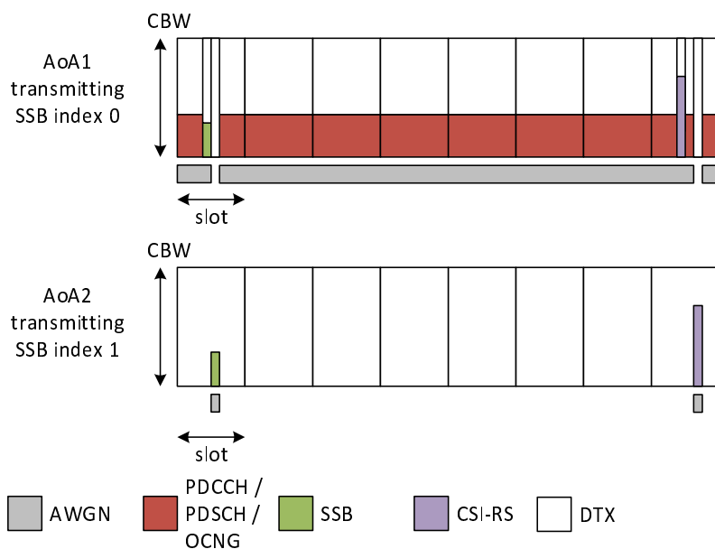
Figure A.7.5.8.3.1.1-1: Time multiplexed downlink transmissions during T1
