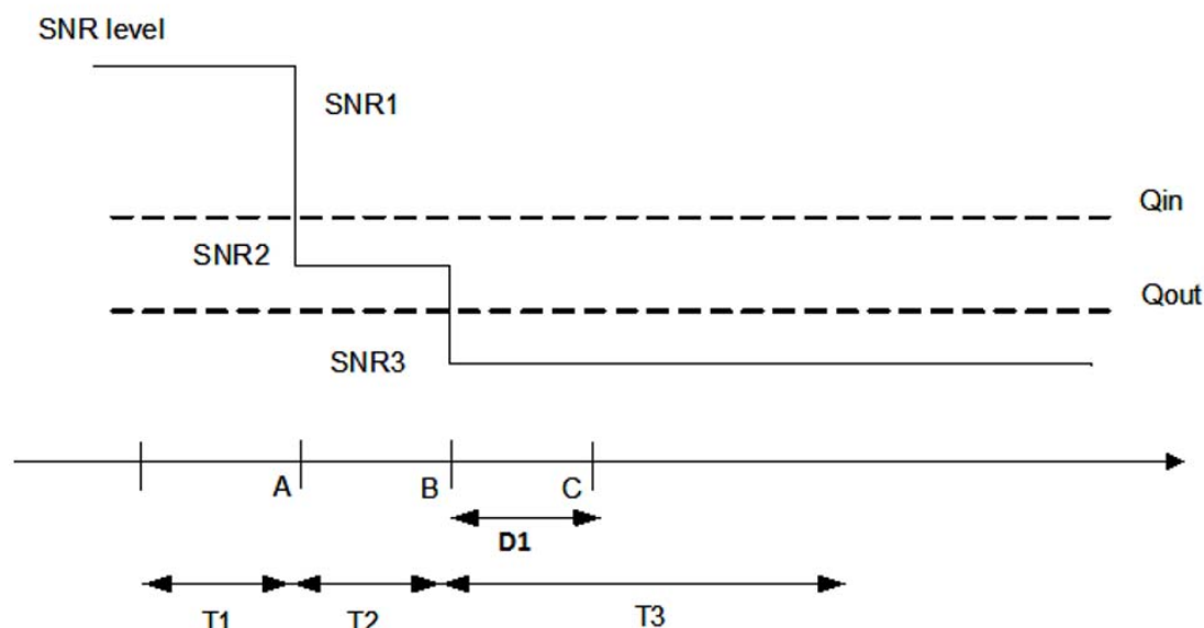
Figure A.16.5.1.6.1-1: SNR variation for out-of-sync testing
