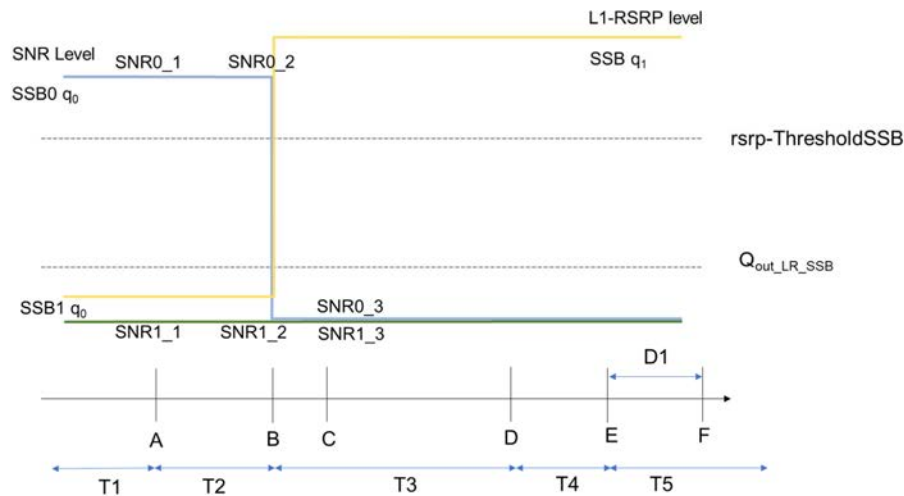
Figure A.5.5.9.1-1: SNR and L1-RSRP variation for SSB-based beam failure detection and link recovery testing in DRX mode for UE fulfilling relaxed measurement criterion
