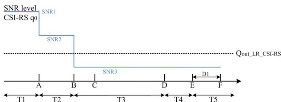
Figure A.5.5.7.1-1: SNR variation for CSI-RS-based beam failure detection and link recovery testing for SCell in DRX mode
