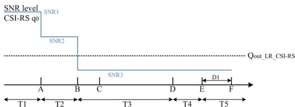
Figure A.7.5.5.6.1-1: SNR and L1-RSRP variation for beam failure detection and link recovery testing for SCell in non-DRX mode
