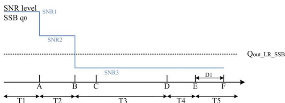
Figure A.17.5.2.1.1-1: SNR variation for SSB-based beam failure detection and link recovery testing in non-DRX mode
