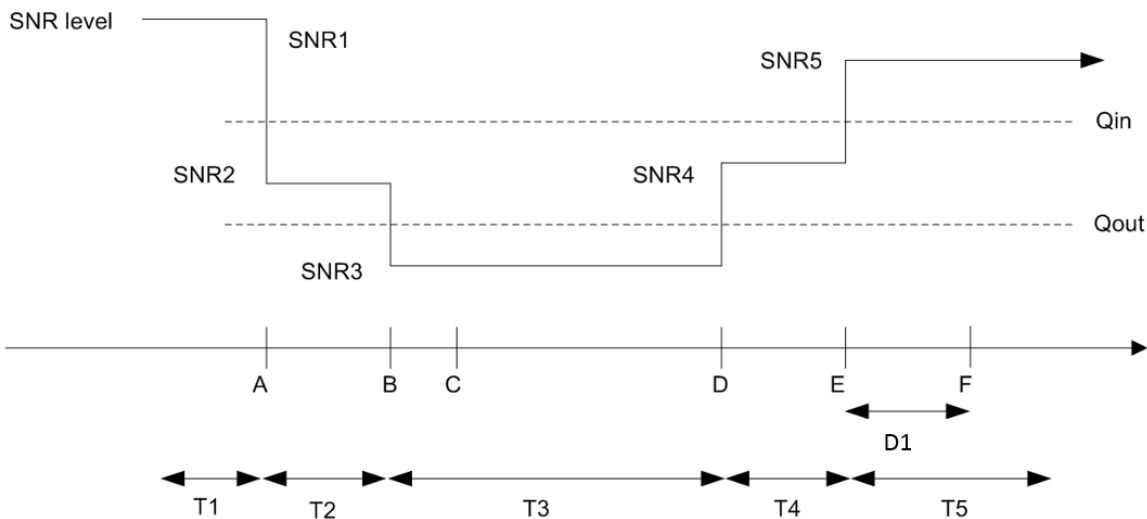
Figure A.14.4.1.2.1-1: SNR variation for in-sync testing
