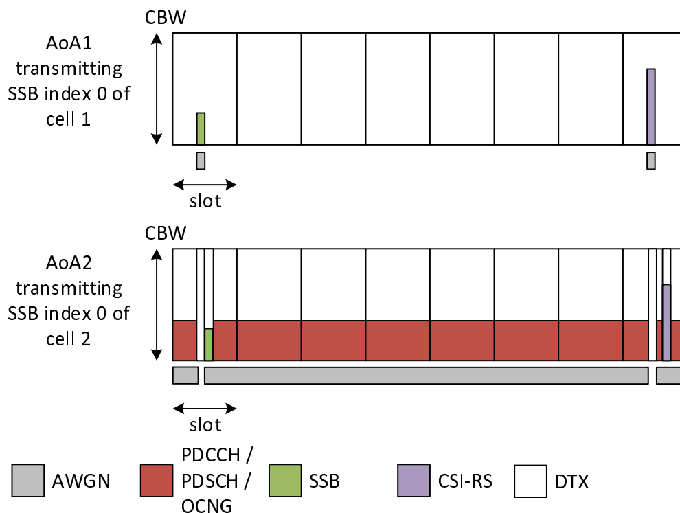
Figure A.7.5.13.3.1.2-2: Time multiplexed downlink transmissions during T2
