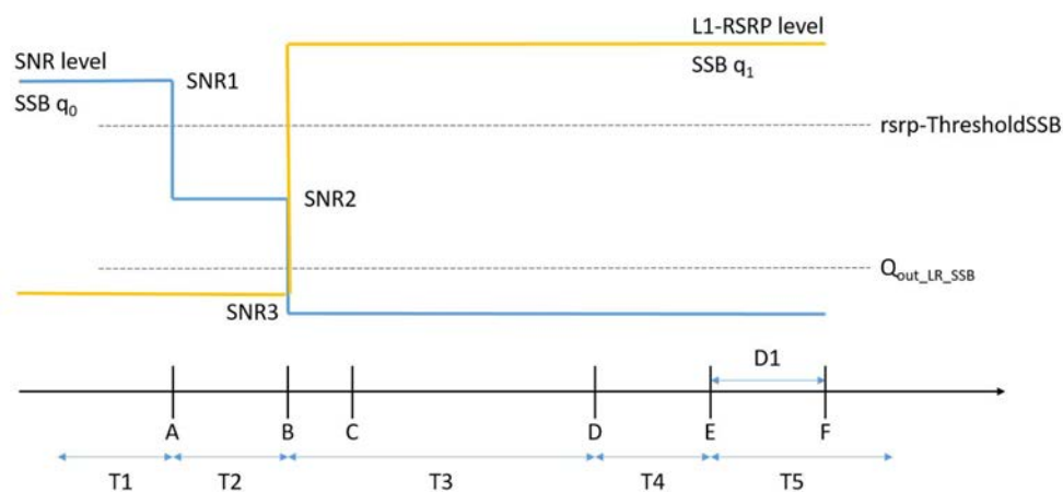
Figure A.11.4.2.1-1: SNR and L1-RSRP variation for SSB-based beam failure detection and link recovery testing in non-DRX mode
