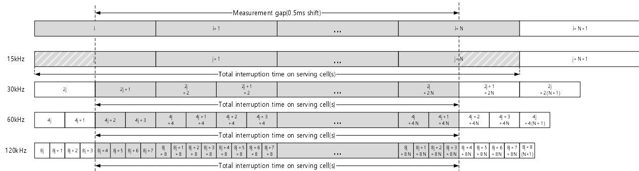
(b) Measurement gap with MGL = N(\text{ms}) with MG timing advance of 0.5ms for serving cell in synchronous NR standalone operation (with single carrier)
