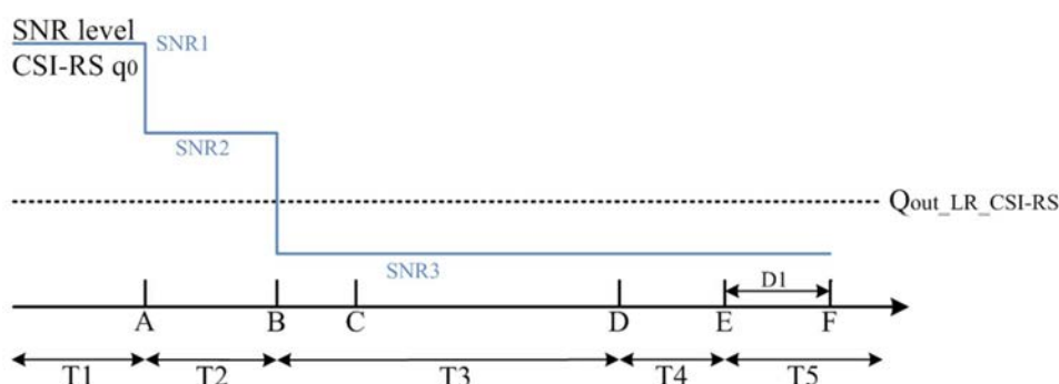
Figure A.17.5.2.4.1-1: SNR variation for CSI-RS-based beam failure detection and link recovery testing in DRX mode
