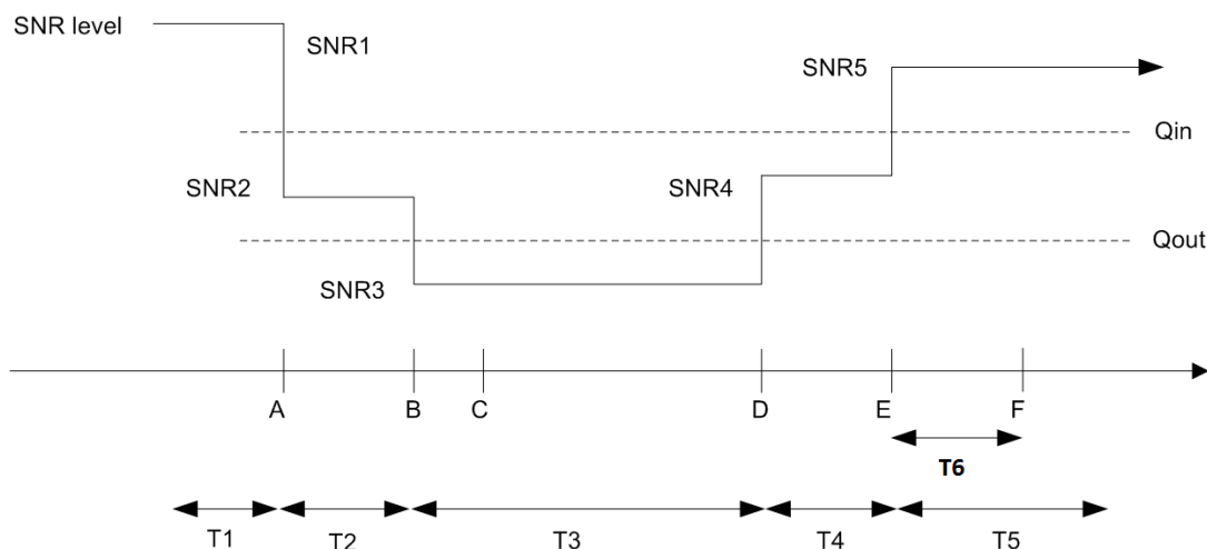
Figure A.14.4.1.6.1-1: SNR variation for CSI-RS in-sync testing
