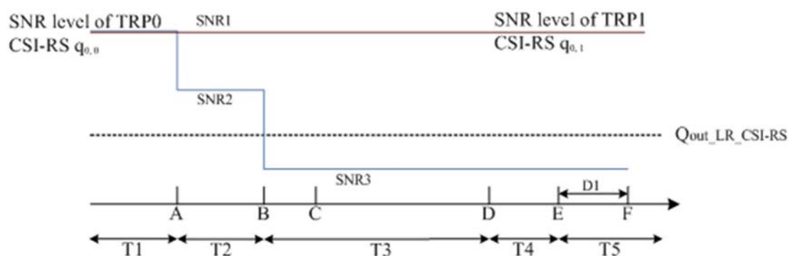
Figure A.4.5.5.8.1-1: SNR variation for beam failure detection and link recovery testing for TRP0 in non-DRX mode
