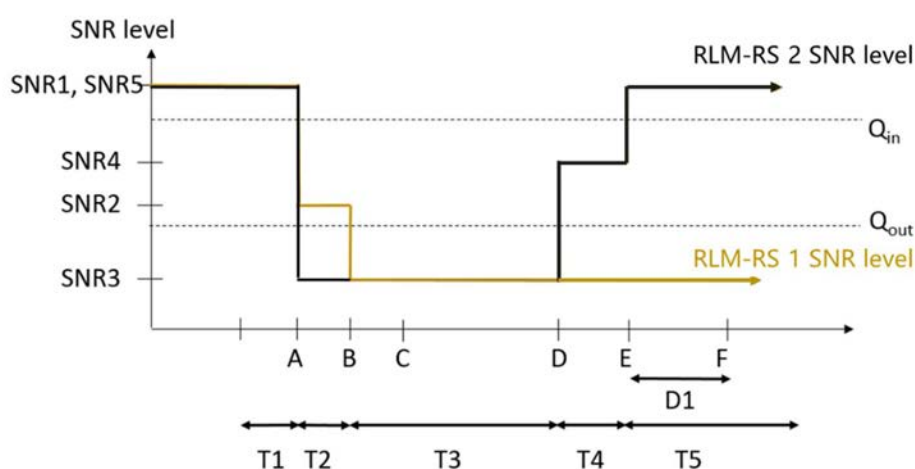
Figure A.17.5.1.6.1-1: SNR variation for CSI-RS in-sync testing
