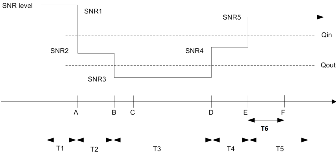
Figure A.14.4.1.8.1-1: SNR variation for CSI-RS in-sync testing
