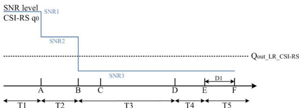
Figure A.17.5.2.3.1-1: SNR variation for CSI-RS based beam failure detection and link recovery testing in non-DRX mode
