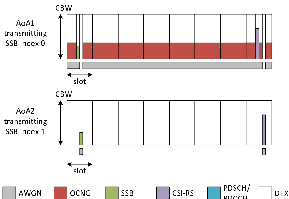
Figure A.17.5.1.9.1-1: Time multiplexed downlink transmissions
