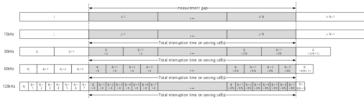
(a) Measurement gap with MGL = N(\text{ms}) with MG timing advance of 0ms for serving cell in synchronous NR standalone operation (with single carrier)
