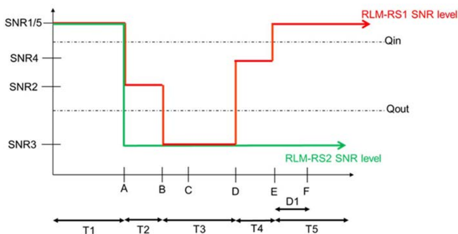
Figure A.17.5.1.8.1-1: SNR variation for CSI-RS in-sync testing
