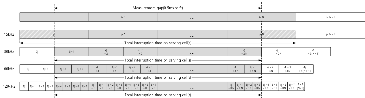
(b) Measurement gap with MGL = N(ms) with MG timing advance of 0.5ms for NR standalone operation configured with only single carrier
