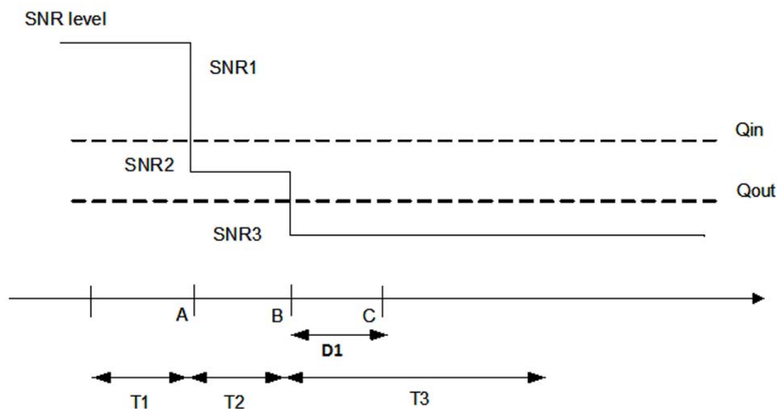
Figure A.16.5.1.5.1-1: SNR variation for out-of-sync testing
