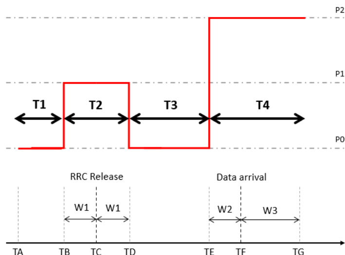
Figure A.7.2.1.1.1-1: RSRP variation for TA validation for CG-SDT Sub-test#1
