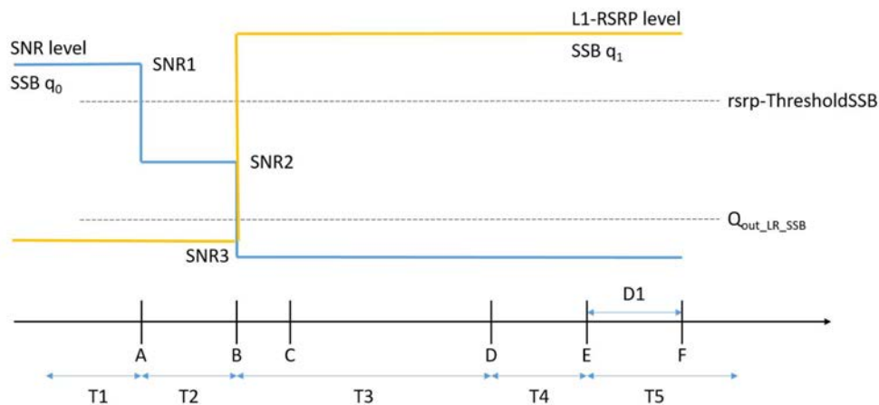
Figure A.16.5.2.2.1-1: SNR and L1-RSRP variation for SSB-based beam failure detection and link recovery testing in non-DRX mode
