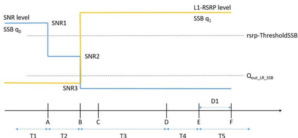
Figure A.14.4.2.2.1-1: SNR and L1-RSRP variation for SSB-based beam failure detection and link recovery testing in non-DRX mode
