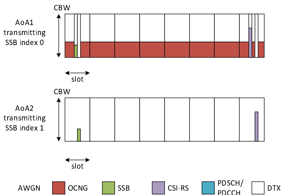
Figure A.7.6.1.8.1-1: Time multiplexed downlink transmissions (Config 1 example)
