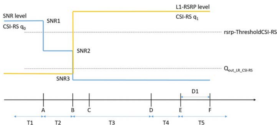
Figure A.14.4.2.4.1-1: SNR and L1-RSRP variation for CSI-RS-based beam failure detection and link recovery testing in DRX mode
