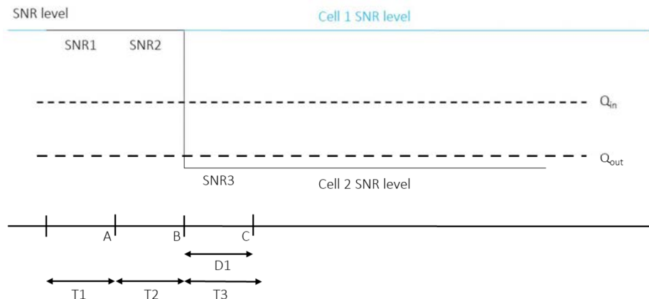
Figure A.4.5.1.9.1-1: SNR variation for out-of-sync testing
