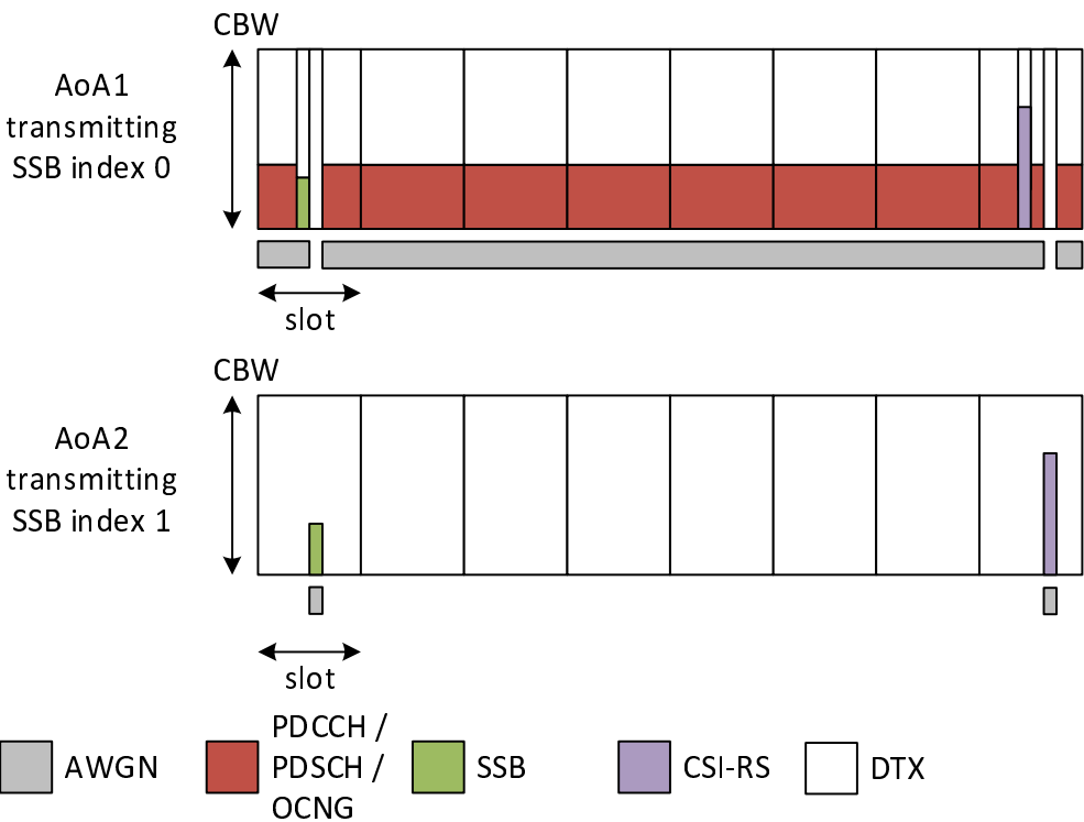
Figure A.17.5.4.1.1.1-1: Time multiplexed downlink transmissions during T1
