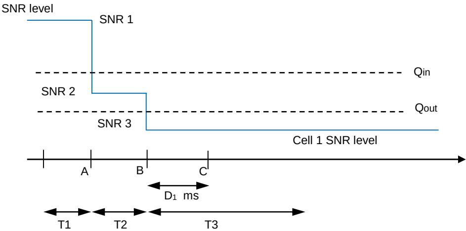
Figure A.16.5.1.9.1-1: SNR variation for CSI-RS out-of-sync testing
