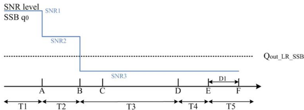
Figure A.17.5.2.2.1-1: SNR variation for SSB-based beam failure detection and link recovery testing in DRX mode
