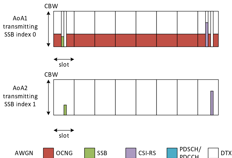
Figure A.15.4.1.1.1-1: Time multiplexed downlink transmissions (Config 1 example)
