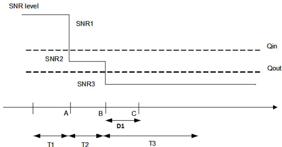
Figure A.11.4.1.2.1-1: SNR variation for out-of-sync testing.
