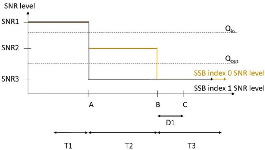
Figure A.17.5.1.1 .1-1: SNR variation for out-of-sync testing
