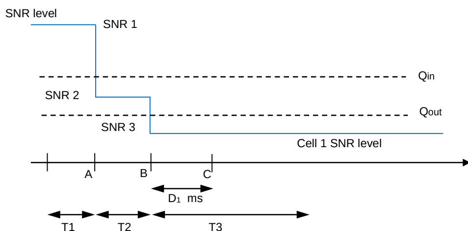
Figure A.14.4.1.7.1-1: SNR variation for CSI-RS out-of-sync testing
