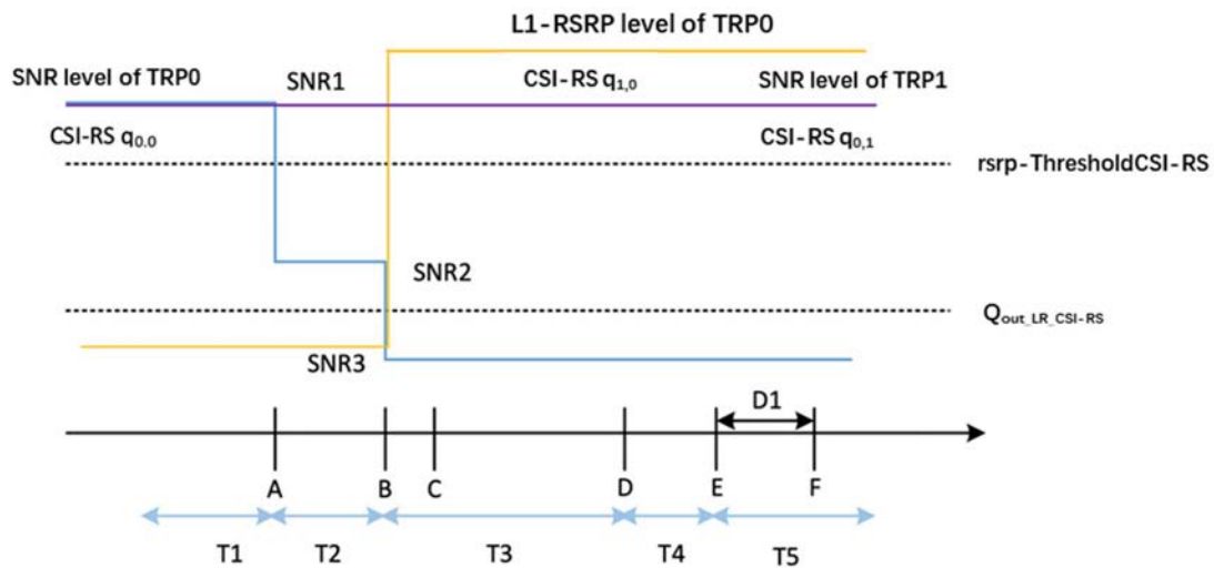
Figure A.5.5.8.1-1: SNR and L1-RSRP variation for CSI-RS-based beam failure detection and link recovery testing in DRX mode
