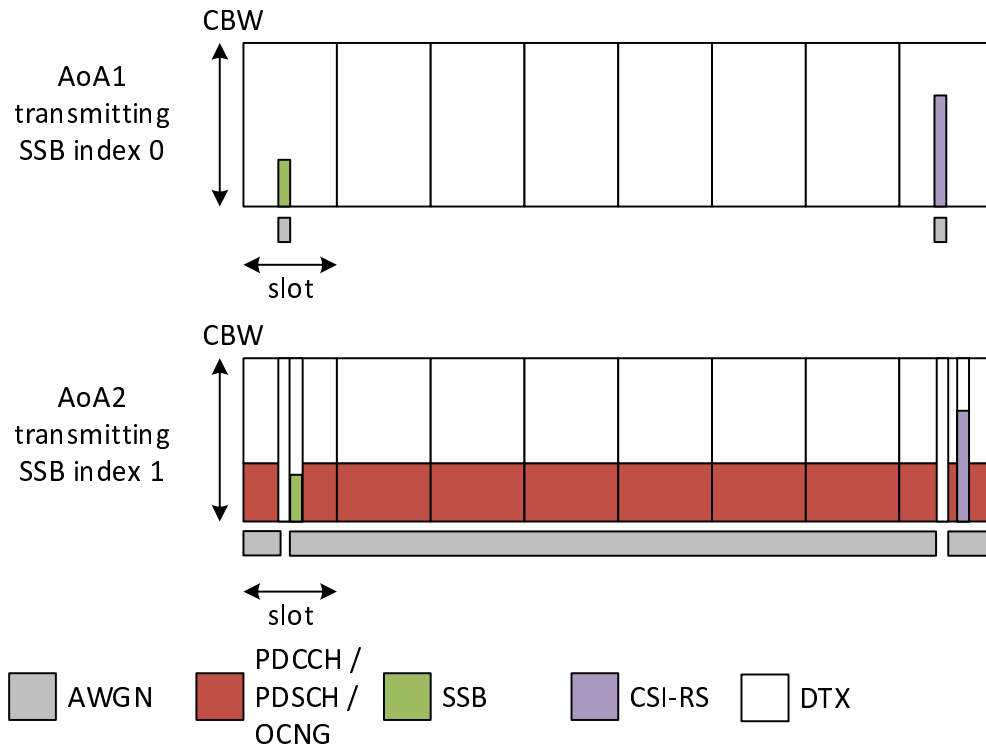
Figure A.5.5.11.3.1.1-2: Time multiplexed downlink transmissions during T2
