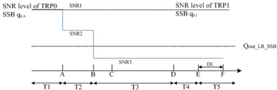
Figure A.4.5.5.7.1-1: SNR variation for SSB-based beam failure detection and link recovery testing in non-DRX mode
