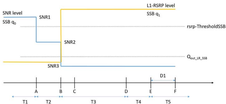
Figure A.14.4.2.1.1-1: SNR and L1-RSRP variation SSB for SSB-based beam failure detection and link recovery testing in non-DRX mode
