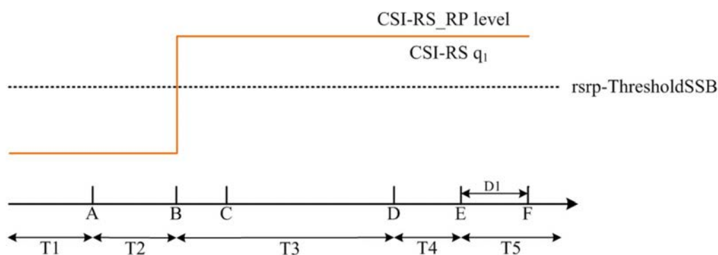
Figure A.17.5.2.4.1-2: CSI-RS_RP level variation for CSI-RS based beam failure detection and link recovery testing in DRX mode
