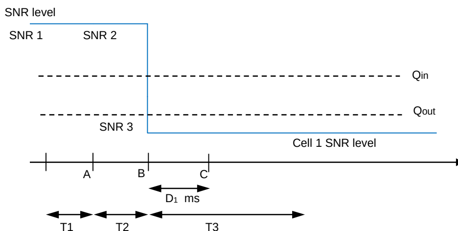
Figure A.6.5.1.9.1-1: SNR variation for CSI-RS out-of-sync testing
