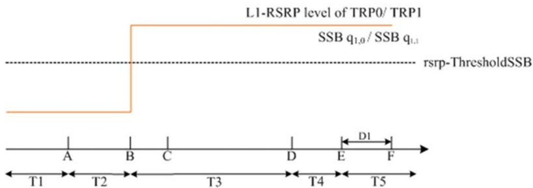
Figure A.4.5.5.7.1-2: L1-RSRP level variation for SSB-based beam failure detection and link recovery testing in non-DRX mode
