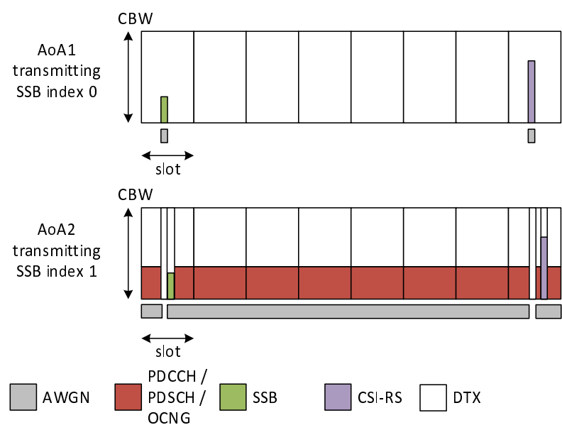
Figure A.7.5.8.3.1.1-2: Time multiplexed downlink transmissions during T2
