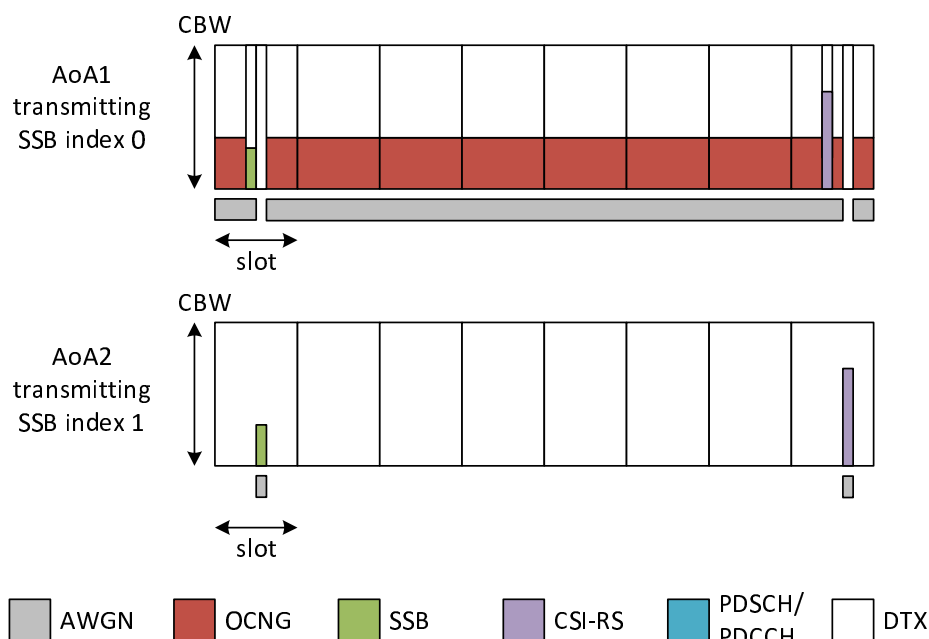
Figure A.17.5.1.3.1-2: Time multiplexed downlink transmissions
