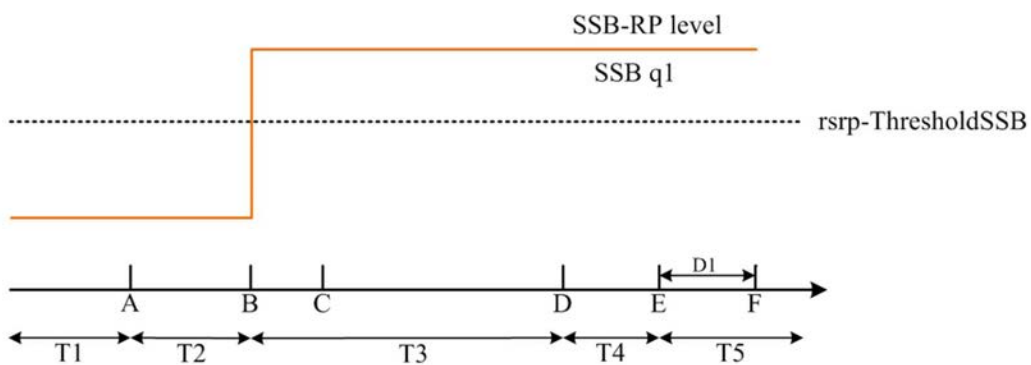
Figure A.17.5.2.2.1-2: SSB_RP level variation for SSB-based beam failure detection and link recovery testing in DRX mode
