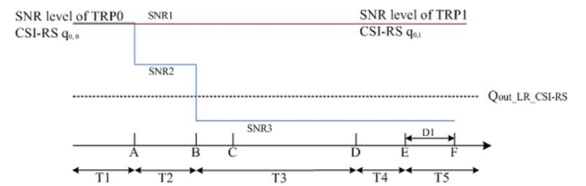
Figure A.6.5.7.1-1: SNR variation for CSI-RS-based beam failure detection and link recovery testing in DRX mode
