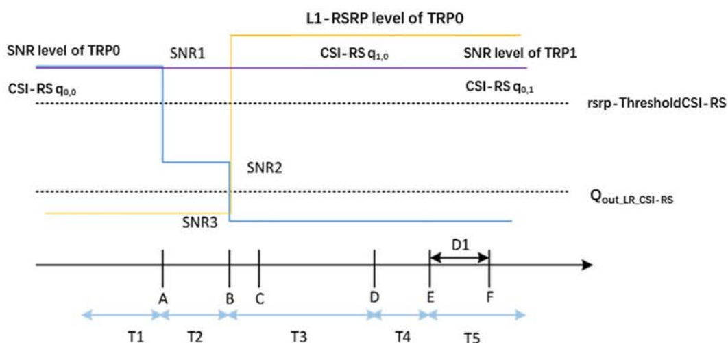
Figure A.7.5.5.9.1-1: SNR and L1-RSRP variation for beam failure detection and link recovery testing for SCell in DRX mode
