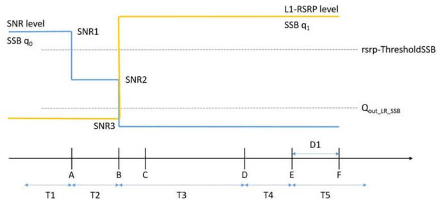
Figure A.7.5.5.13.1-1: SNR and L1-RSRP variation SSB for SSB-based beam failure detection and link recovery testing in non-DRX mode
