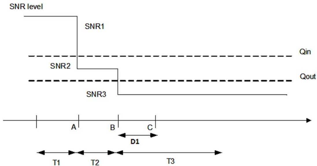
Figure A.14.4.1.3.1-1: SNR variation for out-of-sync testing
