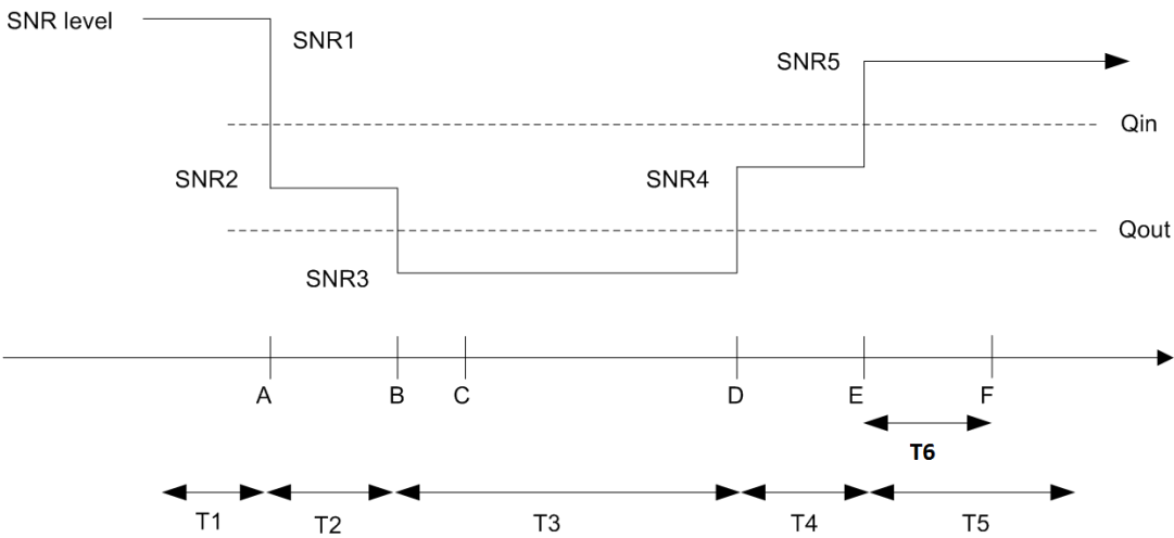
Figure A.16.5.1.15.1-1: SNR variation for CSI-RS in-sync testing
