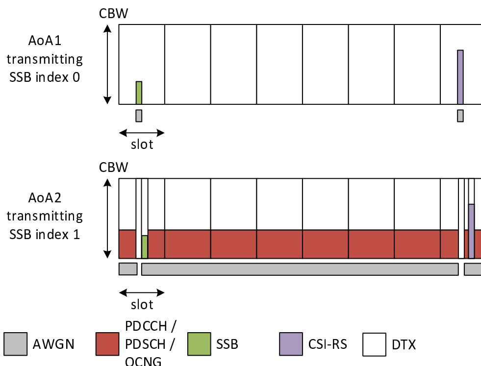
Figure A.17.5.4.2.1.1-2: Time multiplexed downlink transmissions during T2
