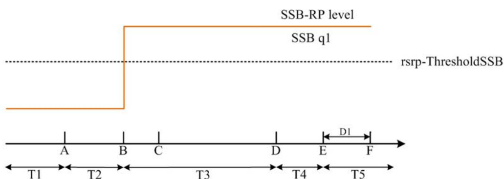
Figure A.17.5.2.1.1-2: SSB_RP level variation for SSB-based beam failure detection and link recovery testing in non-DRX mode
