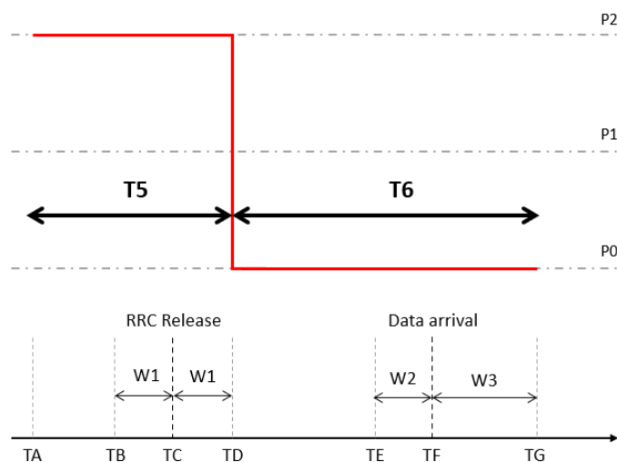
Figure A.17.2.1.1.1-2: RSRP variation model for CG-SDT Sub-test#2
