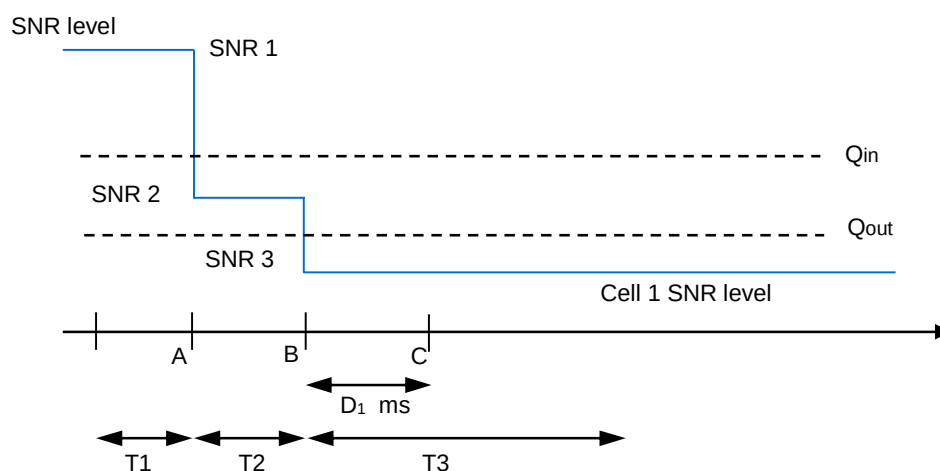
Figure A.16.5.1.10.1-1: SNR variation for CSI-RS out-of-sync testing
