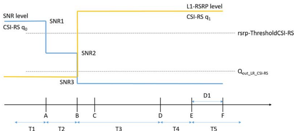
Figure A.7.5.5.11.1-1: SNR and L1-RSRP variation for CSI-RS based beam failure detection and link recovery testing in non-DRX mode
