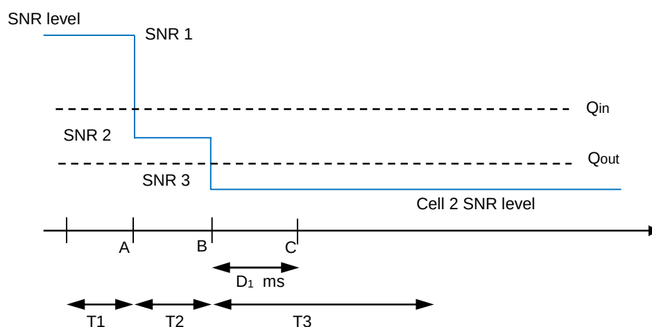
Figure A.16.5.1.13.1-1: SNR variation for CSI-RS out-of-sync testing
