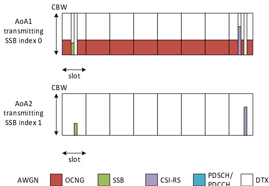
Figure A.17.6.1.1.1-1: Time multiplexed downlink transmissions (Config 1 example)
