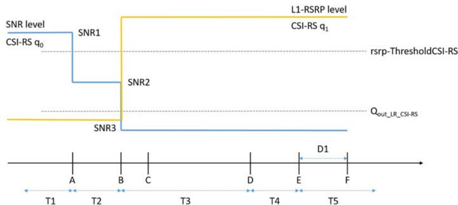
Figure A.16.5.2.8.1-1: SNR and L1-RSRP variation for CSI-RS-based beam failure detection and link recovery testing in DRX mode
