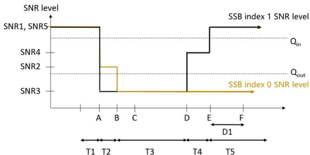
Figure A.17.5.1.2.1-1: SNR variation for in-sync testing
