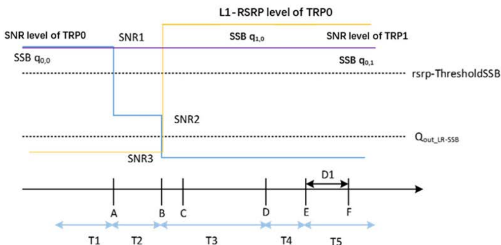
Figure A.7.5.5.10.1-1: SNR and L1-RSRP variation SSB for SSB-based beam failure detection and link recovery testing in non-DRX mode
