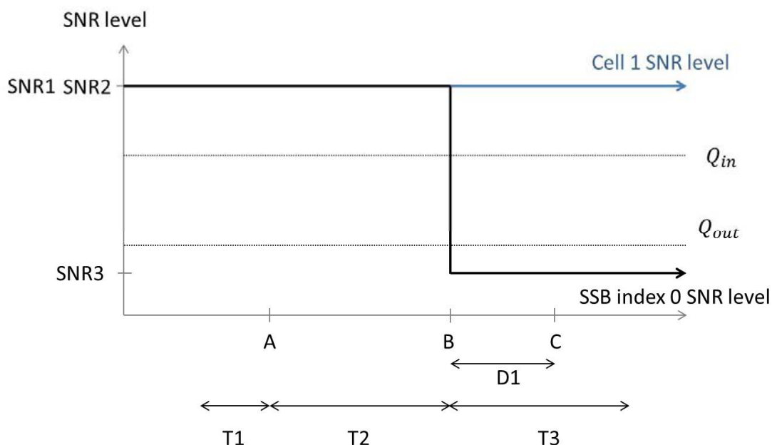
Figure A.5.5.1.10.1-1: SNR variation for out-of-sync testing
