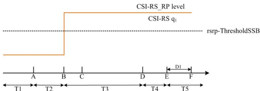
Figure A.17.5.2.3.1-2: CSI-RS_RP level variation for CSI-RS based beam failure detection and link recovery testing in non-DRX mode
