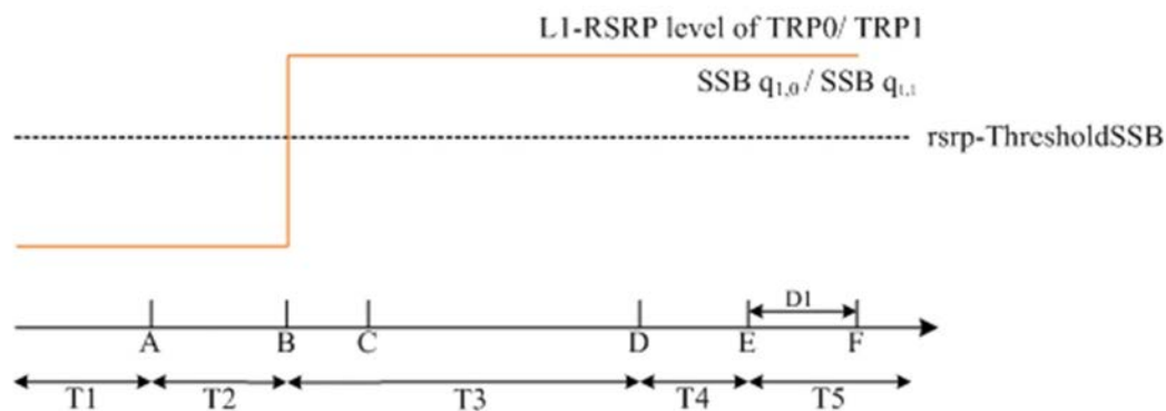
Figure A.4.5.5.8.1-2: L1-RSRP level variation for beam failure detection and link recovery testing for TRP 0 in non-DRX mode
