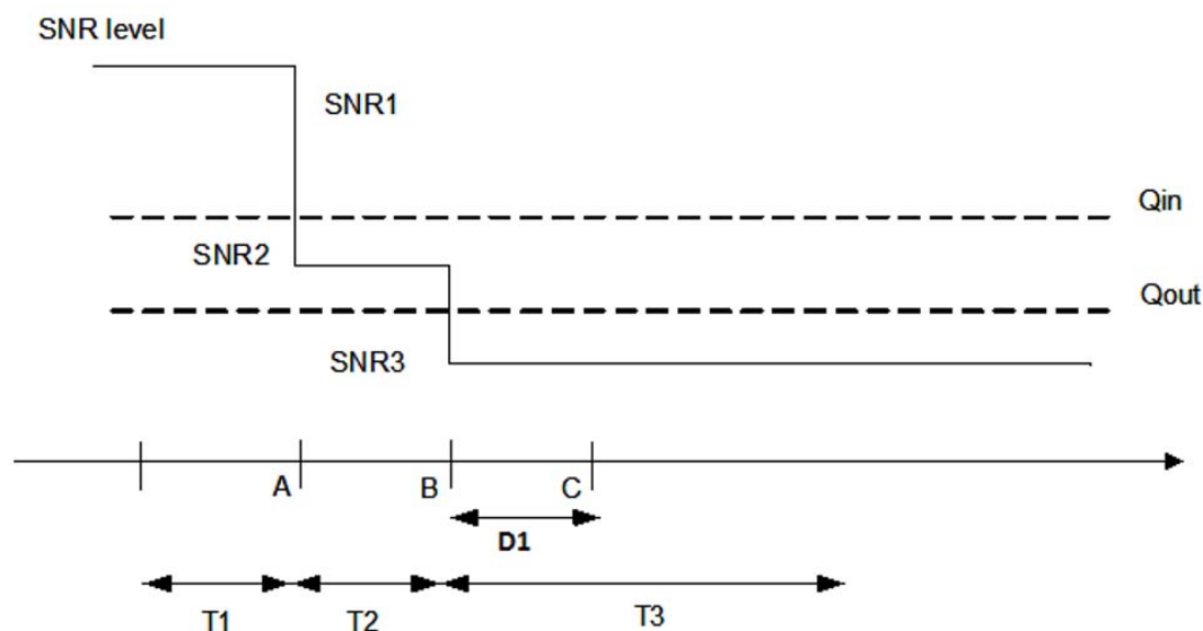
Figure A.14.4.1.1.1-1: SNR variation for out-of-sync testing
