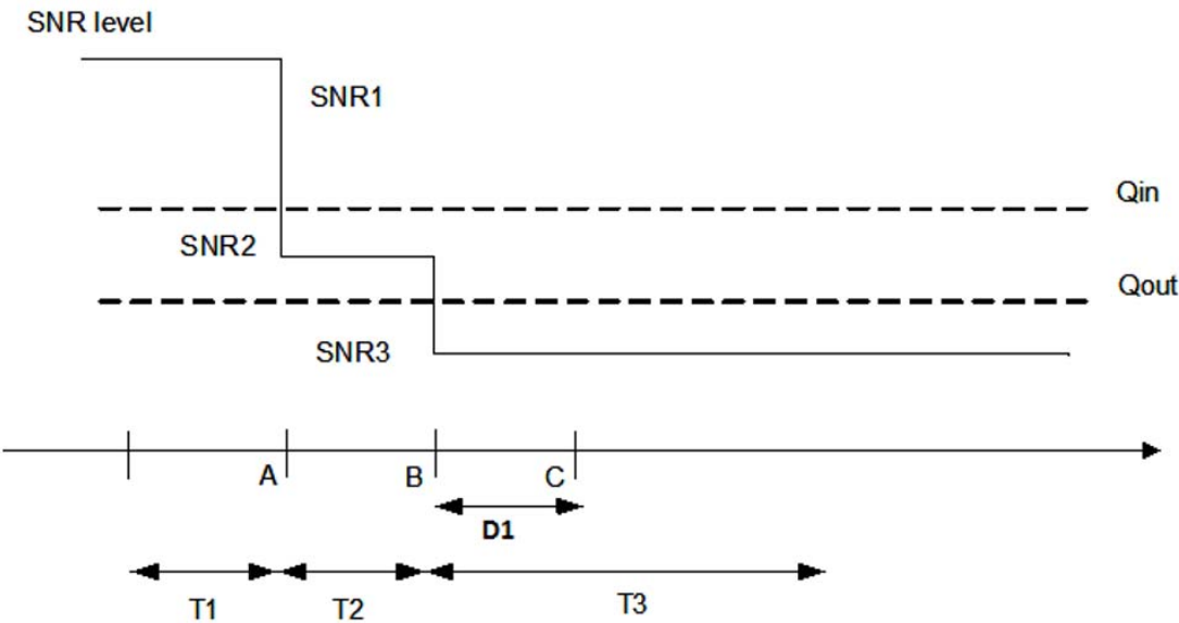
Figure A.16.5.1.2.1-1: SNR variation for out-of-sync testing
