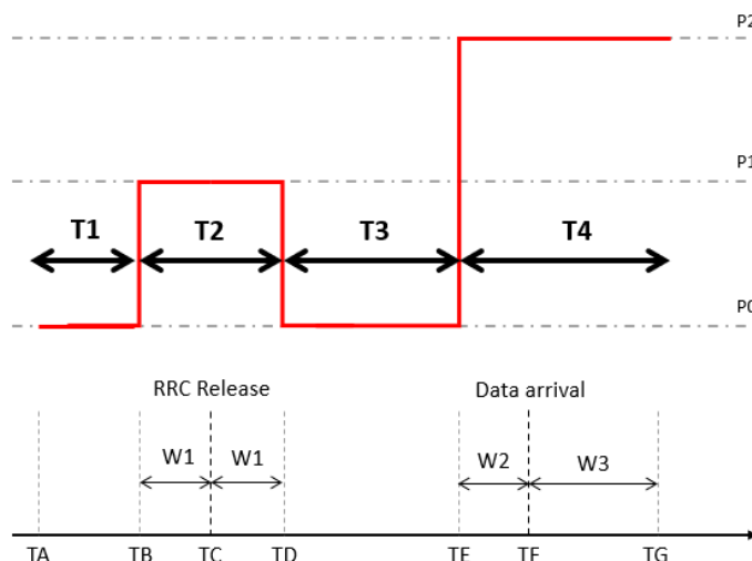
Figure A.6.2.1.1-1: RSRP variation model for CG-SDT Sub-test#1
