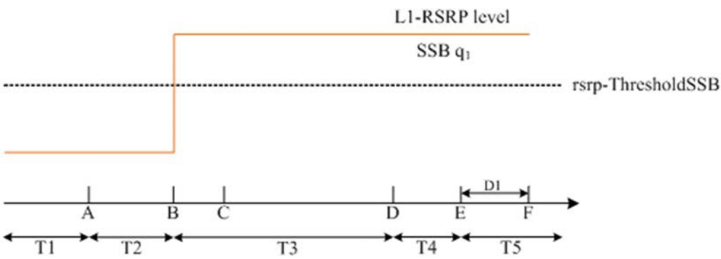
Figure A.4.5.5.2.1-2: L1-RSRP level variation for SSB-based beam failure detection and link recovery testing in DRX mode
