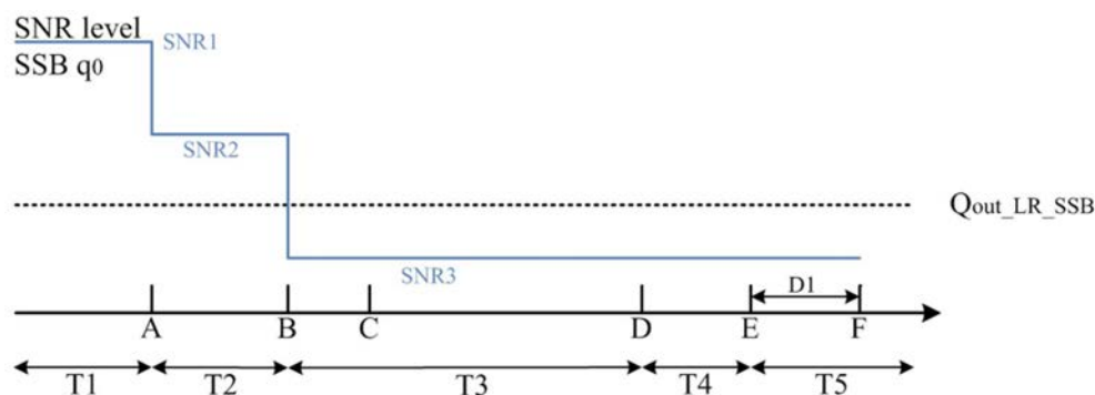
Figure A.17.5.2.5.1-1: SNR variation SSB for SSB-based beam failure detection and link recovery testing in non-DRX mode
