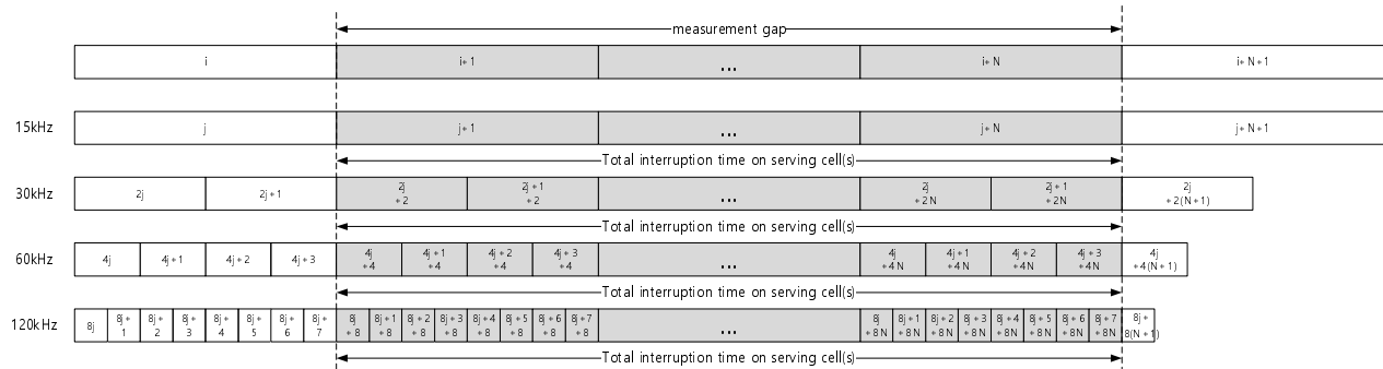
(a) Measurement gap with MGL = N(ms) with MG timing advance of 0ms for NR standalone operation configured with only single carrier
