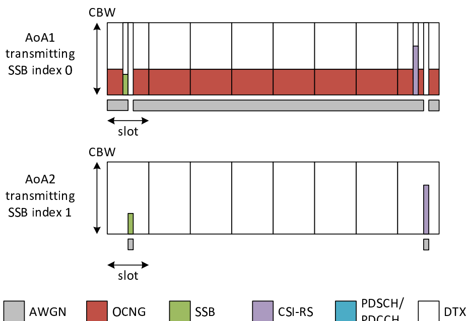
Figure A.17.5.1.1 .1-2: Time multiplexed downlink transmissions
