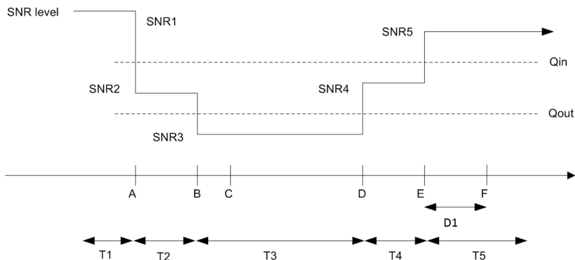
Figure A.10.3.1.2.1-1: SNR variation for in-sync testing.
