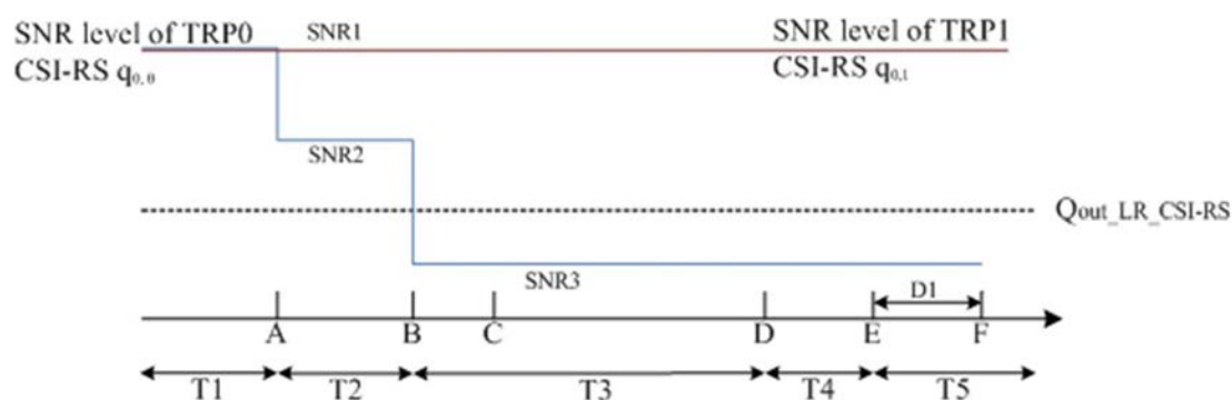
Figure A.6.5.7.1-1: SNR variation for CSI-RS-based beam failure detection and link recovery testing in DRX mode
