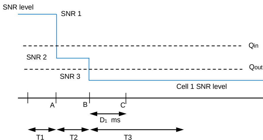
Figure A.6.5.1.5.1-1: SNR variation for CSI-RS out-of-sync testing
