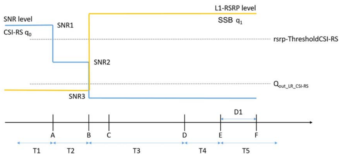
Figure A.14.4.2.5.1-1: SNR and L1-RSRP variation for beam failure detection and link recovery testing in for SCell non-DRX mode
