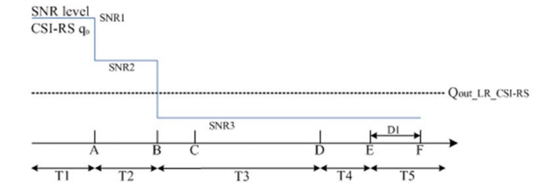
Figure A.6.5.5.3.1-1: SNR variation for CSI-RS-based beam failure detection and link recovery testing in non-DRX mode
