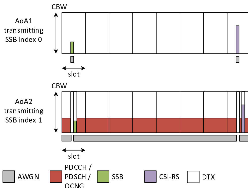
Figure A.5.5.11.3.1.1-2: Time multiplexed downlink transmissions during T2
