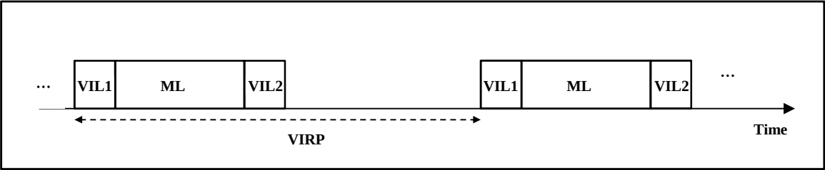
Figure 9.1.9.3-1: Illustration of NCSG parameters: VIL1, ML, VIL2 and VIRP
