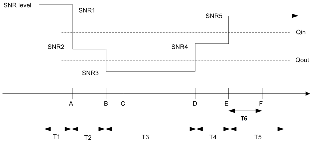
Figure A.16.5.1.11.1-1: SNR variation for CSI-RS in-sync testing
