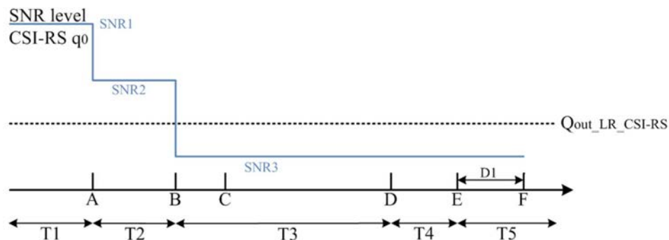
Figure A.17.5.2.4.1-1: SNR variation for CSI-RS-based beam failure detection and link recovery testing in DRX mode
