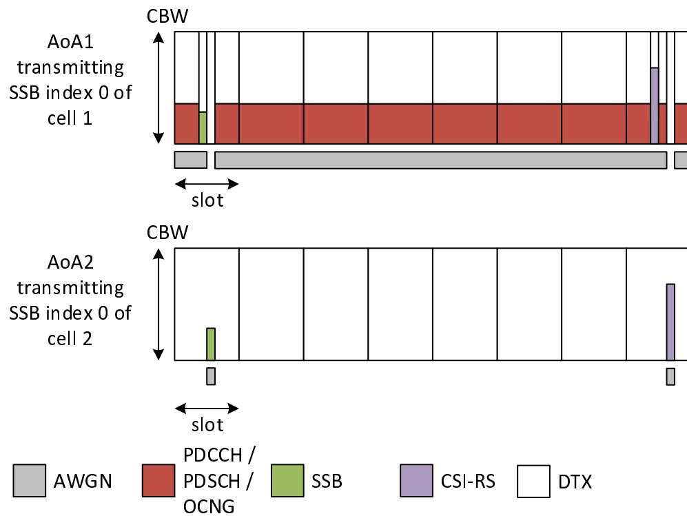
Figure A.7.5.13.3.1.2-1: Time multiplexed downlink transmissions during T1
