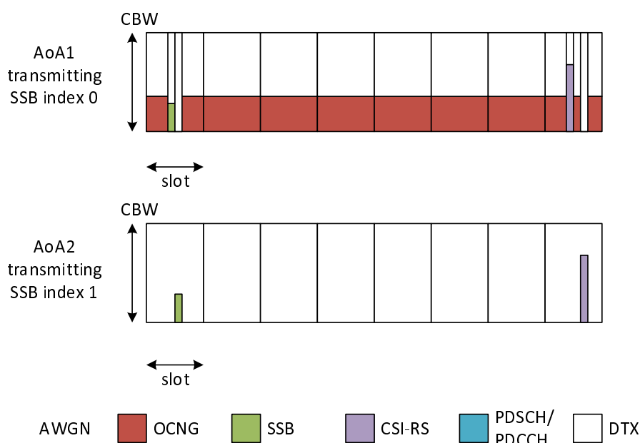
Figure A.7.6.1.1-1: Time multiplexed downlink transmissions (Config 1 example)
