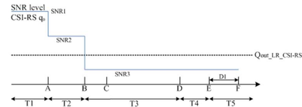
Figure A.4.5.5.6.1-1: SNR variation for beam failure detection and LR testing for SCell in DRX mode
