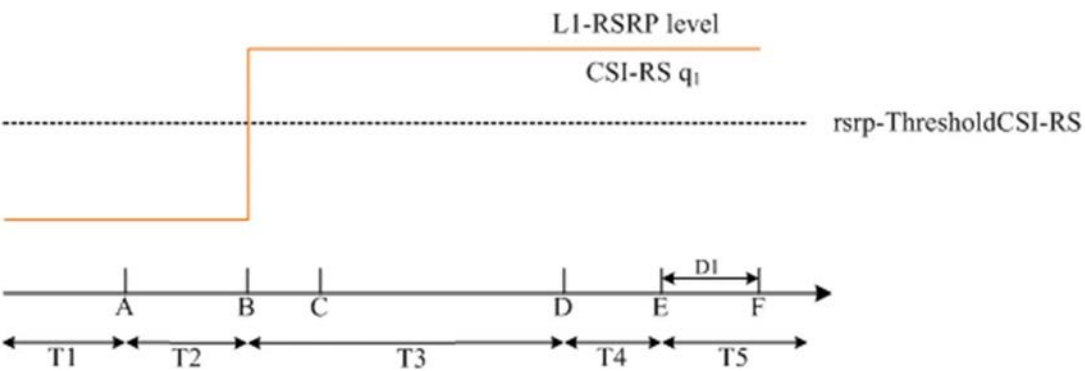
Figure A.4.5.5.4.1-2: L1-RSRP level variation for CSI-RS based beam failure detection and link recovery testing in DRX mode
