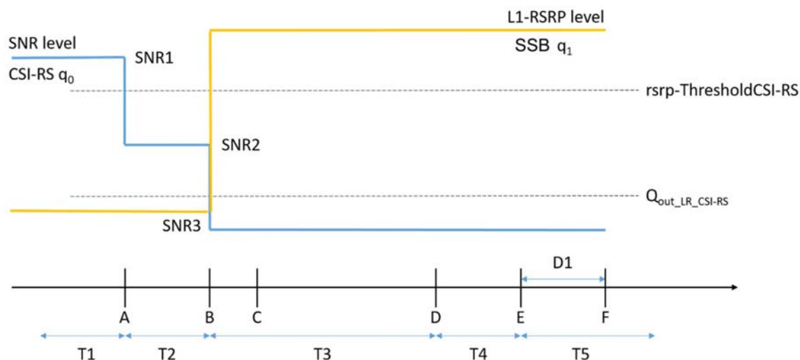
Figure A.14.4.2.6.1-1: SNR and L1-RSRP variation for beam failure detection and link recovery testing for SCell in DRX mode
