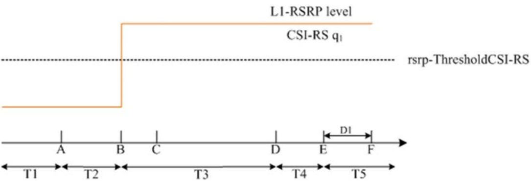
Figure A.6.5.5.3.1-2: L1-RSRP level variation for CSI-RS based beam failure detection and link recovery testing in non-DRX mode
