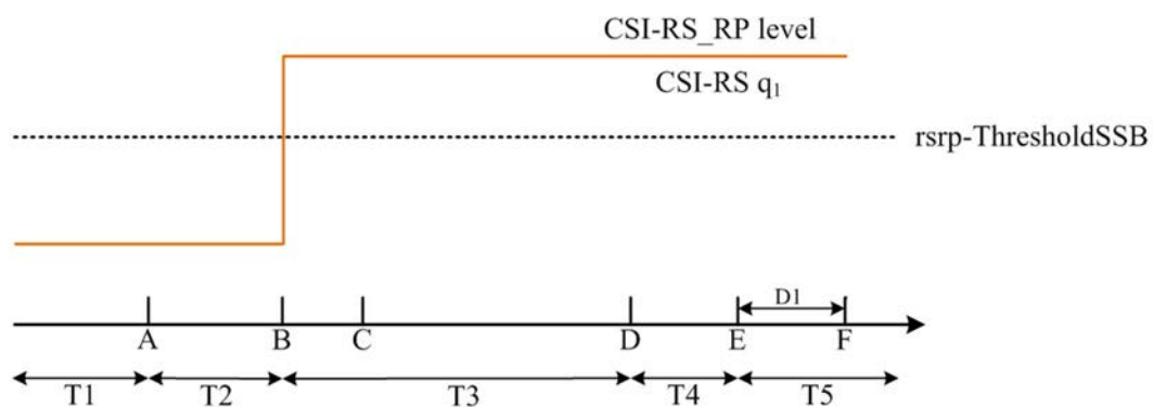
Figure A.5.5.5.6.1-2: CSI-RS_RP level variation for CSI-RS based beam failure detection and link recovery testing for SCell in non-DRX mode
