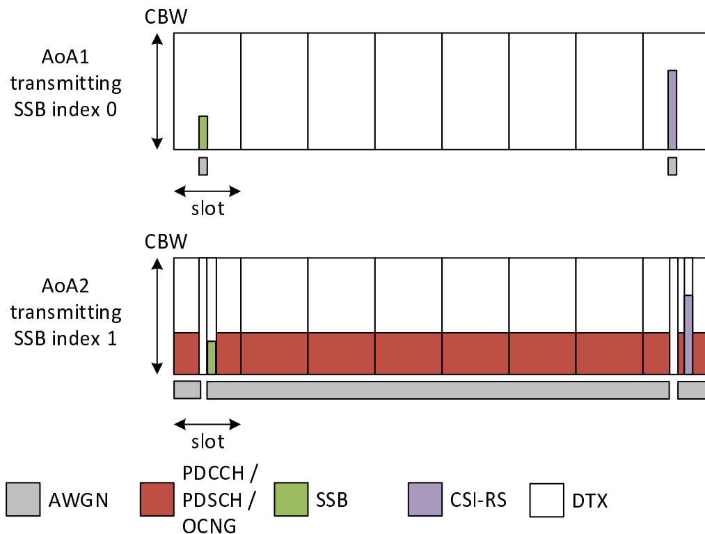
Figure A.7.5.8.1.1.1-2: Time multiplexed downlink transmissions during T2
