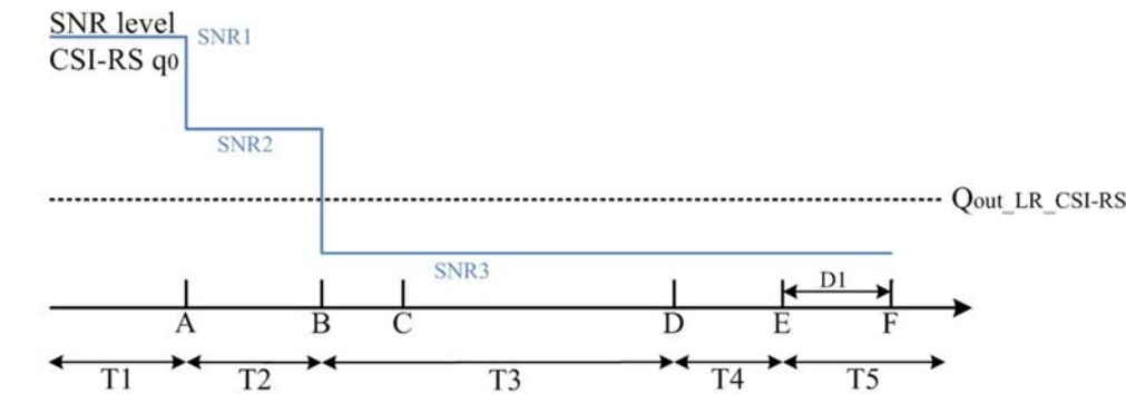
Figure A.5.5.5.4.1-1: SNR variation for CSI-RS-based beam failure detection and link recovery testing in DRX mode
