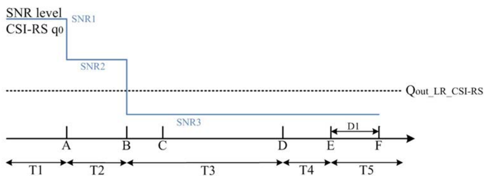
Figure A.5.5.5.6.1-1: SNR variation for CSI-RS based beam failure detection and link recovery testing for SCell in non-DRX mode
