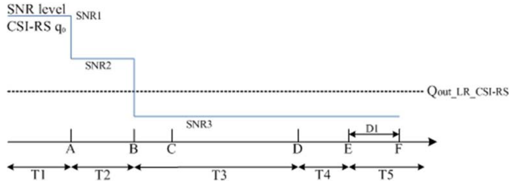
Figure A.4.5.5.4.1-1: SNR variation for CSI-RS-based beam failure detection and link recovery testing in DRX mode
