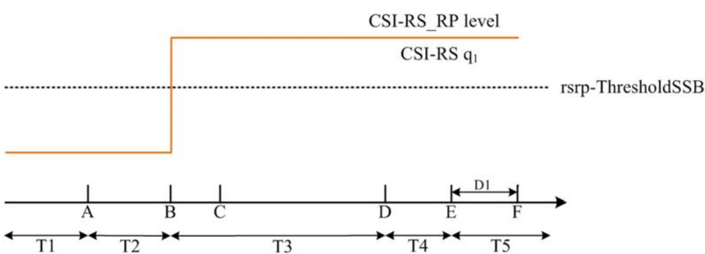
Figure A.5.5.5.3.1-2: CSI-RS_RP level variation for CSI-RS based beam failure detection and link recovery testing in non-DRX mode
