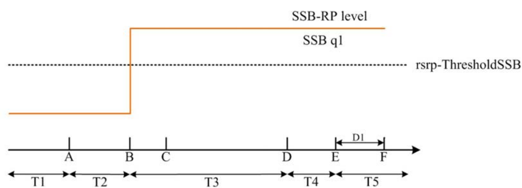
Figure A.7.5.5.2.1-2: SSB_RP level variation for SSB-based beam failure detection and link recovery testing in DRX mode
