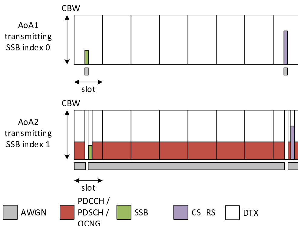
Figure A.5.5.8.1.1.1-2: Time multiplexed downlink transmissions during T2
