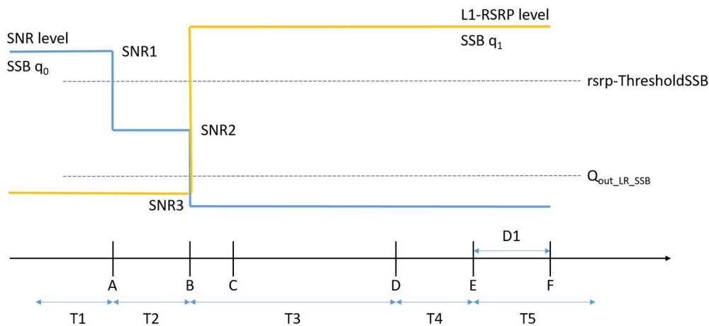
Figure A.7.5.5.1.1-1: SNR and L1-RSRP variation SSB for SSB-based beam failure detection and link recovery testing in non-DRX mode
