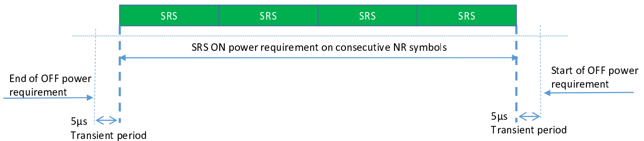
Figure 9.3.3.6-2: Consecutive SRS time mask for the case when no power change is required in FR2-NTN
