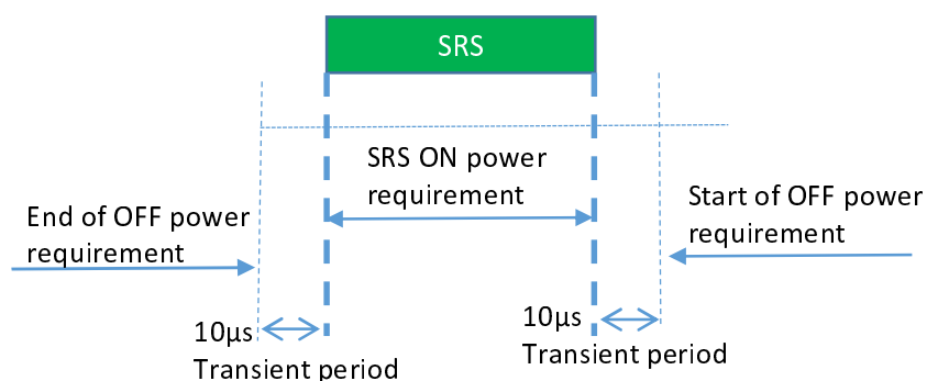
Figure 9.3.3.6-1a: Single SRS time mask for NR UL transmission in FR1-NTN above 10 GHz
