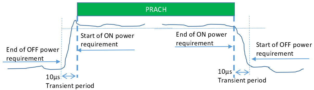
Figure 9.3.3.4-1a: PRACH ON/OFF time mask in FR1-NTN above 10 GHz
