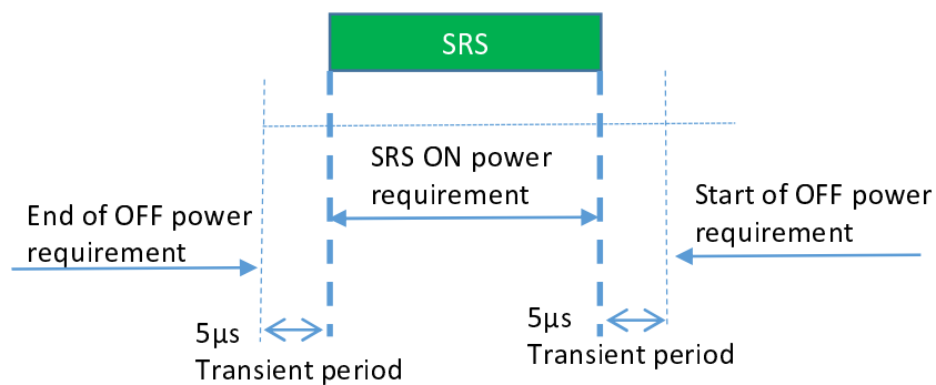
Figure 9.3.3.6-1: Single SRS time mask for NR UL transmission in FR2-NTN
