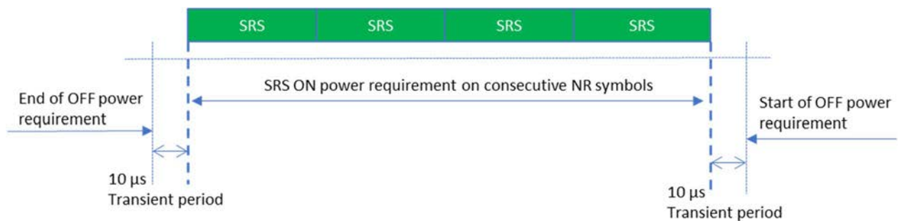
Figure 9.3.3.6-2a: Consecutive SRS time mask for the case when no power change is required in FR1-NTN above 10 GHz
