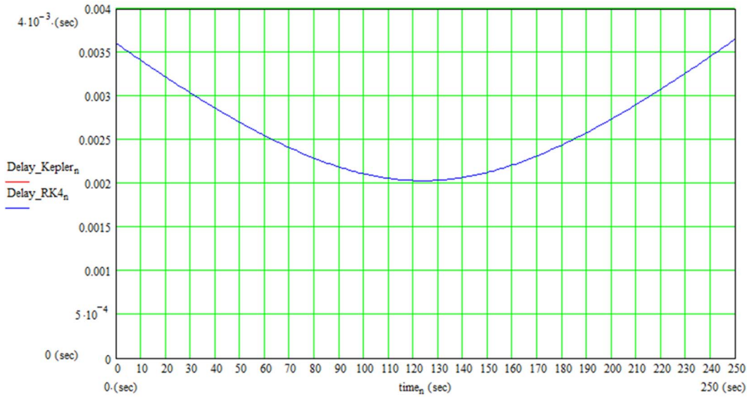
Figure G.3.2-2: Propagation delay of LEO-600 calculated by Newton-Raphson method and fourth-order Runge-Kutta method
