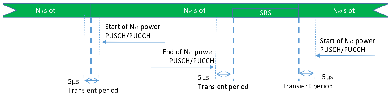
Figure 9.3.3.7-1: PUCCH/PUSCH/SRS time mask when there is a transmission before or after or both before and after SRS in FR2-NTN
