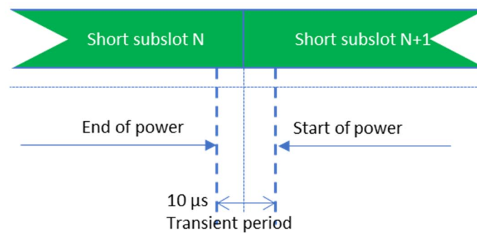
Figure 9.3.3.9-1a: Consecutive short subslot transmissions time mask where DMRS is not the first symbol in the adjacent short subslot transmission in FR1-NTN above 10 GHz
