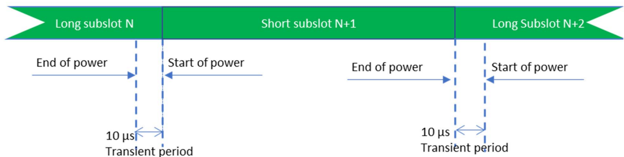
Figure 9.3.3.8-1a Consecutive slot or long subslot transmission and short subslot transmission time mask in FR1-NTN above 10 GHz
