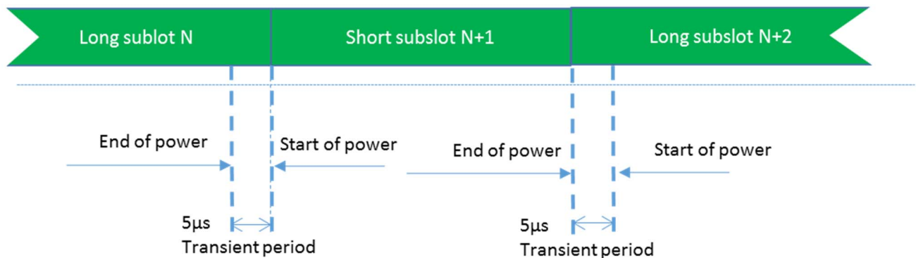
Figure 9.3.3.8-1: Consecutive slot or long subslot transmission and short subslot transmission time mask in FR2-NTN
