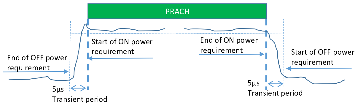
Figure 9.3.3.4-1: PRACH ON/OFF time mask in FR2-NTN
