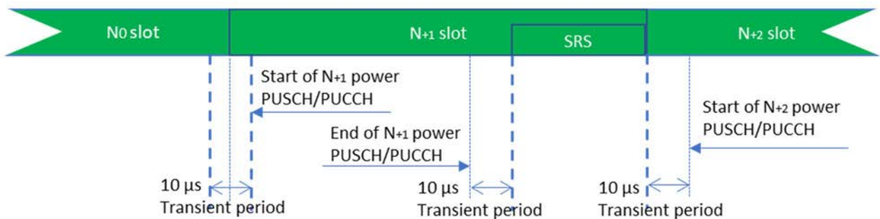
Figure 9.3.3.7-1a: PUCCH/PUSCH/SRS time mask when there is a transmission before or after or both before and after SRS in FR1-NTN above 10 GHz
