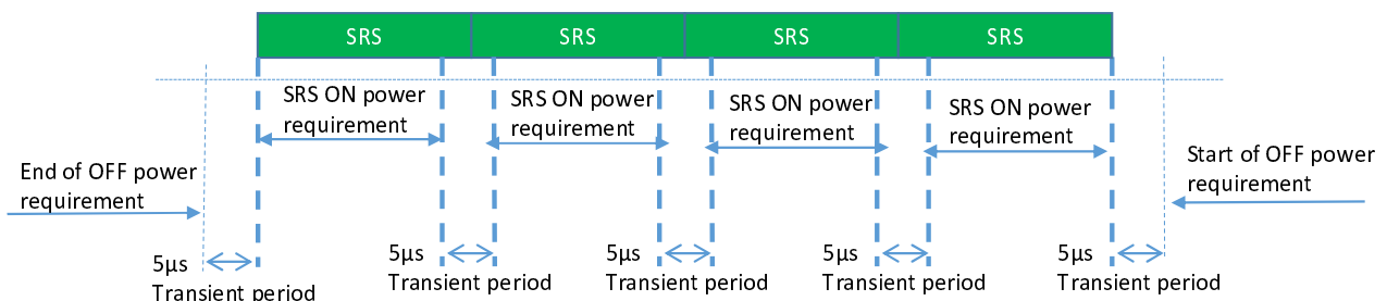
Figure 9.3.3.6-3: Consecutive SRS time mask for the case when power change is required and when 60kHz SCS is used in FR2-NTN
