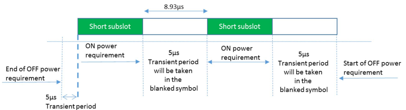
Figure 9.3.3.9-2: Consecutive short subslot (1 symbol gap) time mask for the case when transient period is required on both sides of the symbol and when 120 kHz SCS is used in FR2-NTN
