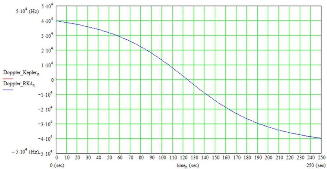
Figure G.3.2-1: Doppler shift of LEO-600 calculated by Newton-Raphson method and fourth-order Runge-Kutta method
