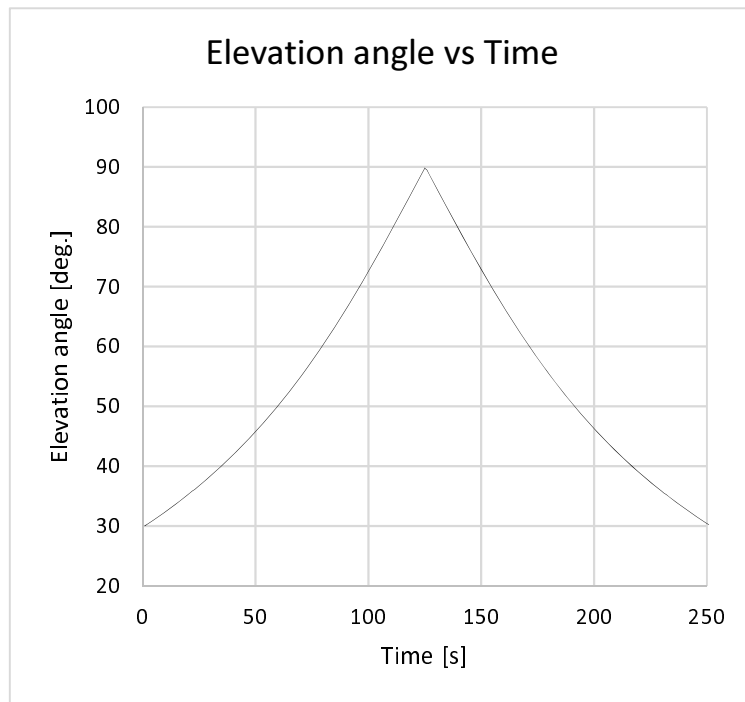
Figure G.3.3-1: Elevation angle for LEO-600 with maximum positive Doppler scenario
