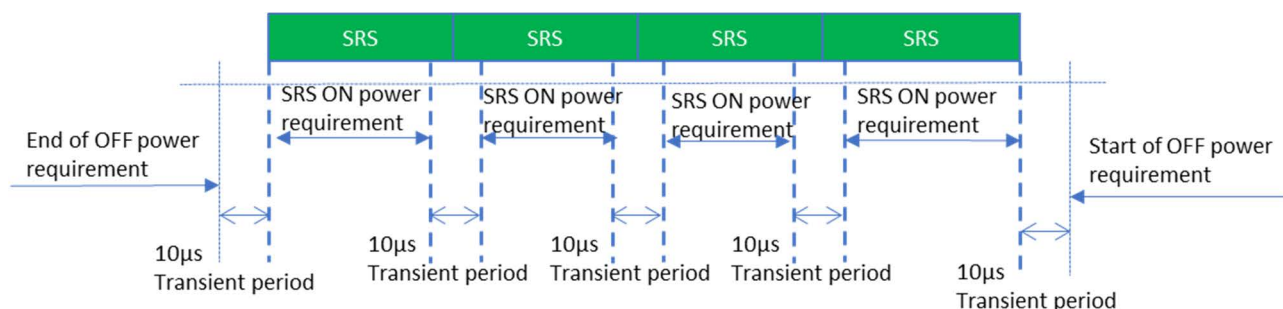
Figure 9.3.3.6-3a: Consecutive SRS time mask for the case when power change is required and when 15kHz and 30kHz SCS is used in FR1-NTN above 10 GHz
