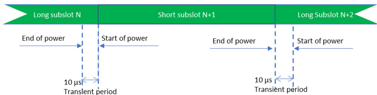
Figure 9.3.3.8-1a Consecutive slot or long subslot transmission and short subslot transmission time mask in FR1-NTN above 10 GHz
