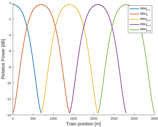
Figure B.3.5-2 Relative power level trajectories
