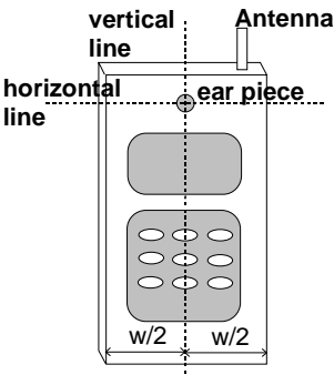
Figure 4.3.1-3: Reference lines at a DUT
