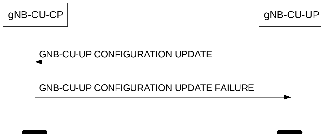
Figure 8.2.5.3-1: gNB-CU-UP Configuration Update procedure: Unsuccessful Operation.
