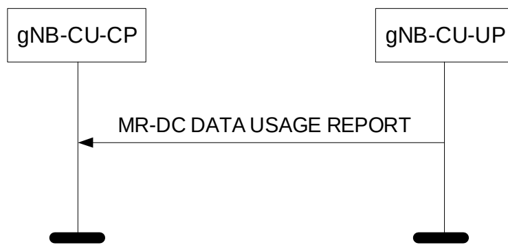
Figure 8.3.11.2-1: MR-DC Data Usage Report procedure: Successful Operation.
