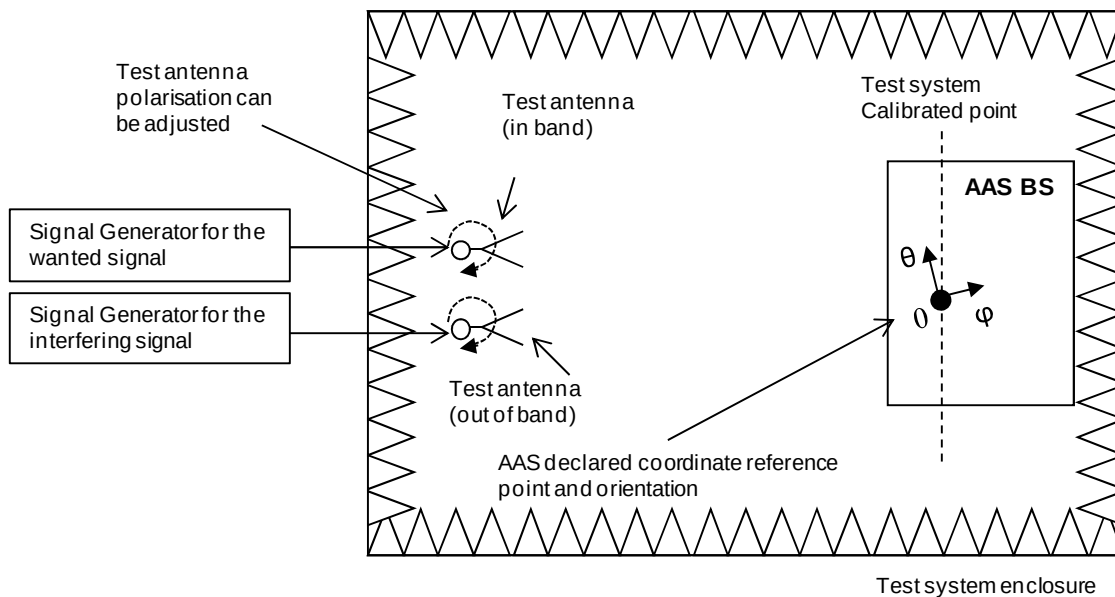
Figure D.2.4-1: Measurement set up for OTA Blocking
