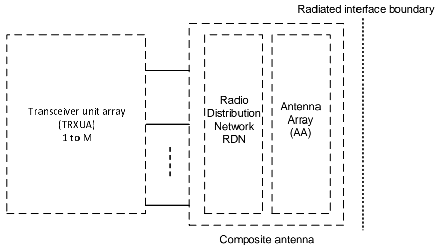
Figure 4.3-2: Radiated points of reference of OTA AAS BS
