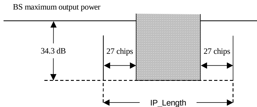
Figure 6.4.5.5-1: IPDL Time Mask
