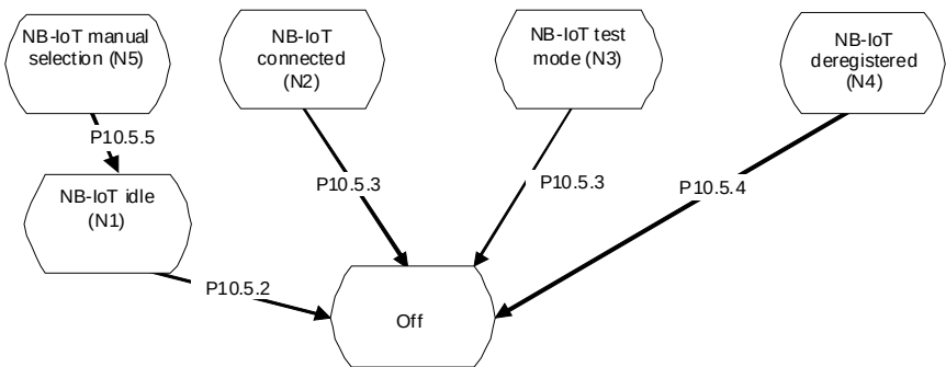
Figure 10.5.1-1: UE postamble states and procedures for NB-IoT
