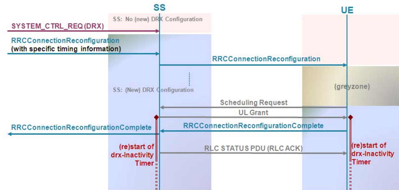
Figure 7.15-1: DRX (Re)configuration
