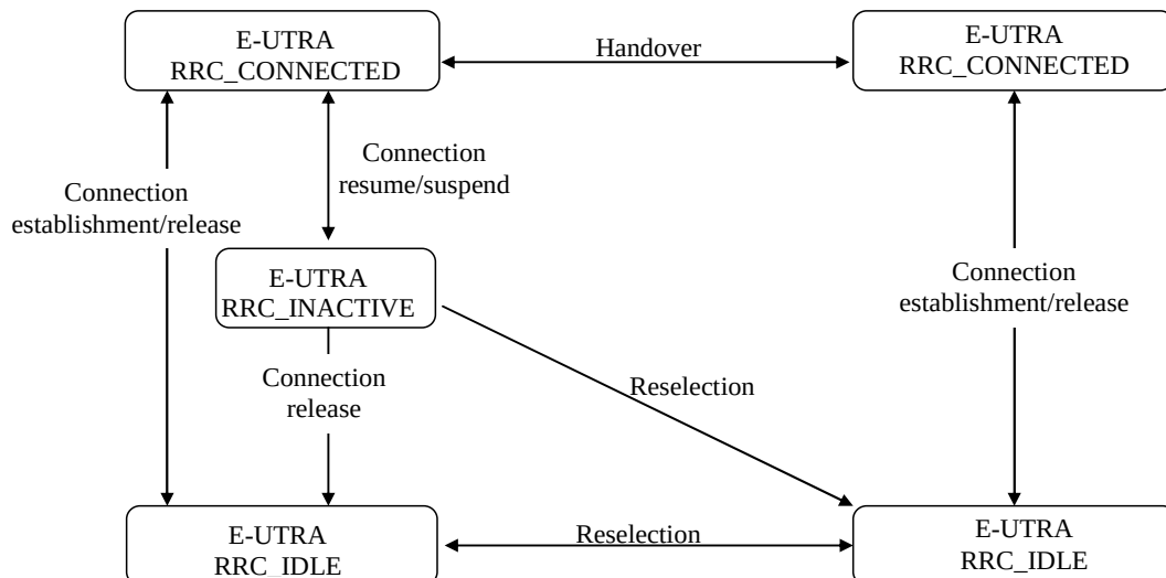
Figure 4.2.1-5: Mobility procedures between E-UTRA/5GC and E-UTRA/EPC
