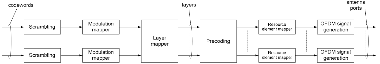
Figure 6.3-1: Overview of physical channel processing
