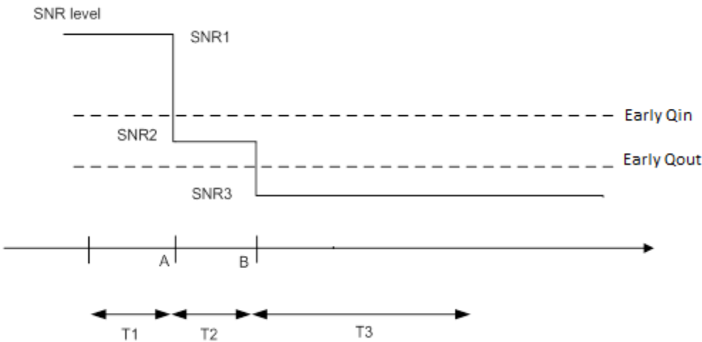
Figure A.7.3.101.1-1: SNR variation for early out-of-sync testing
