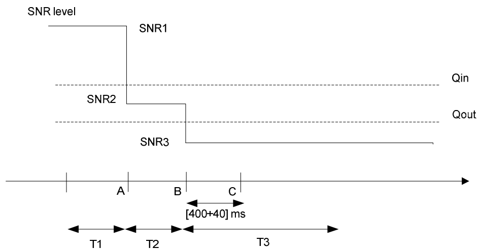
Figure A.7.3.97.1-1: SNR variation for out-of-sync testing
