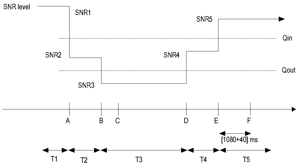
Figure A.14.4.3.6.1-1: SNR variation for in-sync testing in DRX
