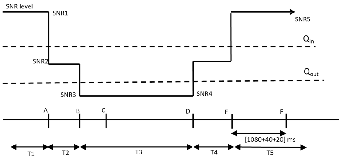
Figure A.14.4.3.8.1-1: SNR variation for in-sync testing in DRX
