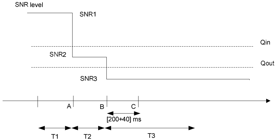
Figure A.7.3.14.1-1 SNR variation for out-of-sync testing
