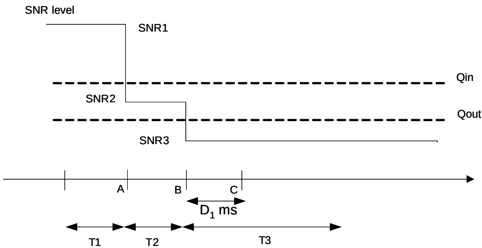
Figure A.14.4.3.7.1-1: SNR variation for out-of-sync testing in DRX
