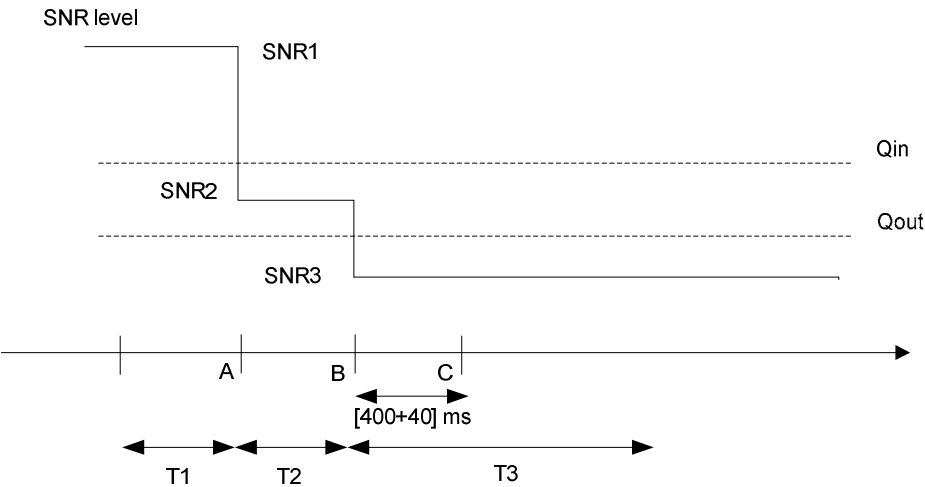
Figure A.14.4.3.1.1-1: SNR variation for out-of-sync testing
