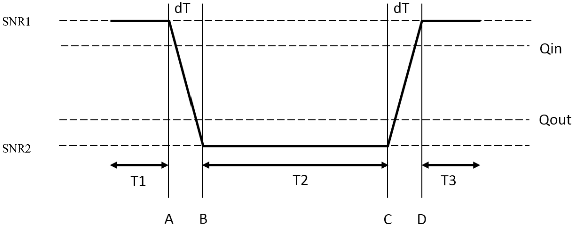
Figure A.13.4.3.5.1-1: SNR variation for in-sync testing without DRX
