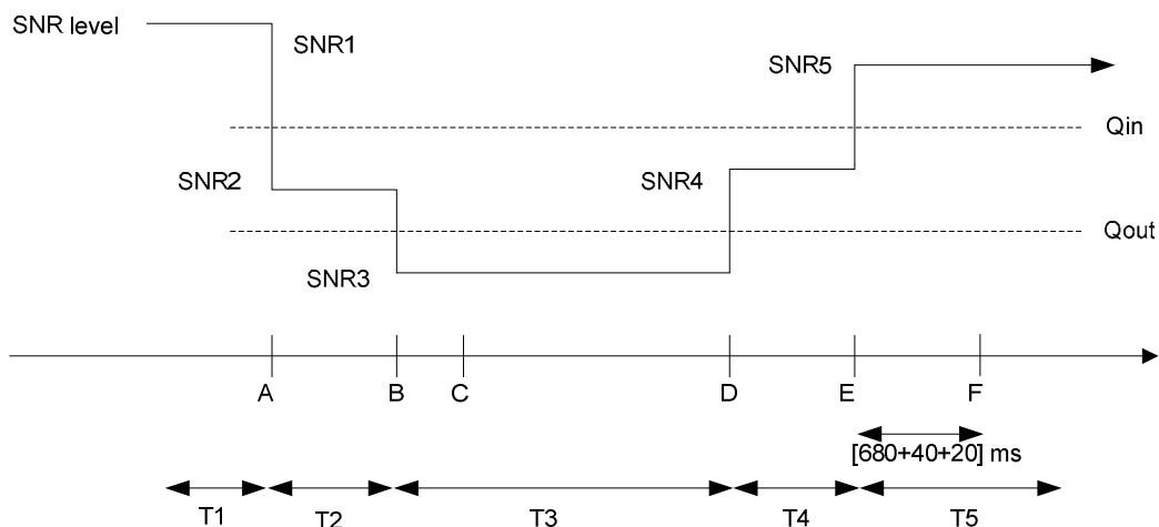
Figure A.14.4.3.4.1-1: SNR variation for in-sync testing
