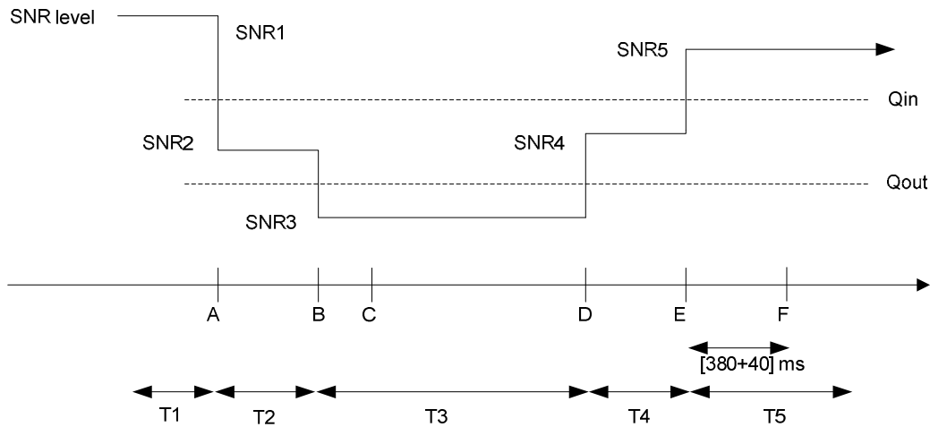
Figure A.7.3.27.1-1: SNR variation for in-sync testing
