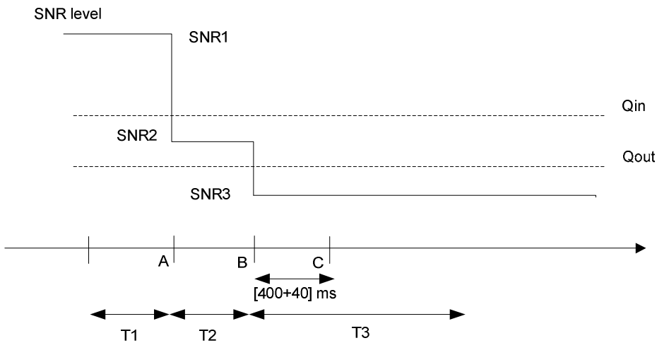
Figure A.7.3.78.1-1: SNR variation for out-of-sync testing
