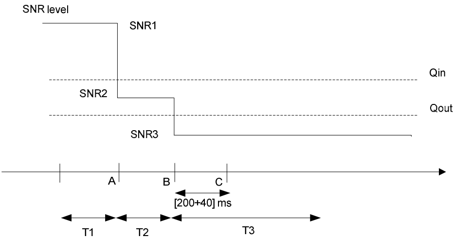
Figure A.7.3.34.1-1: SNR variation for out-of-sync testing
