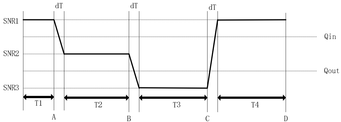
Figure A.13.4.3.2.1-1: SNR variation for HD-FDD Radio Link Monitoring Test for Out-of-sync in DRX for UE category NB1 Standalone mode in enhanced coverage
