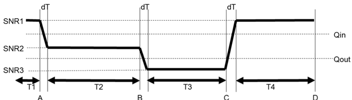
Figure A.13.4.3.8.1-1: SNR variation for out-of-sync testing
