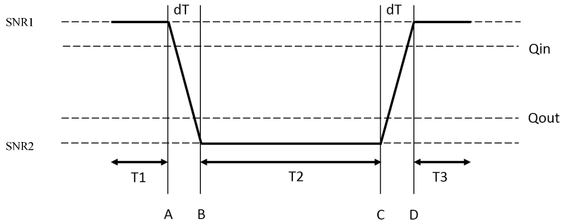
Figure A.13.4.3.3.1-1: SNR variation for in-sync testing with DRX
