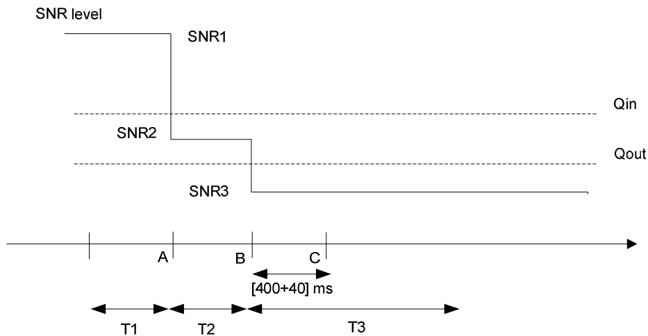
Figure A.7.3.56.1-1: SNR variation for out-of-sync testing
