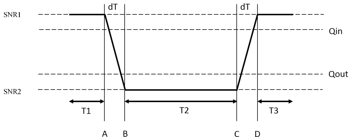
Figure A.13.4.3.6.1-1: SNR variation for in-sync testing without DRX
