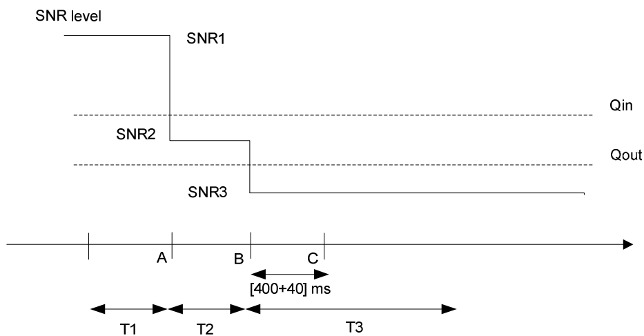
Figure A.7.3.74.1-1: SNR variation for out-of-sync testing
