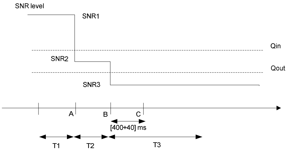
Figure A.7.3.98.1-1: SNR variation for out-of-sync testing
