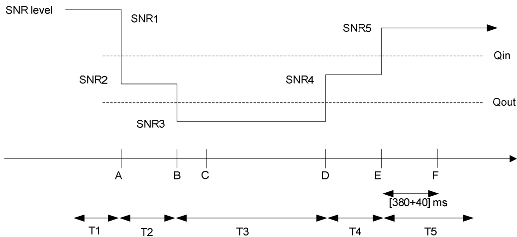
Figure A.7.3.20.1-1 SNR variation for in-sync testing
