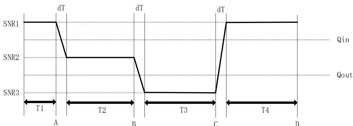
Figure A.13.4.3.1.1-1: SNR variation for out-of-sync testing in DRX for NB-IoT HD-FDD out-of-sync testing for UE category NB1 Standalone mode in normal coverage
