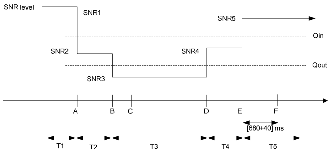
Figure A.14.4.3.2.1-1: SNR variation for in-sync testing
