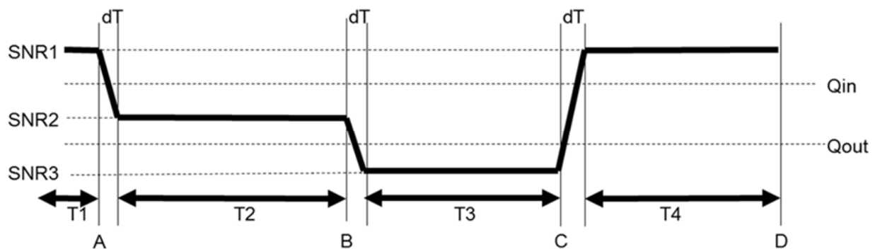
Figure A.13.4.3.7.1-1: SNR variation for out-of-sync testing
