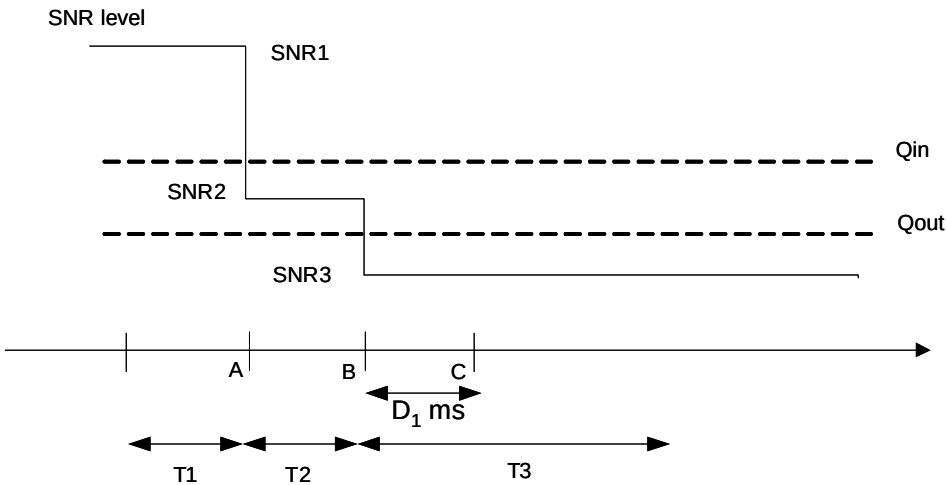
Figure A.14.4.3.5.1-1: SNR variation for out-of-sync testing in DRX
