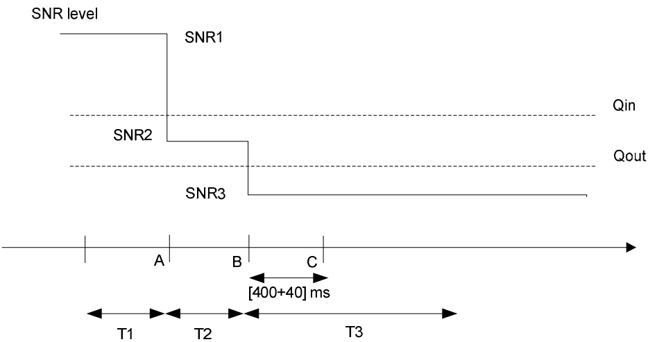
Figure A.7.3.48.1-1: SNR variation for out-of-sync testing
