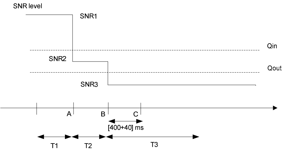
Figure A.14.4.3.3.1-1: SNR variation for out-of-sync testing
