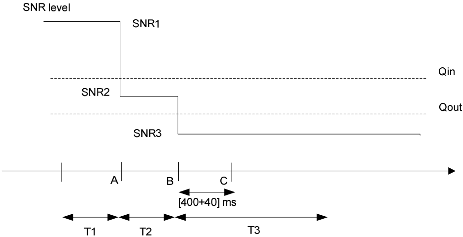
Figure A.7.3.74.1-1: SNR variation for out-of-sync testing
