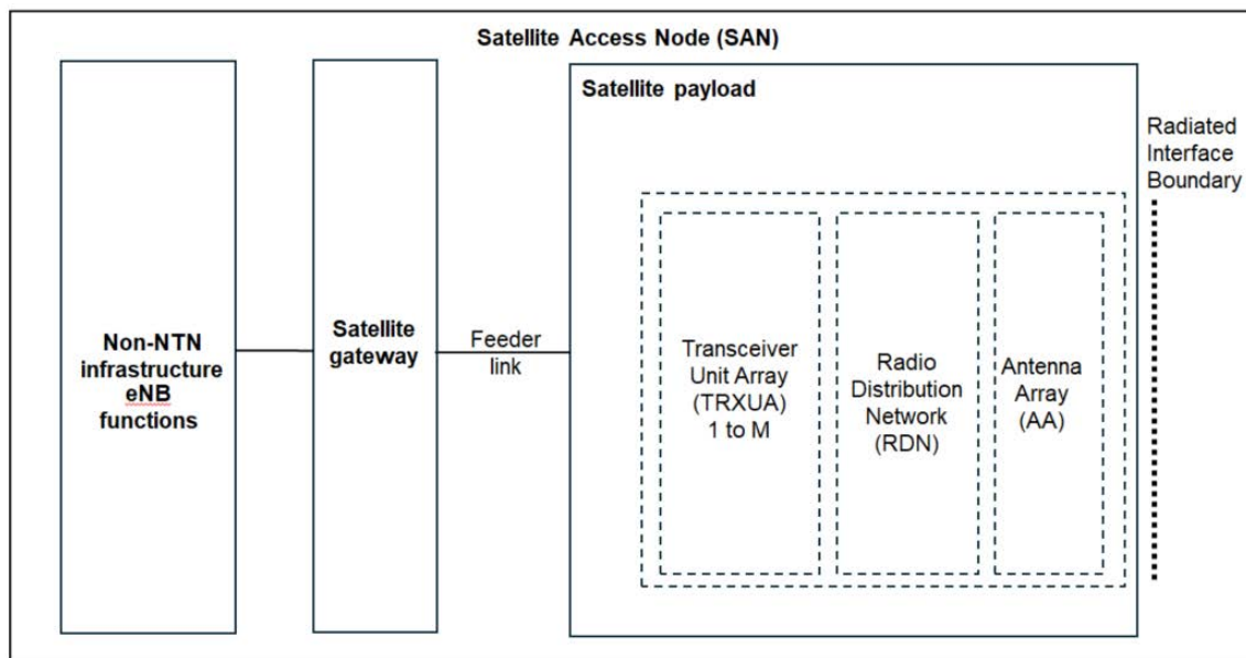
Figure 4.3.2-1: Radiated reference points for SAN type 1-O
