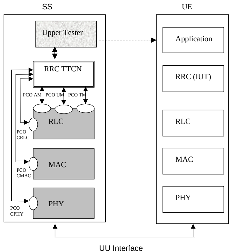
Figure 6.4.1: RRC testing architecture
