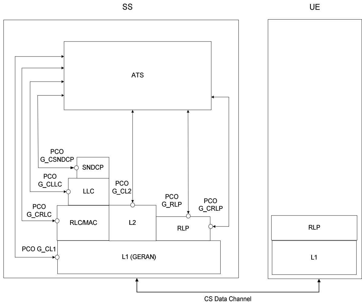
Figure 26: GERAN RLP codec model After the establishment of a CS non-transparent data call in a GERAN cell during the test, the UE may attempt to initiate a Radio Link Protocol (RLP) connection or start XID exchange before the RLP connection if the UE has an RLP installed. The RLP frame exchanges shall be handled by the SS, in order to carry on the test. Otherwise, the UE may disconnect the CS call.
