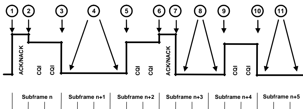
Figure 5.7A.2: Transmit power template below max power with TPC_cmd = 0
