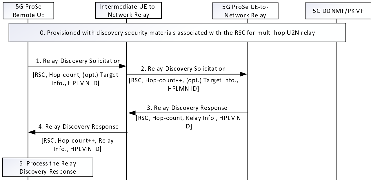
Figure 6.1.3.4.3.2-1: Model B Discovery operation supporting multi-hop UE-to-Network Relay
