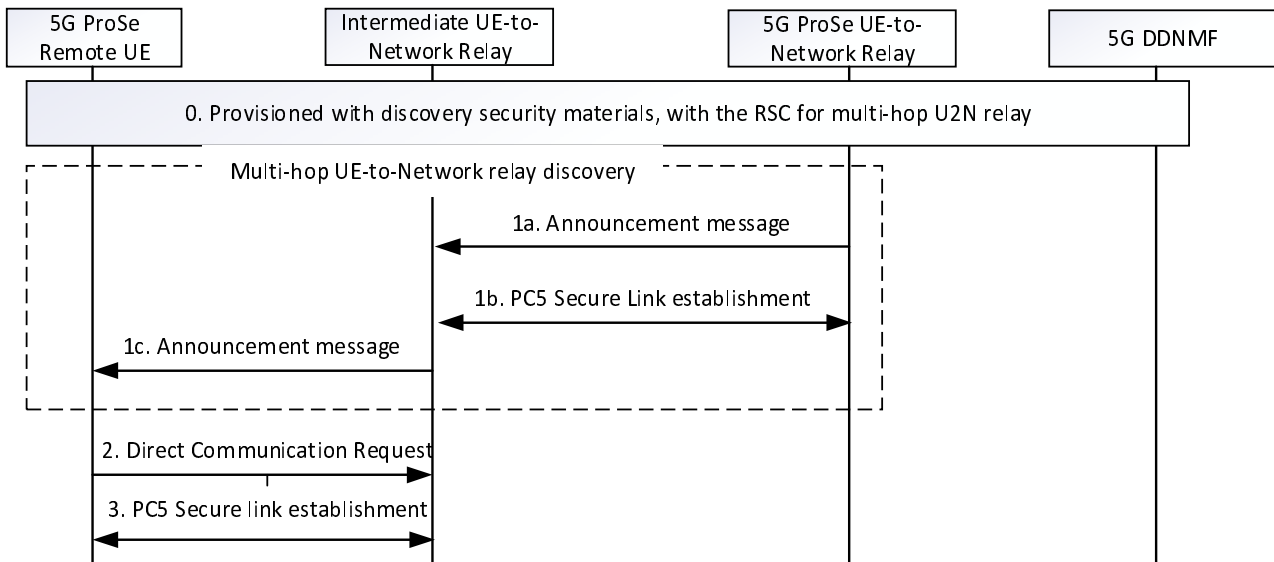
Figure 6.3.8.2.1-1: Security procedure over Control Plane for multi-hop UE-to-Network Relay communication when multi-hop UE-to-Network Relay discovery with Model A is used
