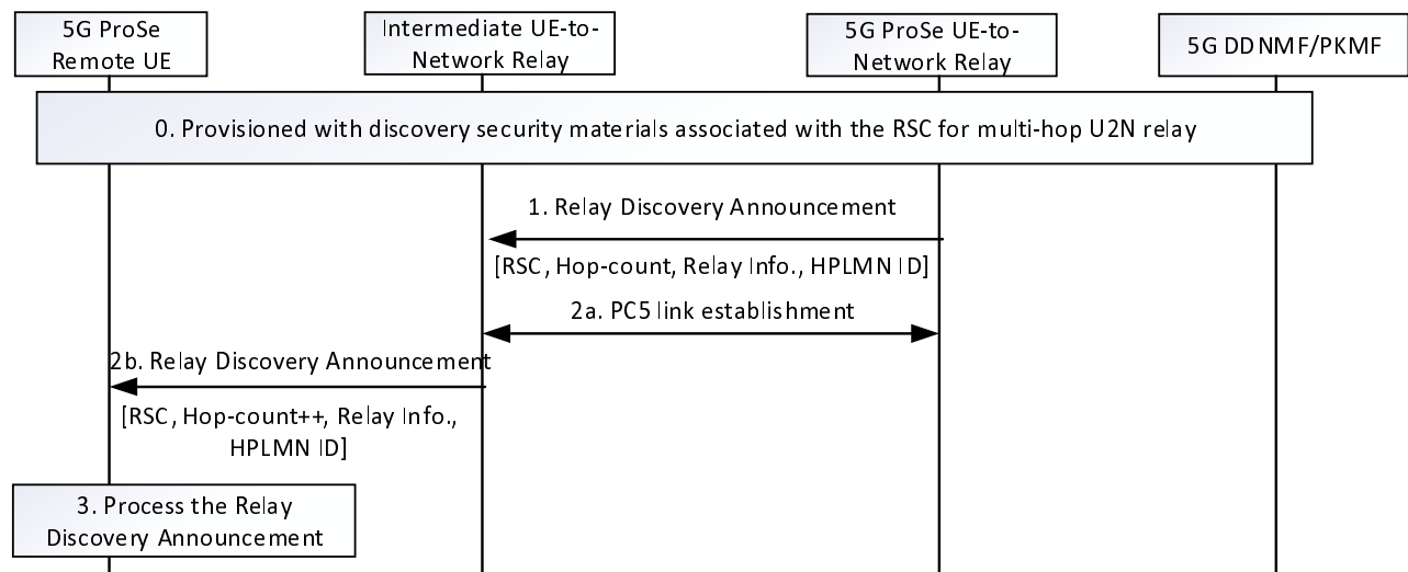
Figure 6.1.3.4.3.1-1: Model A Discovery operation supporting multi-hop UE-to-Network Relay
