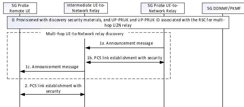
Figure 6.3.8.2.3-1: Security procedure over User Plane for multi-hop UE-to-Network Relay communication when multi-hop UE-to-Network Relay discovery with Model A is used
