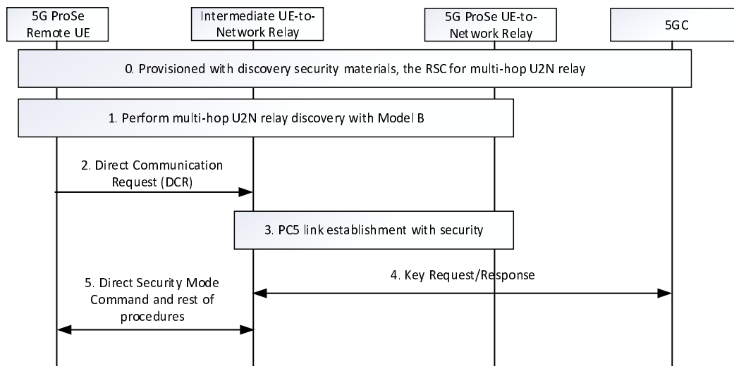
Figure 6.3.8.2.2-1: Security procedure over Control Plane for multi-hop UE-to-Network Relay communication when multi-hop UE-to-Network Relay discovery with Model B is used
