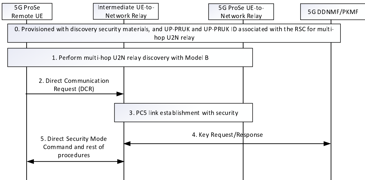
Figure 6.3.8.2.4-1: Security procedure over User Plane for multi-hop UE-to-Network Relay communication when multi-hop UE-to-Network Relay discovery with Model B is used
