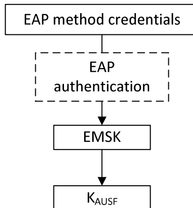
Figure I.2.3-1: K_{\text{AUSF}} derivation for key-generating EAP authentication methods other than EAP-AKA'
