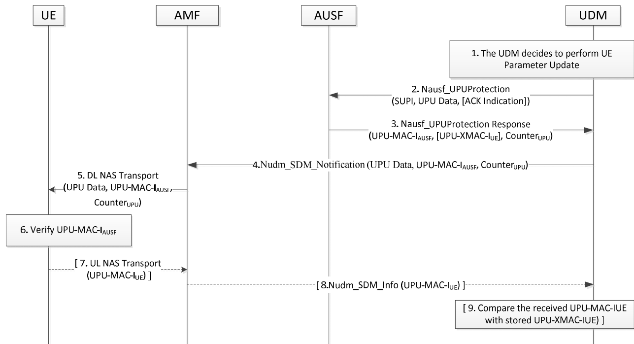
Figure 6.15.2.1-1: Procedure for UE Parameters Update
