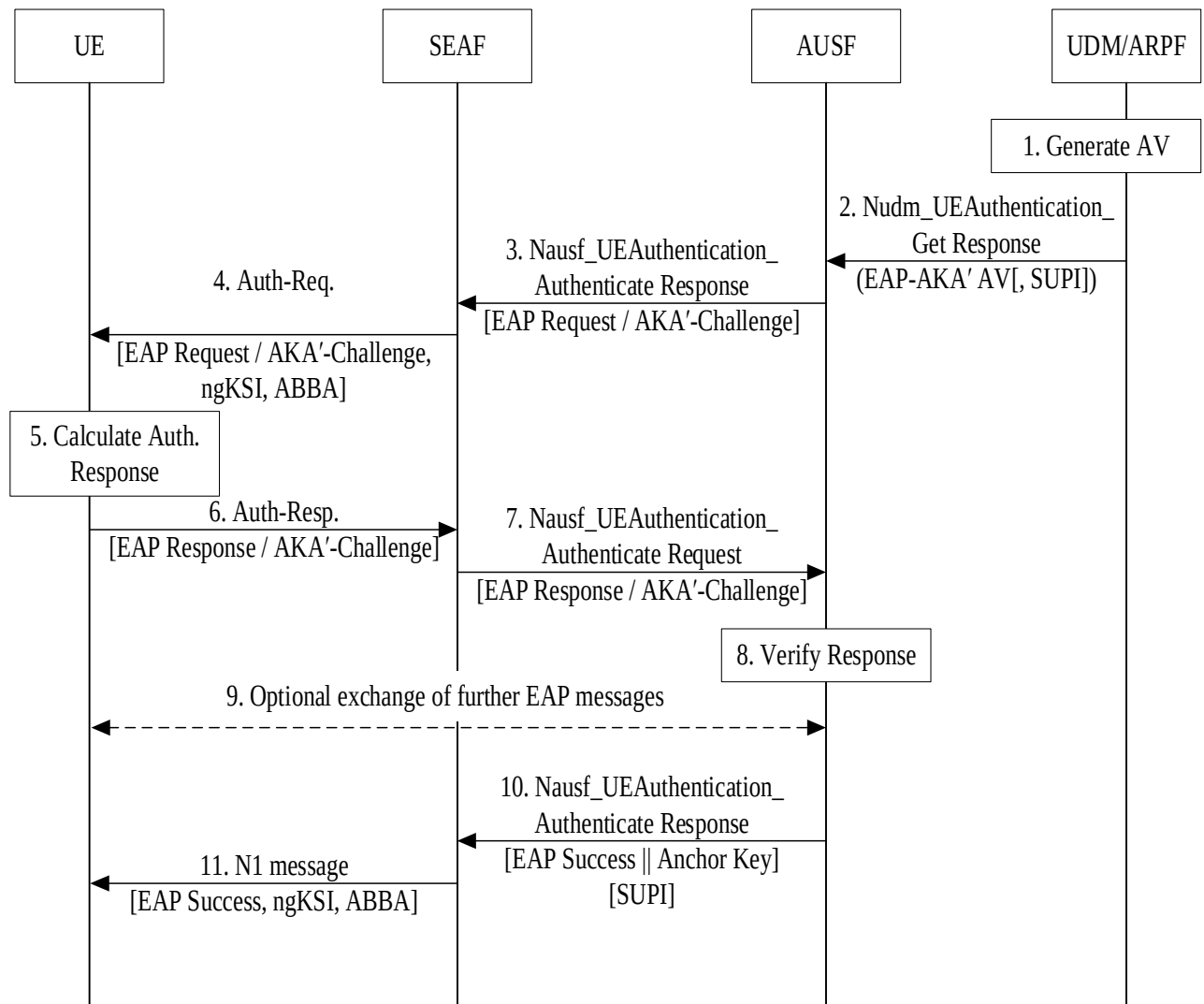
Figure 6.1.3.1-1: Authentication procedure for EAP-AKA'
