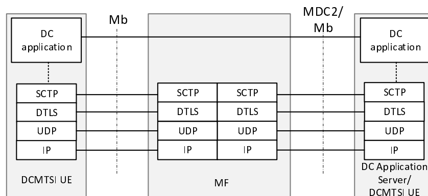
Figure N.3.1-4: Protocol stack for MF in the DC application proxy configuration mode (TS 23.228 [3])
