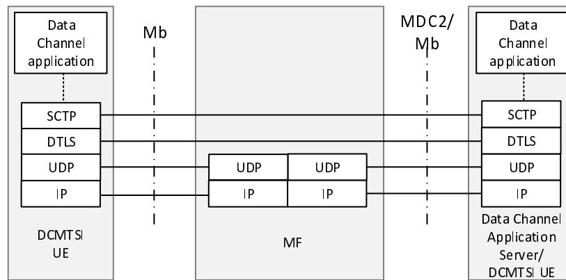
Figure N.3.1-3: Protocol stack for MF in the UDP proxy configuration mode (P2P/P2A/A2P IMS application data channels) (TS 23.228 [3])
