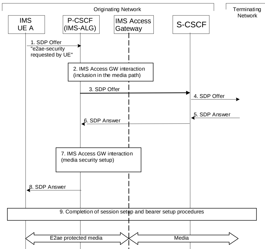
Figure 7.2.1-1: Originating call flow for e2ae case
