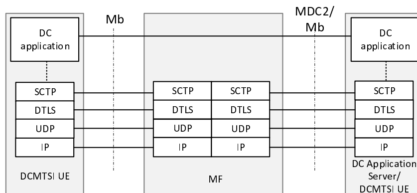
Figure N.3.1-4: Protocol stack for MF in the DC application proxy configuration mode (TS 23.228 [3])
