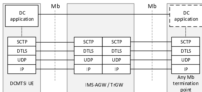
Figure N.3.1-5: Protocol stack for IMS-AGW / TrGW in the DC application proxy configuration mode (TS 23.228 [3])
