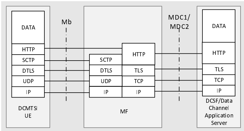
Figure N.3.1-2: Protocol stack for MF in the HTTP proxy configuration mode (IMS bootstrap data channel or IMS application data channel) (TS 23.228 [3])
